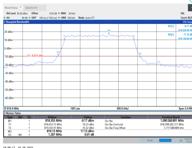
Band26-1.4MHz-QPSK-26740-6RB#0
