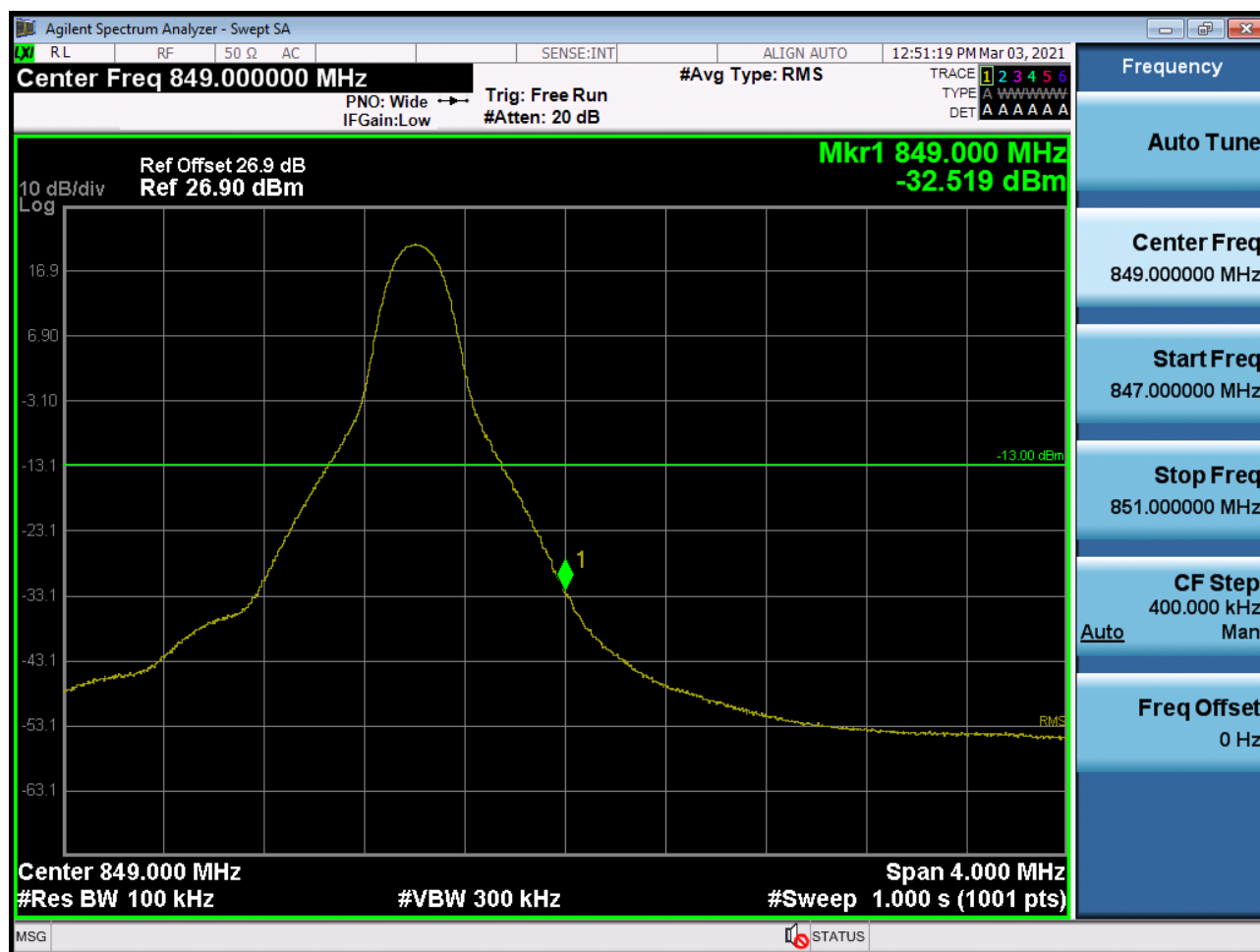
BAND 5. Upper Band Edge Plot (10M BW Ch.20600 QPSK RB1 Offset 49)
