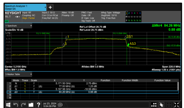
Figure 333 - 802.11ax HE80 SU Maximum 99% OBW
