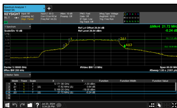
Figure 321 - 802.11n HT20 Maximum 99% OBW
