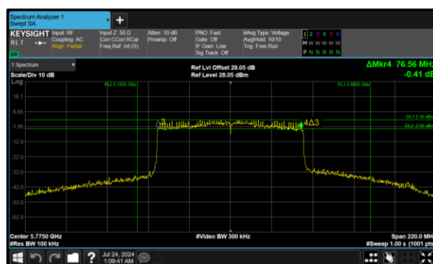
Figure 319 - 802.11ax HE80 SU Maximum 6 dB EBW
