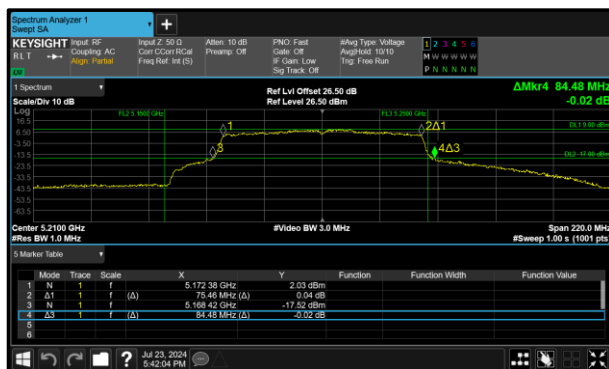
Figure 324 - 802.11ac VHT80 Minimum 99% OBW
