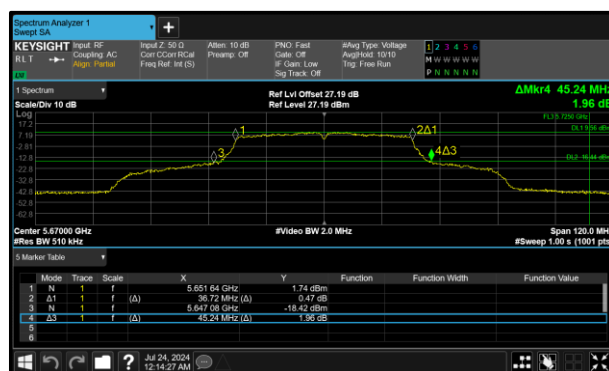
Figure 323 - 802.11n HT40 Maximum 99% OBW
