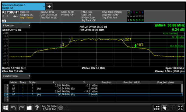
Figure 339 - 802.11ac VHT40 Maximum 99% OBW
