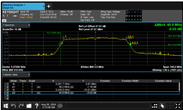
Figure 338 - 802.11ac VHT40 Minimum 99% OBW
