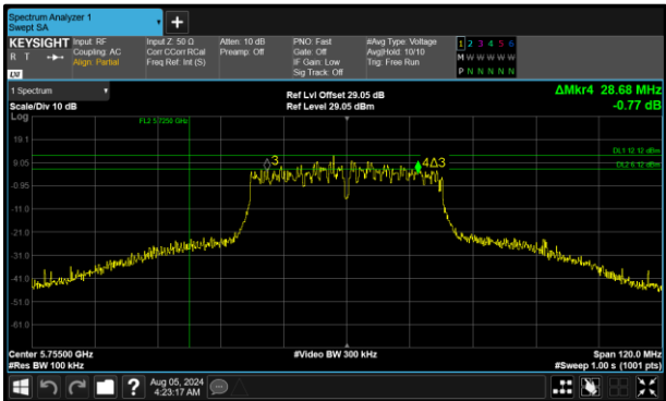
Figure 344 - 802.11ac VHT40 Minimum 6 dB EBW
