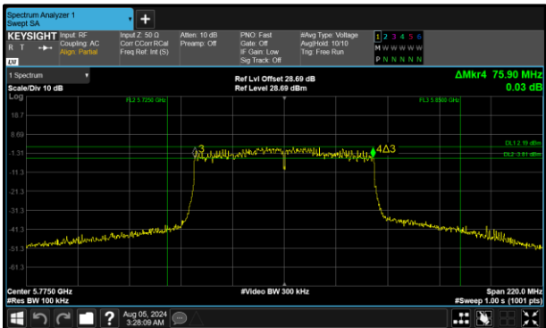
Figure 346 - 802.11ac VHT80 Minimum 6 dB EBW
