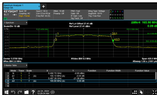
Figure 327 - 802.11ac VHT160 Maximum 99% OBW
