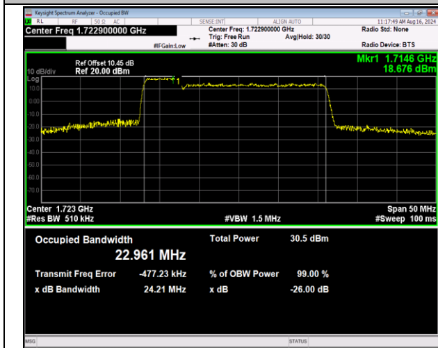
66-66-5MHz-20MHz-64QAM-64QAM-132005-132122-25R B#0-100RB#0-PASS
