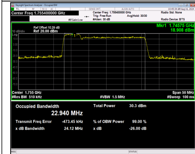
66-66-5MHz-20MHz-16QAM-16QAM-132330-132447-25R B#0-100RB#0-PASS
