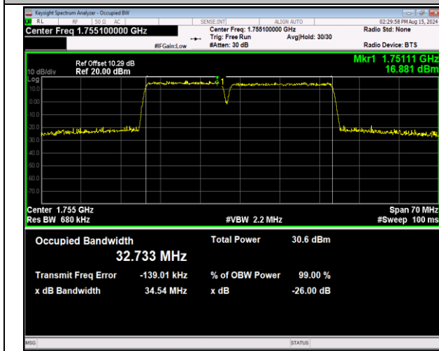
66-66-15MHz-20MHz-64QAM-64QAM-132325-132496-75RB #0-100RB#0-PASS
