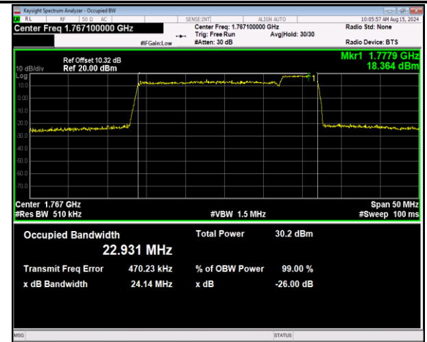
66-66-20MHz-5MHz-16QAM-16QAM-132522-132639-100RB #0-25RB#0-PASS
