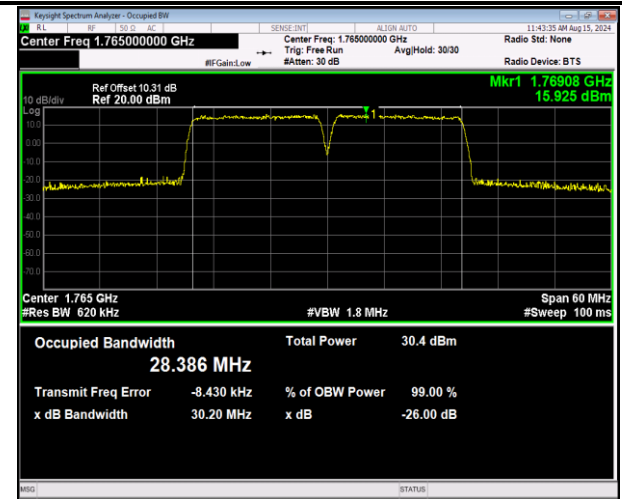
66-66-15MHz-15MHz-16QAM-16QAM-132447-132597-75RB #0-75RB#0-PASS
