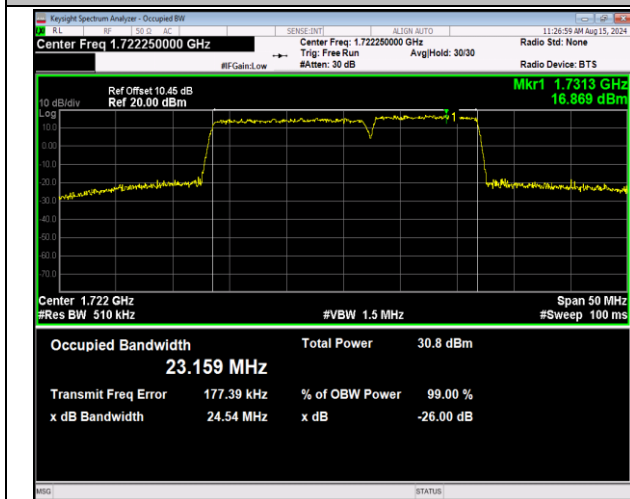
66-66-15MHz-10MHz-16QAM-16QAM-132047-132167-75RB #0-50RB#0-PASS
