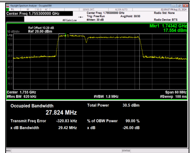
66-66-10MHz-20MHz-64QAM-64QAM-132328-132472-50RB #0-100RB#0-PASS
