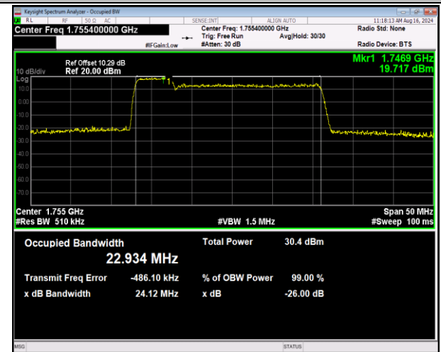
66-66-5MHz-20MHz-64QAM-64QAM-132330-132447-25R B#0-100RB#0-PASS
