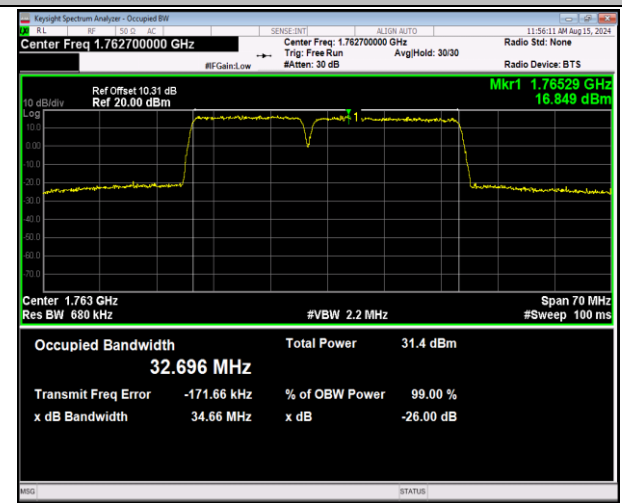
66-66-15MHz-20MHz-QPSK-QPSK-132401-132572-75RB #0-100RB#0-PASS
