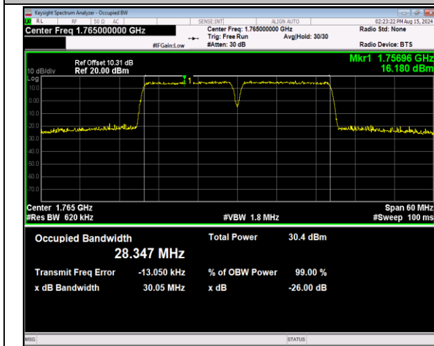
66-66-15MHz-15MHz-64QAM-64QAM-132447-132597-75RB #0-75RB#0-PASS
