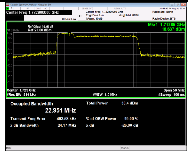
66-66-5MHz-20MHz-16QAM-16QAM-132005-132122-25R B#0-100RB#0-PASS
