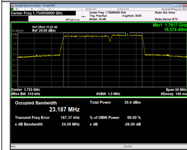
66-66-15MHz-10MHz-64QAM-64QAM-132373-132493-75RB #0-50RB#0-PASS
