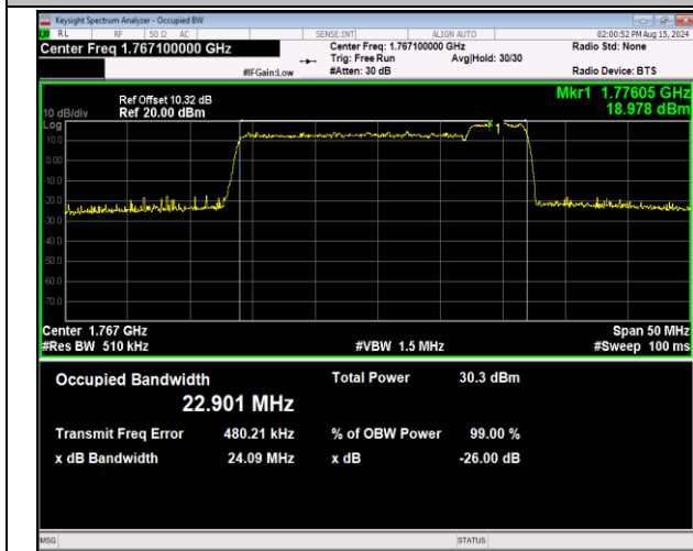
66-66-20MHz-5MHz-64QAM-64QAM-132522-132639-100RB #0-25RB#0-PASS
