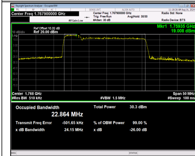
66-66-5MHz-20MHz-64QAM-64QAM-132455-132572-25R B#0-100RB#0-PASS
