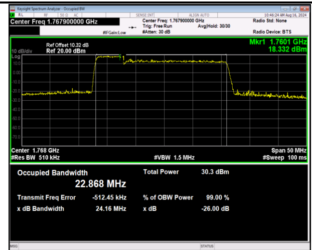
66-66-5MHz-20MHz-16QAM-16QAM-132455-132572-25R B#0-100RB#0-PASS
