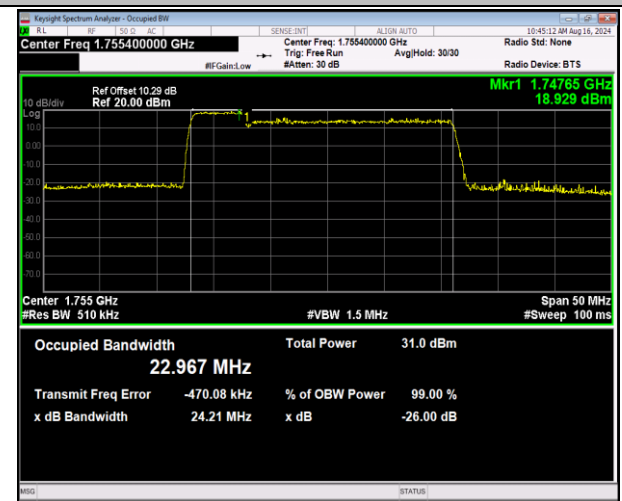
66-66-5MHz-20MHz-QPSK-QPSK-132330-132447-25RB# 0-100RB#0-PASS
