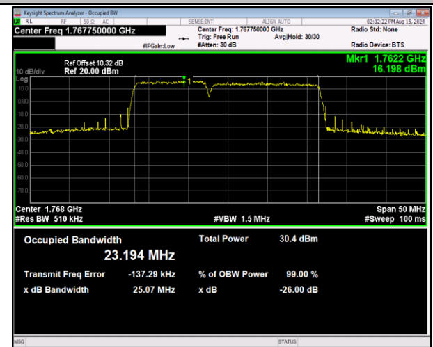
66-66-10MHz-15MHz-64QAM-64QAM-132477-132597-50RB #0-75RB#0-PASS
