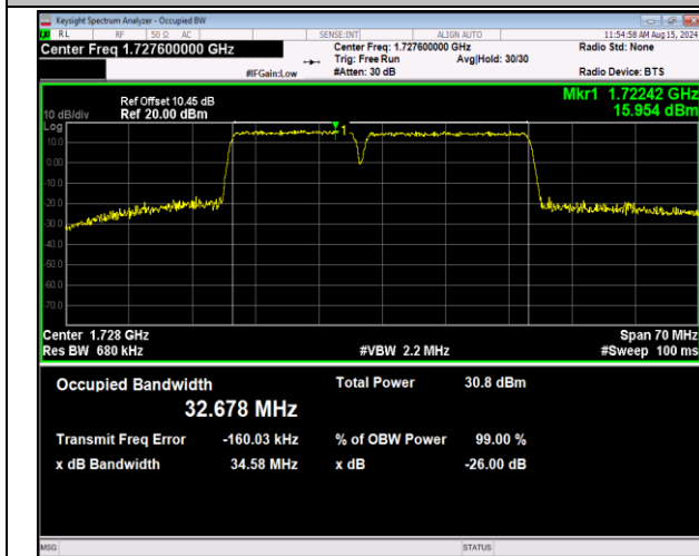
66-66-15MHz-20MHz-16QAM-16QAM-132050-132221-75RB #0-100RB#0-PASS
