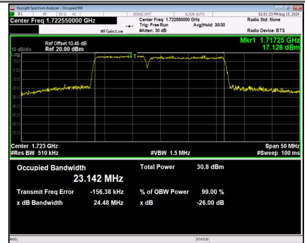
66-66-10MHz-15MHz-64QAM-64QAM-132025-132145-50 RB#0-75RB#0-PASS
