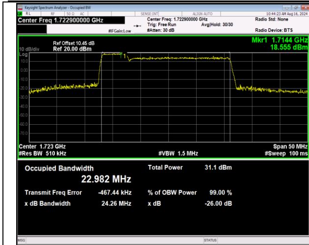
66-66-5MHz-20MHz-QPSK-QPSK-132005-132122-25RB# 0-100RB#0-PASS
