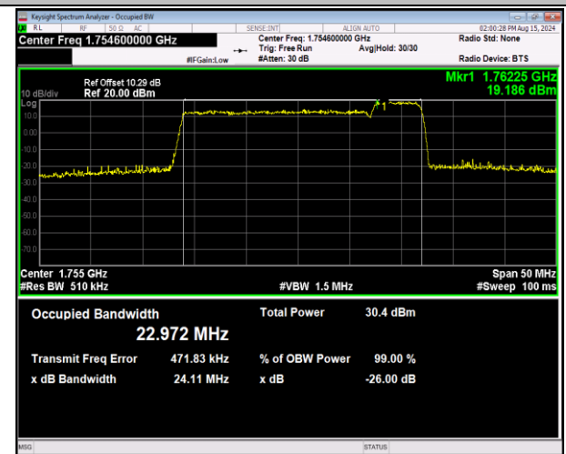
66-66-20MHz-5MHz-64QAM-64QAM-132397-132514-100RB #0-25RB#0-PASS
