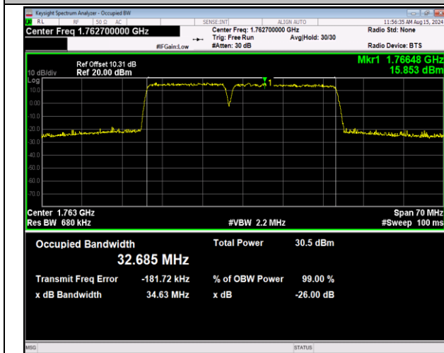
66-66-15MHz-20MHz-16QAM-16QAM-132401-132572-75RB #0-100RB#0-PASS
