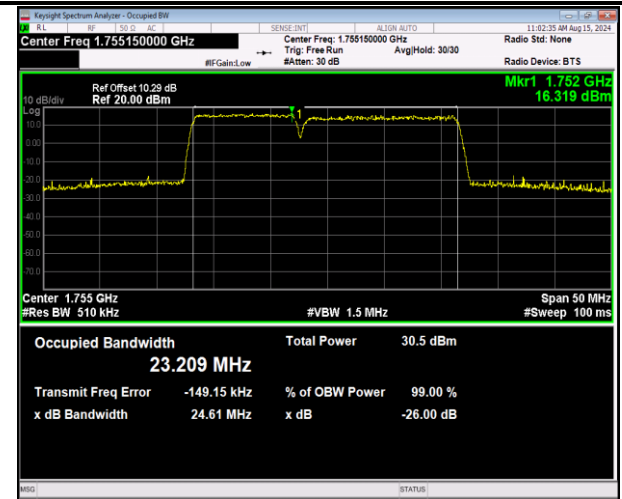
66-66-10MHz-15MHz-16QAM-16QAM-132351-132471-50RB #0-75RB#0-PASS
