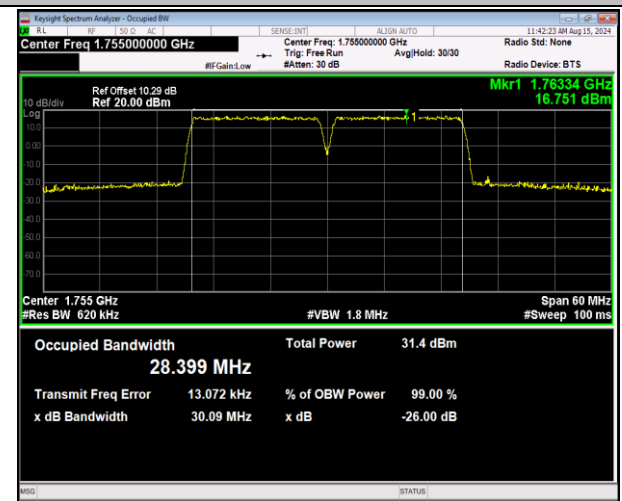
66-66-15MHz-15MHz-QPSK-QPSK-132347-132497-75RB #0-75RB#0-PASS
