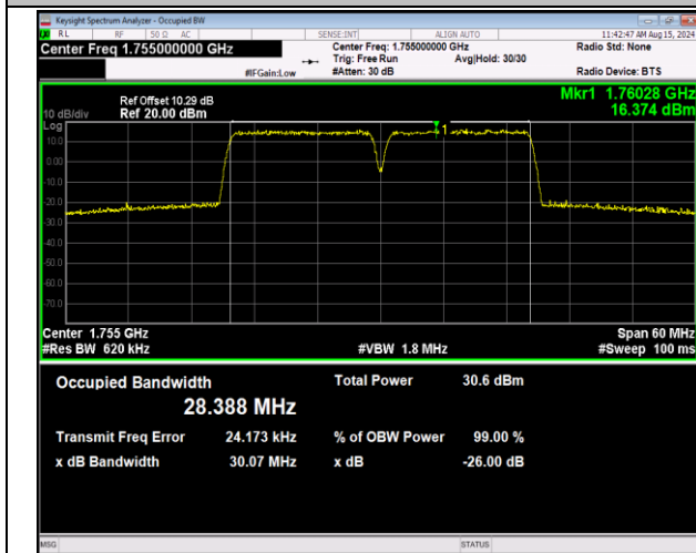
66-66-15MHz-15MHz-16QAM-16QAM-132347-132497-75RB #0-75RB#0-PASS
