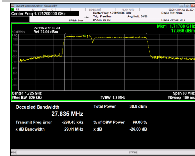
66-66-10MHz-20MHz-64QAM-64QAM-132027-132171-50RB #0-100RB#0-PASS
