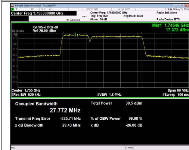
66-66-10MHz-20MHz-16QAM-16QAM-132328-132472-50RB #0-100RB#0-PASS
