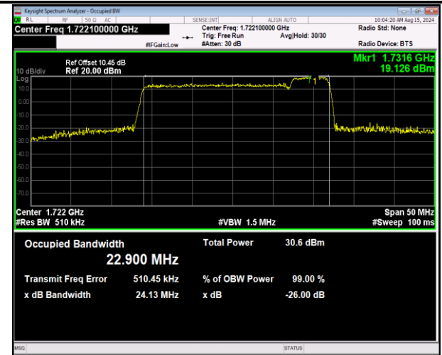
66-66-20MHz-5MHz-16QAM-16QAM-132072-132189-100RB #0-25RB#0-PASS
