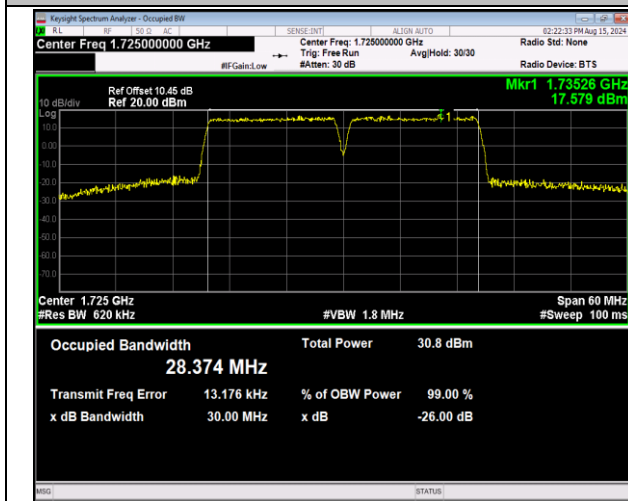
66-66-15MHz-15MHz-64QAM-64QAM-132047-132197-75RB #0-75RB#0-PASS
