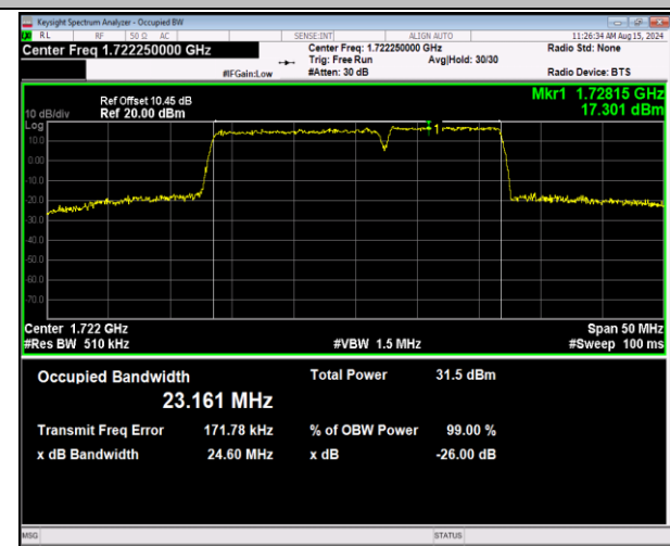
66-66-15MHz-10MHz-QPSK-QPSK-132047-132167-75RB #0-50RB#0-PASS
