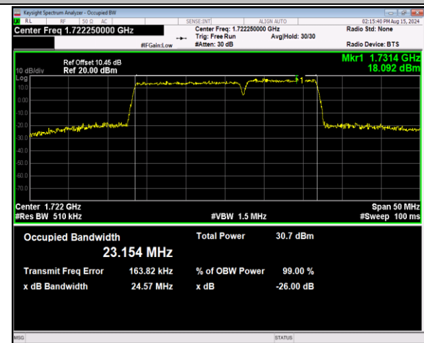
66-66-15MHz-10MHz-64QAM-64QAM-132047-132167-75RB #0-50RB#0-PASS
