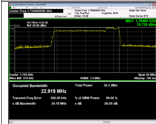
66-66-20MHz-5MHz-16QAM-16QAM-132397-132514-100RB #0-25RB#0-PASS
