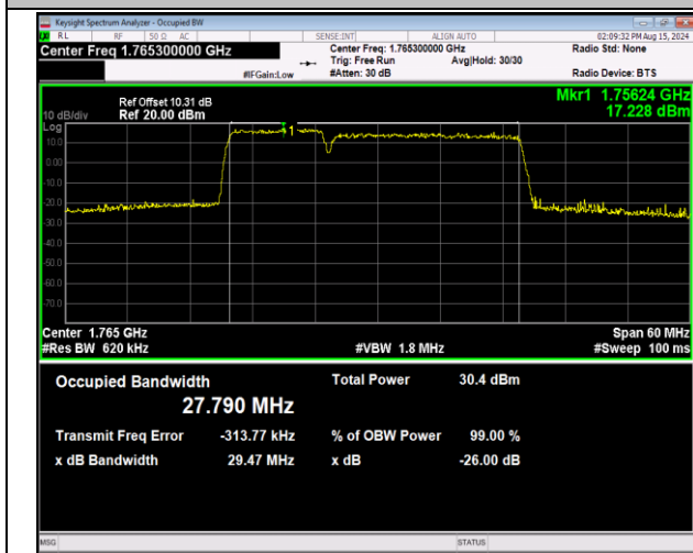
66-66-10MHz-20MHz-64QAM-64QAM-132428-132572-50RB #0-100RB#0-PASS
