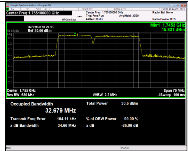
66-66-15MHz-20MHz-16QAM-16QAM-132325-132496-75RB #0-100RB#0-PASS
