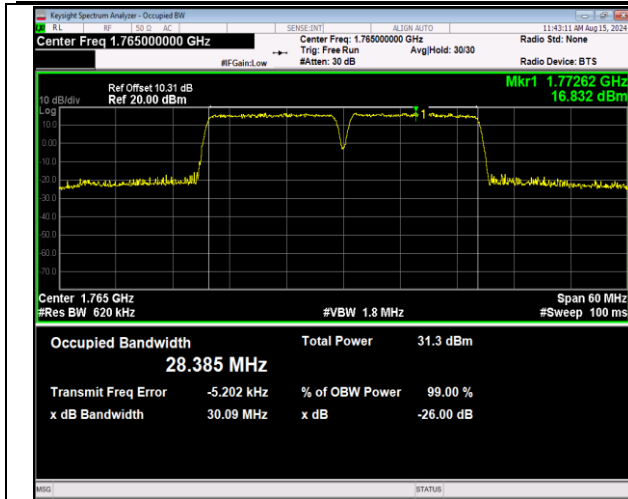
66-66-15MHz-15MHz-QPSK-QPSK-132447-132597-75RB #0-75RB#0-PASS
