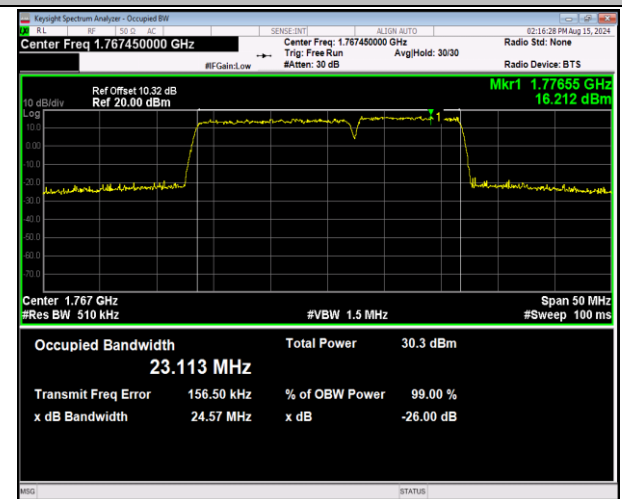
66-66-15MHz-10MHz-64QAM-64QAM-132499-132619-75RB #0-50RB#0-PASS
