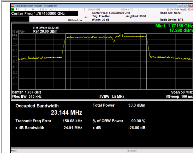
66-66-15MHz-10MHz-16QAM-16QAM-132499-132619-75RB #0-50RB#0-PASS
