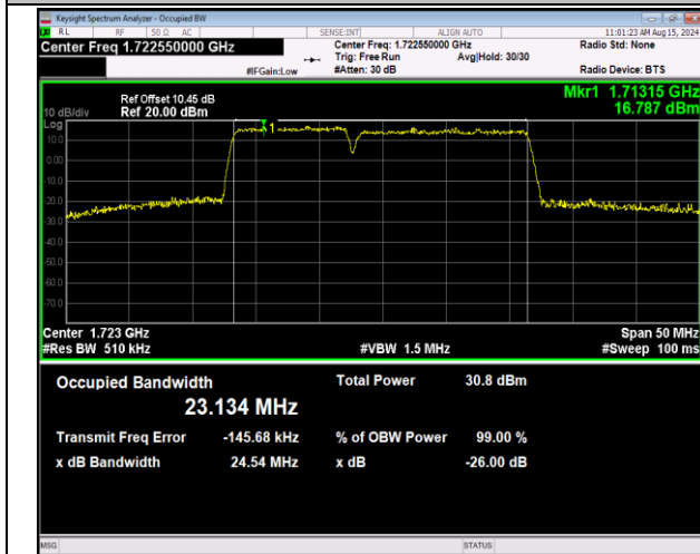
66-66-10MHz-15MHz-16QAM-16QAM-132025-132145-50 RB#0-75RB#0-PASS
