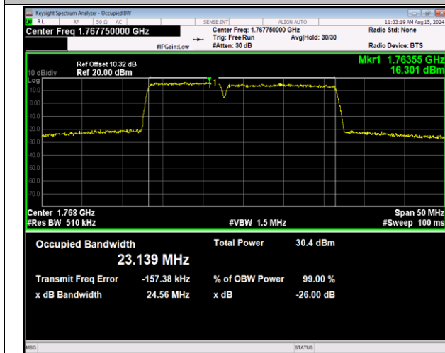
66-66-10MHz-15MHz-16QAM-16QAM-132477-132597-50RB #0-75RB#0-PASS
