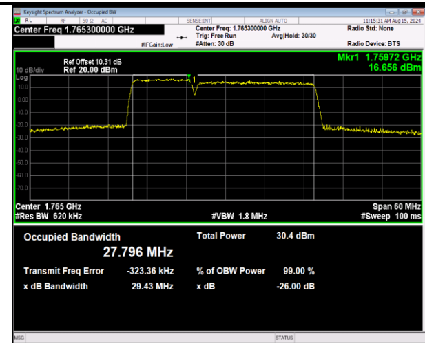
66-66-10MHz-20MHz-16QAM-16QAM-132428-132572-50RB #0-100RB#0-PASS
