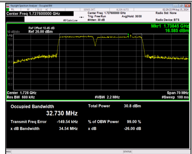
66-66-15MHz-20MHz-64QAM-64QAM-132050-132221-75RB #0-100RB#0-PASS
