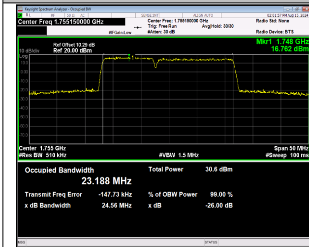
66-66-10MHz-15MHz-64QAM-64QAM-132351-132471-50RB #0-75RB#0-PASS
