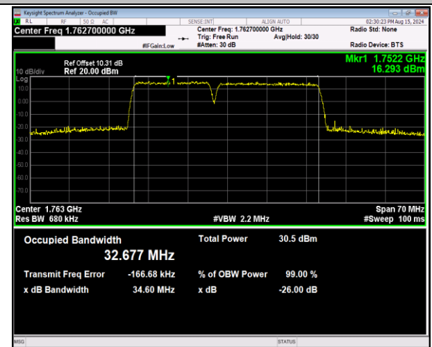
66-66-15MHz-20MHz-64QAM-64QAM-132401-132572-75RB #0-100RB#0-PASS
