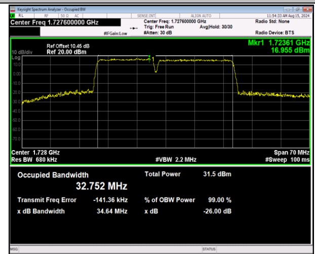
66-66-15MHz-20MHz-QPSK-QPSK-132050-132221-75RB #0-100RB#0-PASS
