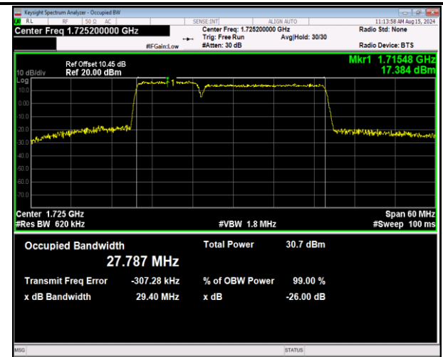
66-66-10MHz-20MHz-16QAM-16QAM-132027-132171-50RB #0-100RB#0-PASS
