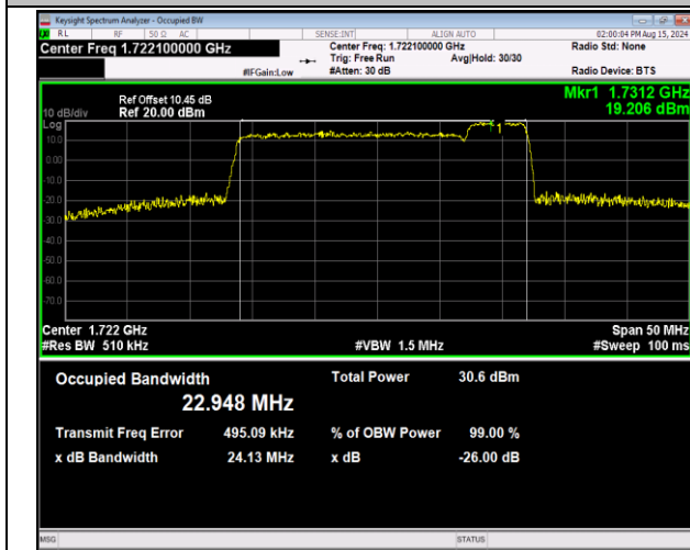
66-66-20MHz-5MHz-64QAM-64QAM-132072-132189-100RB #0-25RB#0-PASS
