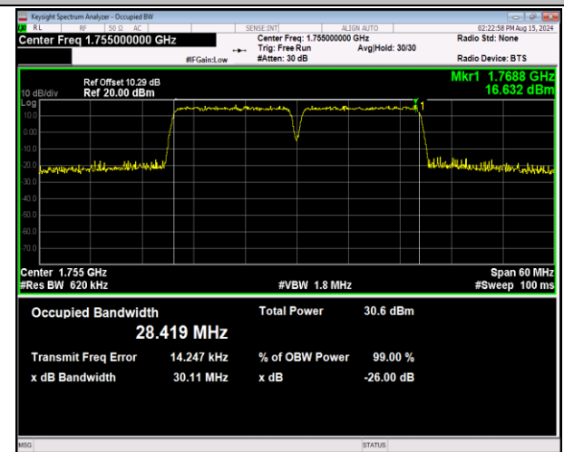
66-66-15MHz-15MHz-64QAM-64QAM-132347-132497-75RB #0-75RB#0-PASS
