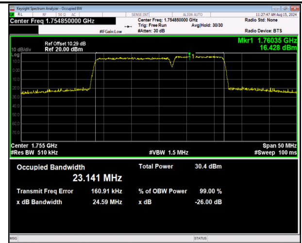
66-66-15MHz-10MHz-16QAM-16QAM-132373-132493-75RB #0-50RB#0-PASS
