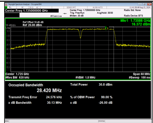
66-66-15MHz-15MHz-16QAM-16QAM-132047-132197-75RB #0-75RB#0-PASS
