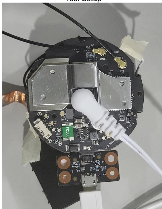
Test Setup
