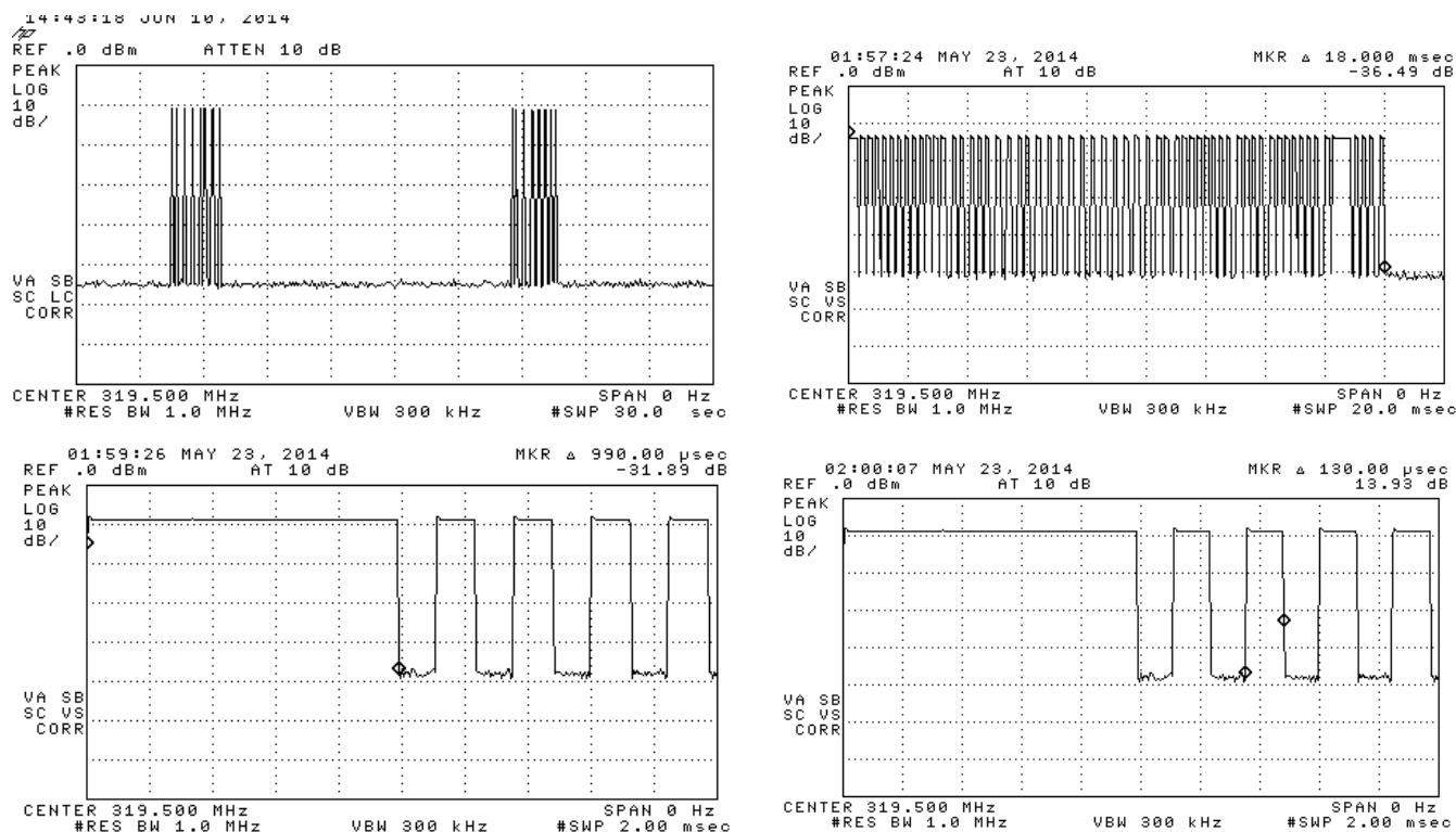
Figure 5: Pulsed Emission Characteristics (Duty Cycle).
