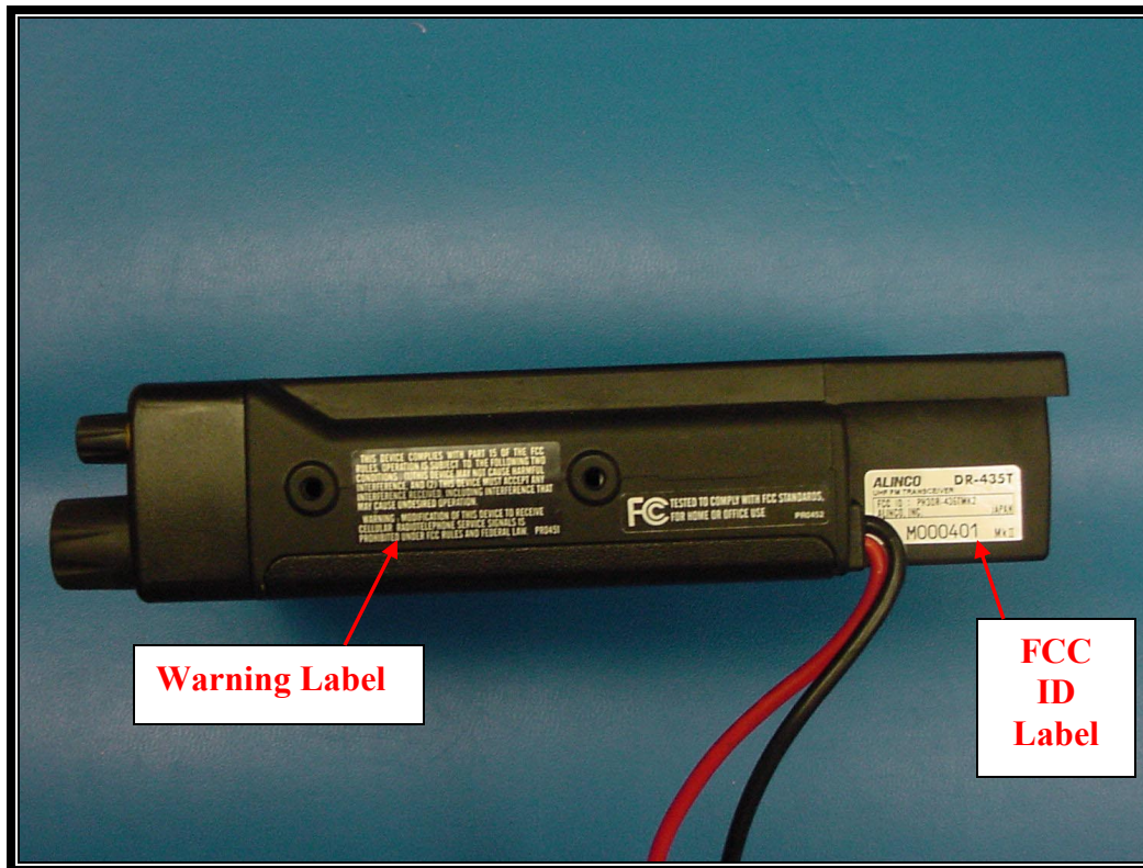
PHOTOGRAPH 3: FCC ID LABEL AND WARNING LABEL LOCATIONS ON RIGHT SIDE OF EUT
