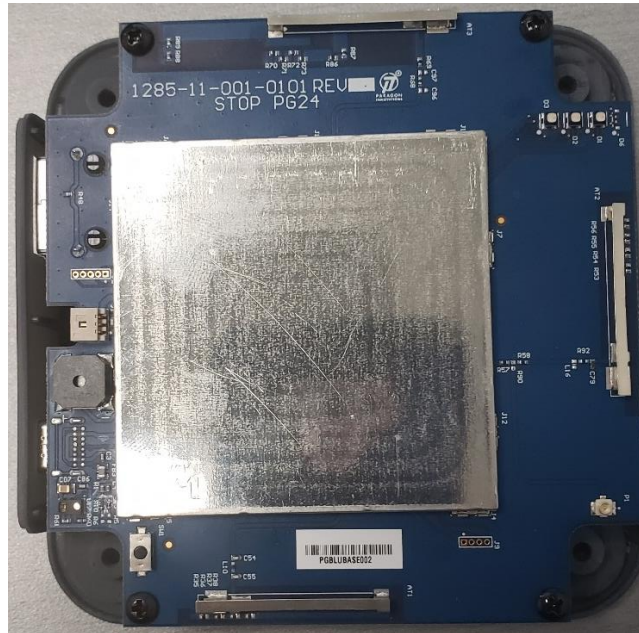
Top of BLUbase PCB with Shield Installed
