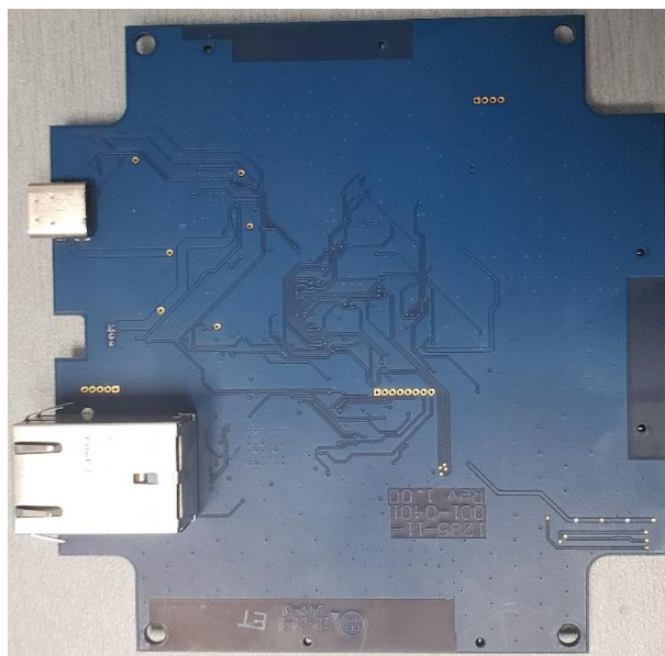
Bottom of BLUbase PCB
