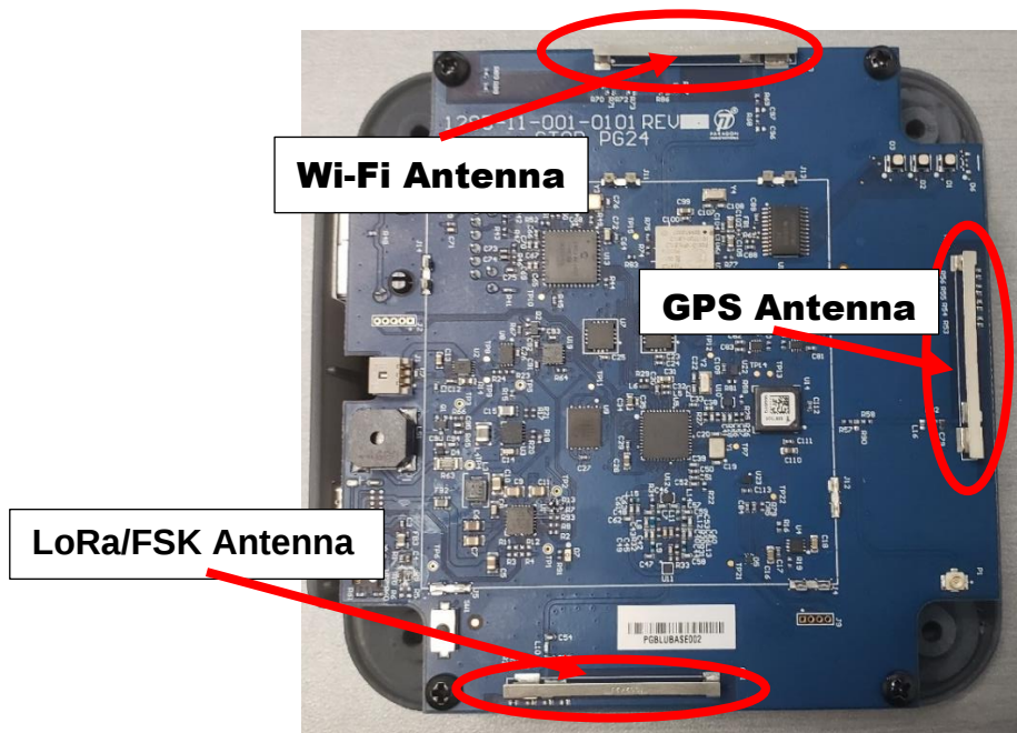
BLUbase Showing Antenna Location
