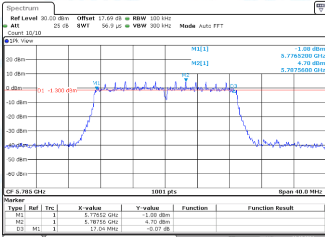
11AC20MIMO-Ant1-5785-PASS
