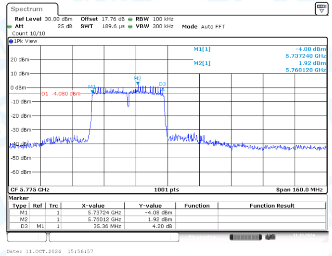
11AX80MIMO-Ant2-5775-PASS
