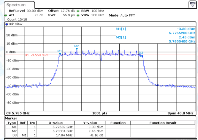
11AC20MIMO-Ant2-5785-PASS
