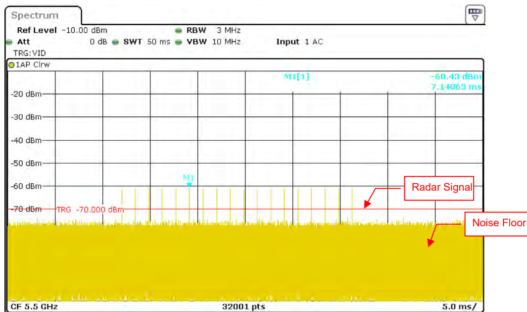
Radar Signal 0
