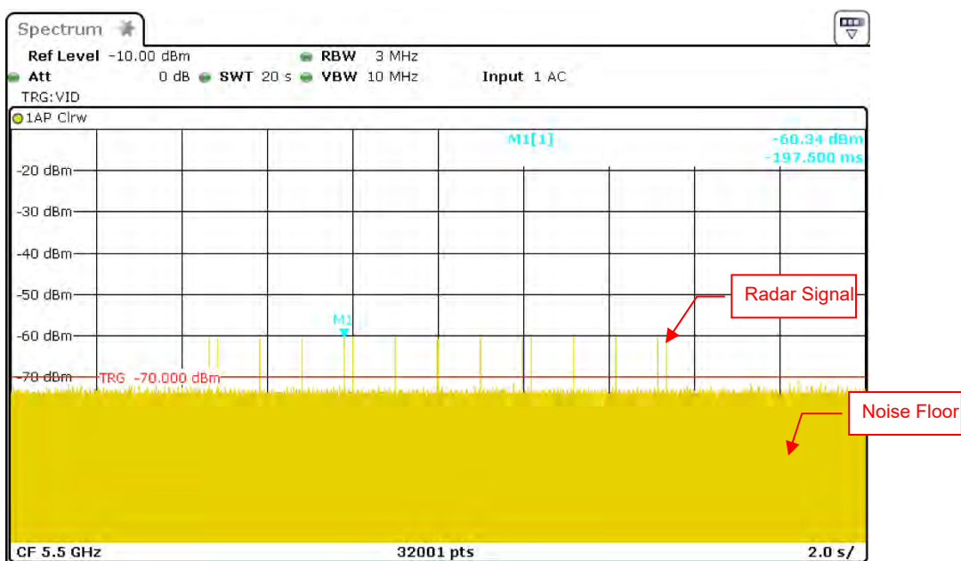
Radar Signal 5
