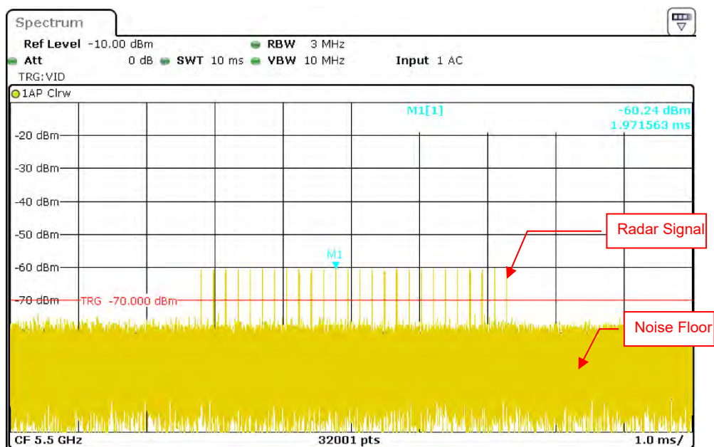
Radar Signal 2
