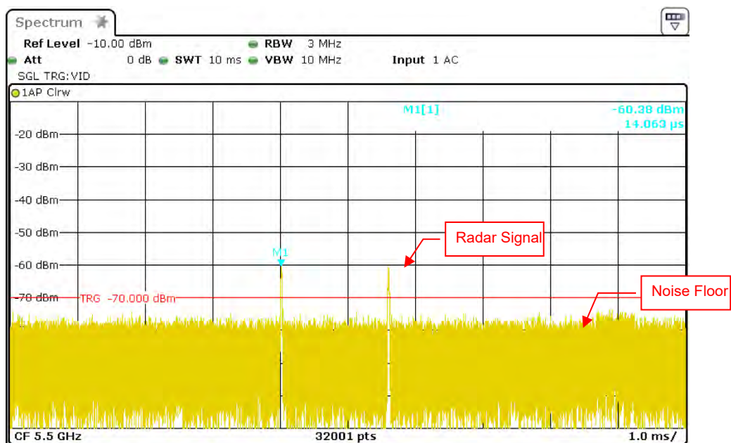
Single Burst of Radar Signal 5
