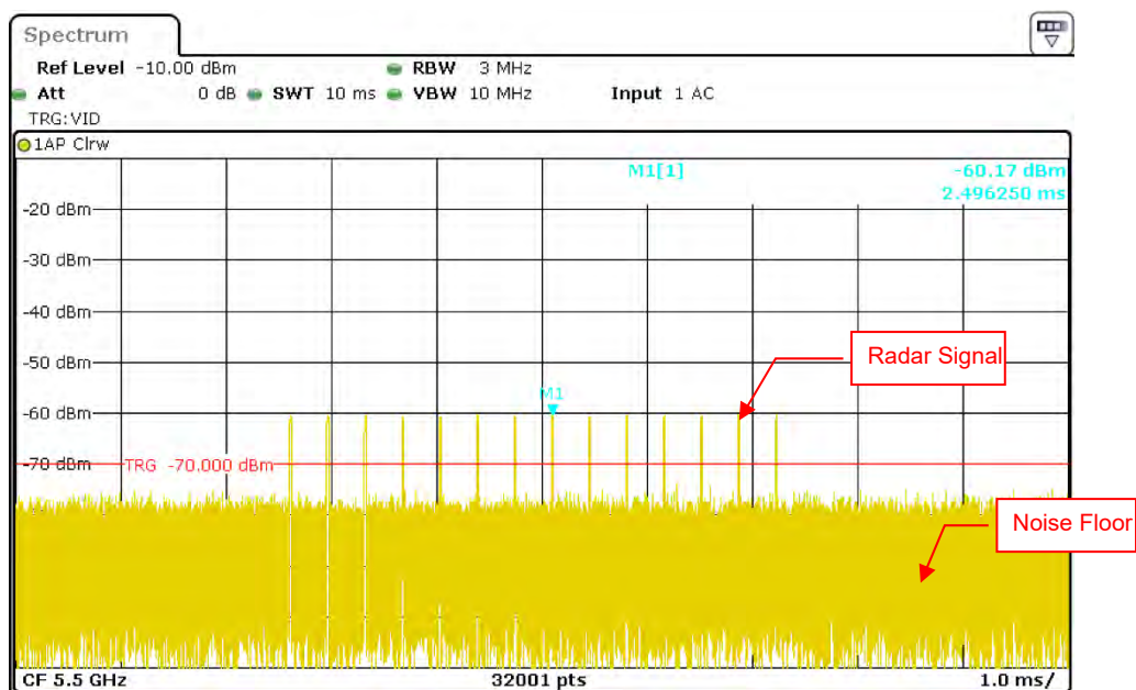
Radar Signal 4
