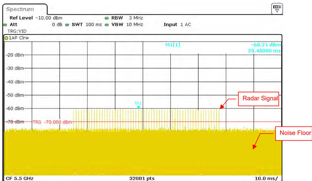
Radar Signal 1 (Test A)
