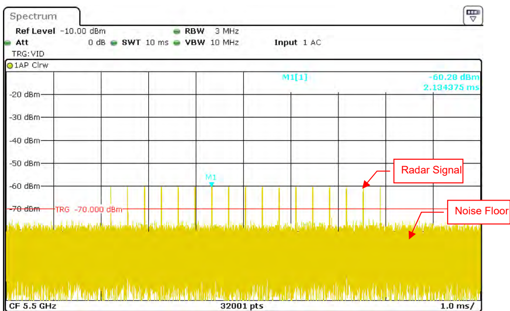
Radar Signal 3
