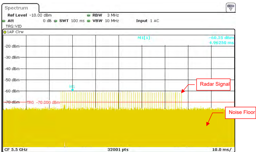
Radar Signal 1 (Test B)
