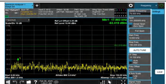
Band26(824-849)-1.4MHz-QPSK-26915-1RB#5-0.009~0.15-PASS S
