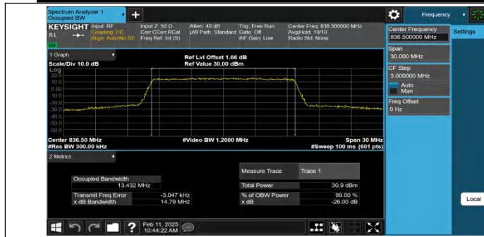
Band26(824-849)-15MHz-QPSK-26915-75RB#0-PASS
