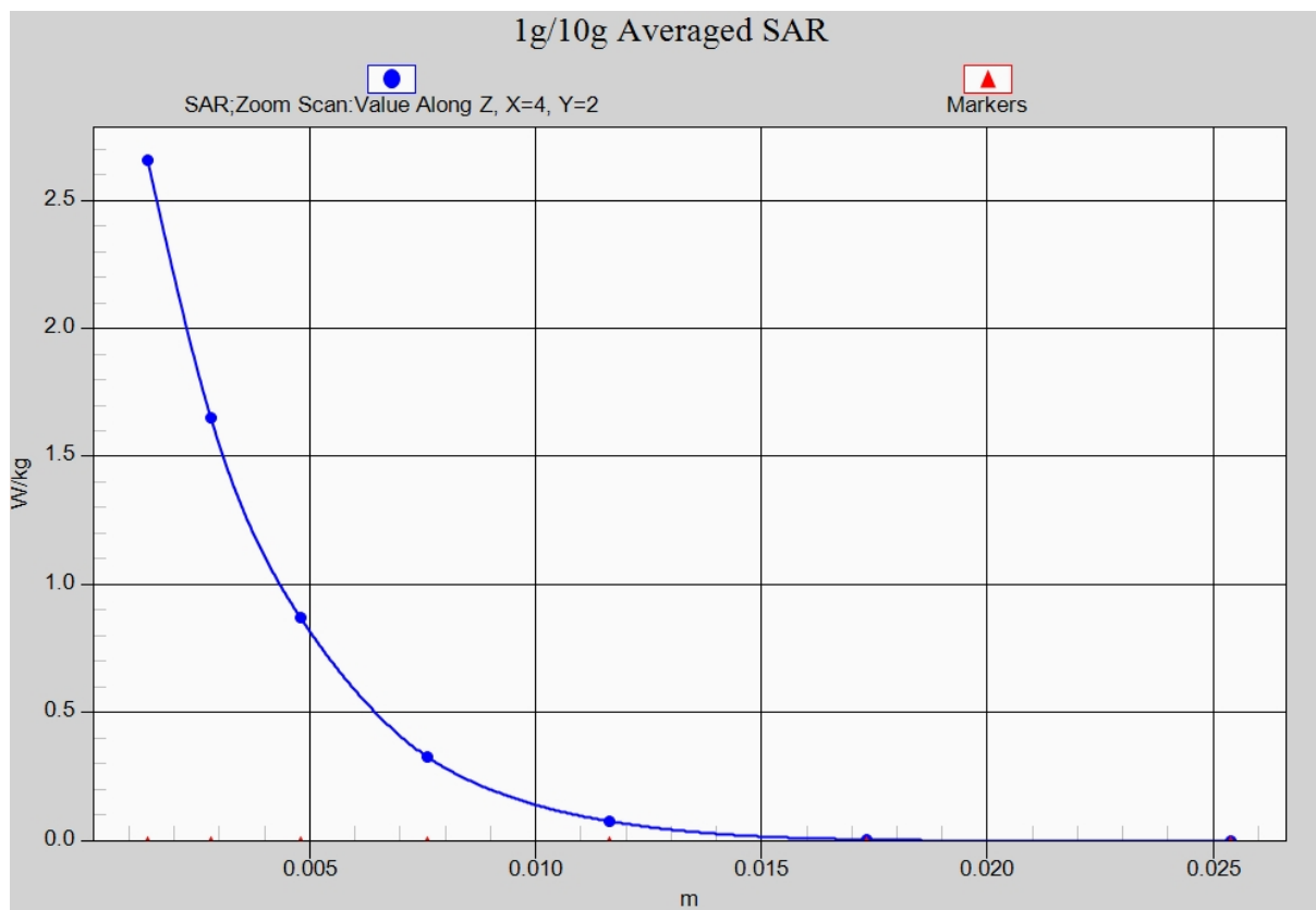
Fig. 17-1 Z-Scan at power reference point (5GHz CH52)
