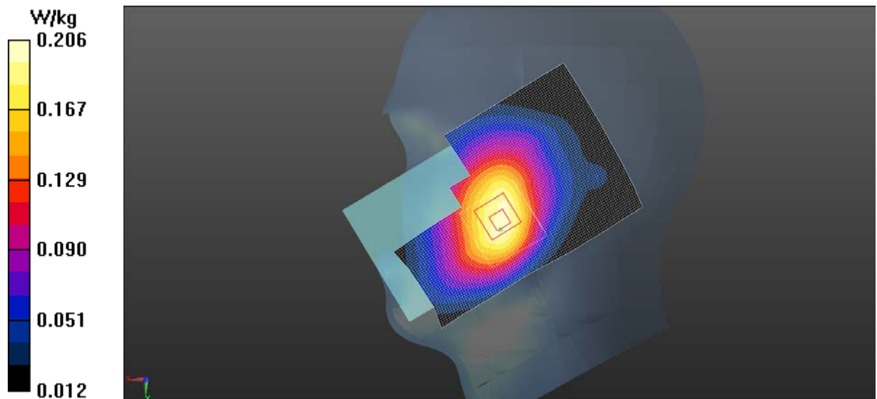
Fig.1 850MHz CH251
