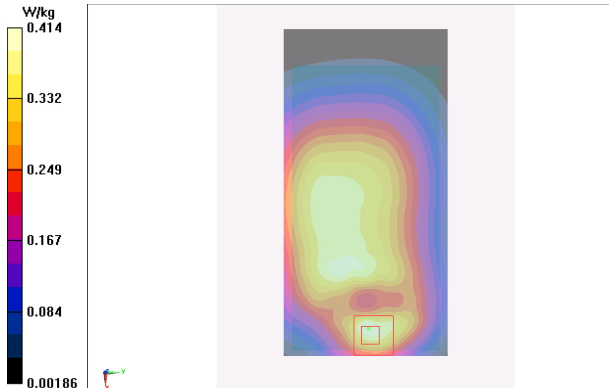
Fig.2 850 MHz CH251
