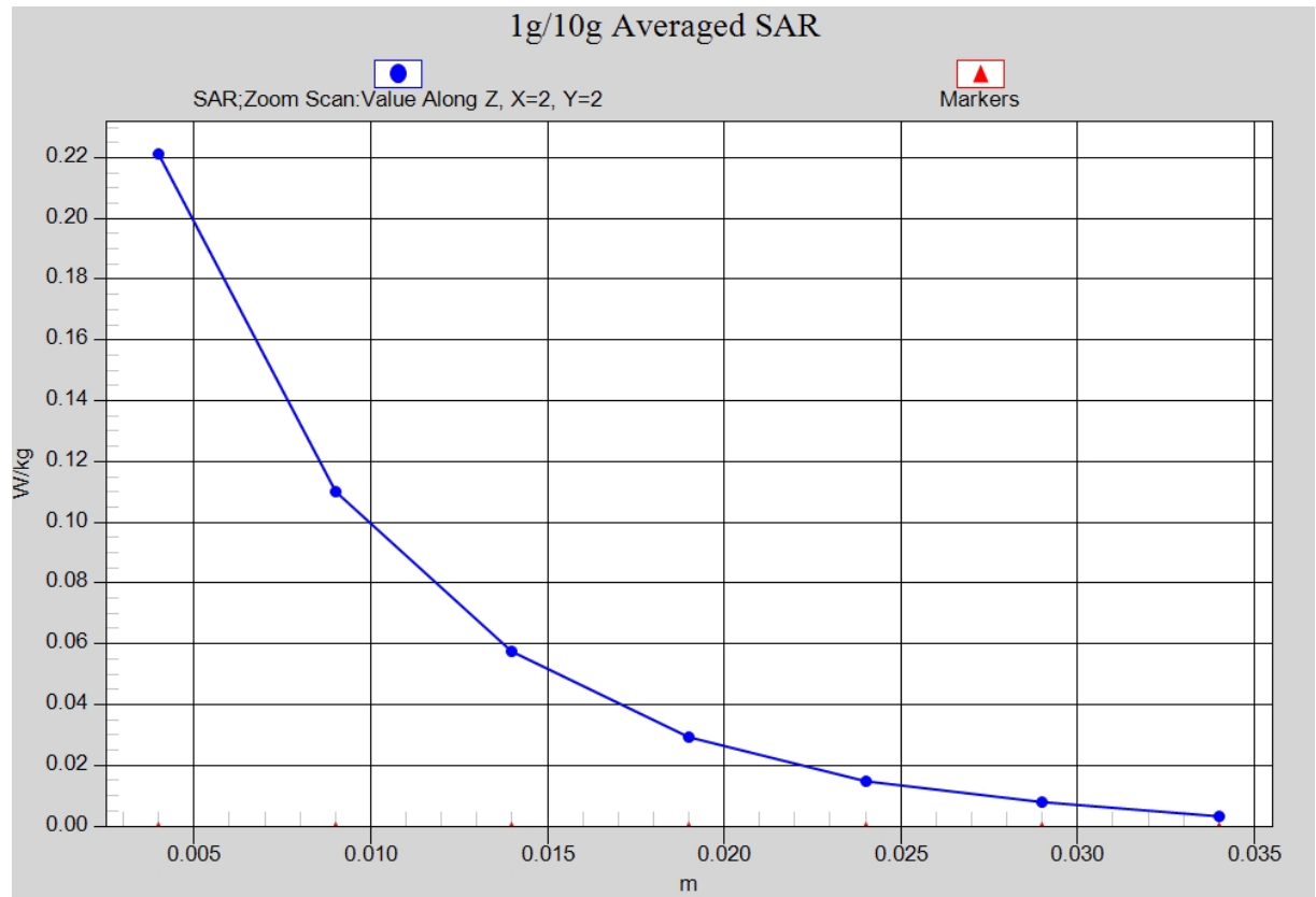
Fig. 16-1 Z-Scan at power reference point (2450 MHz CH1)
