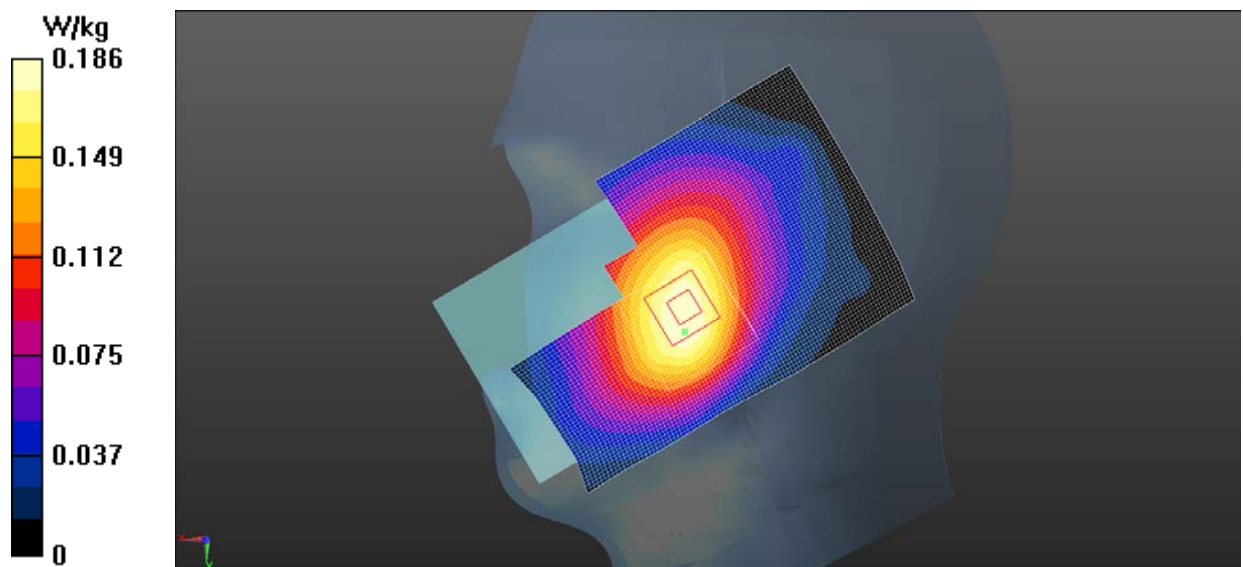
Fig.5 WCDMA 850 CH4233
