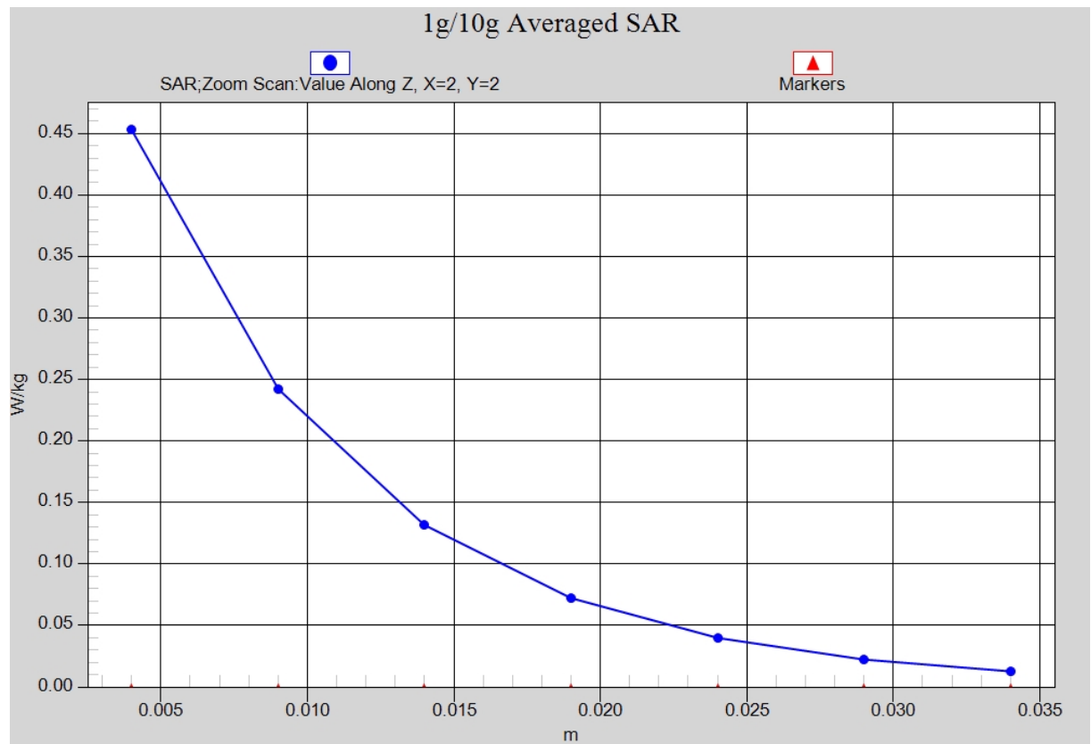
Fig. 13-1 Z-Scan at power reference point (LTE Band7 CH21350)
