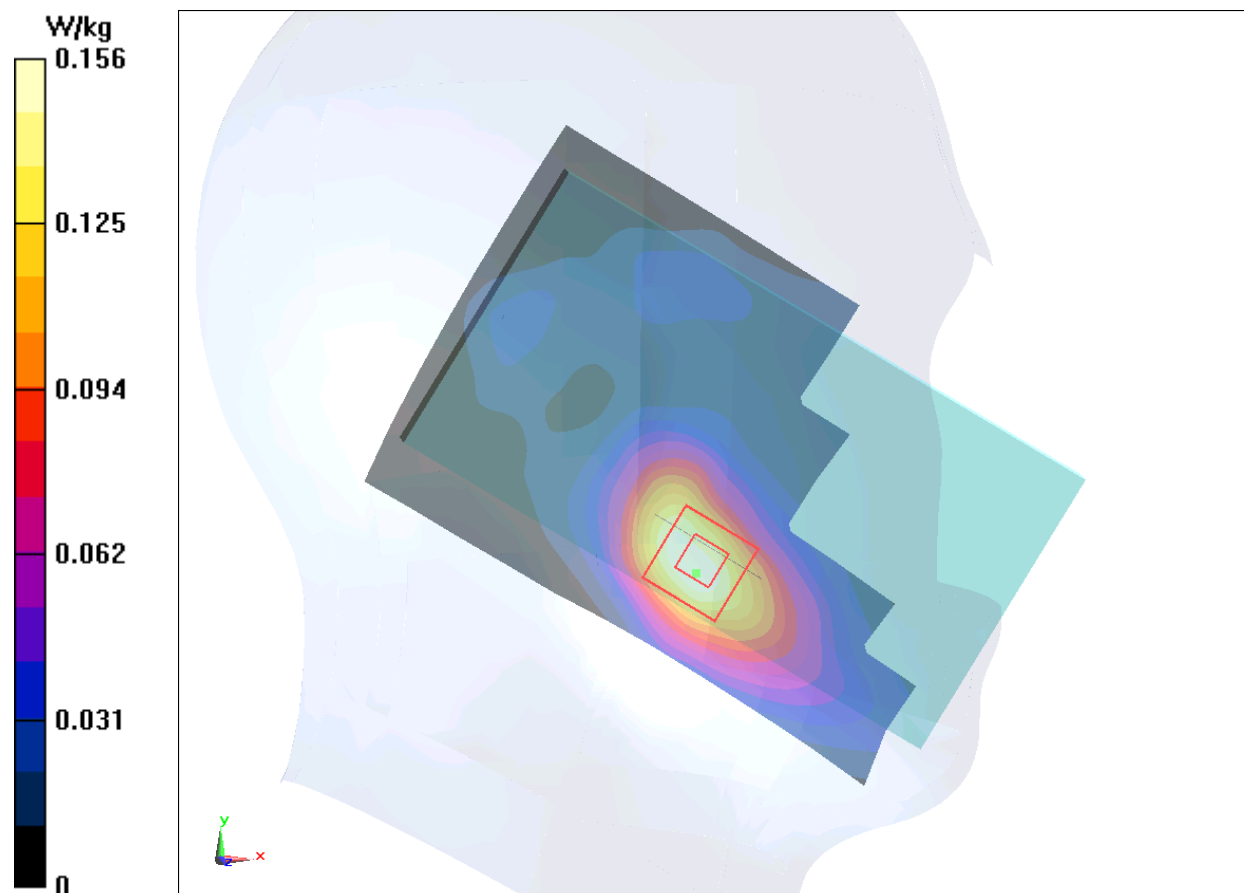
Fig.9 LTE Band2 CH19100
