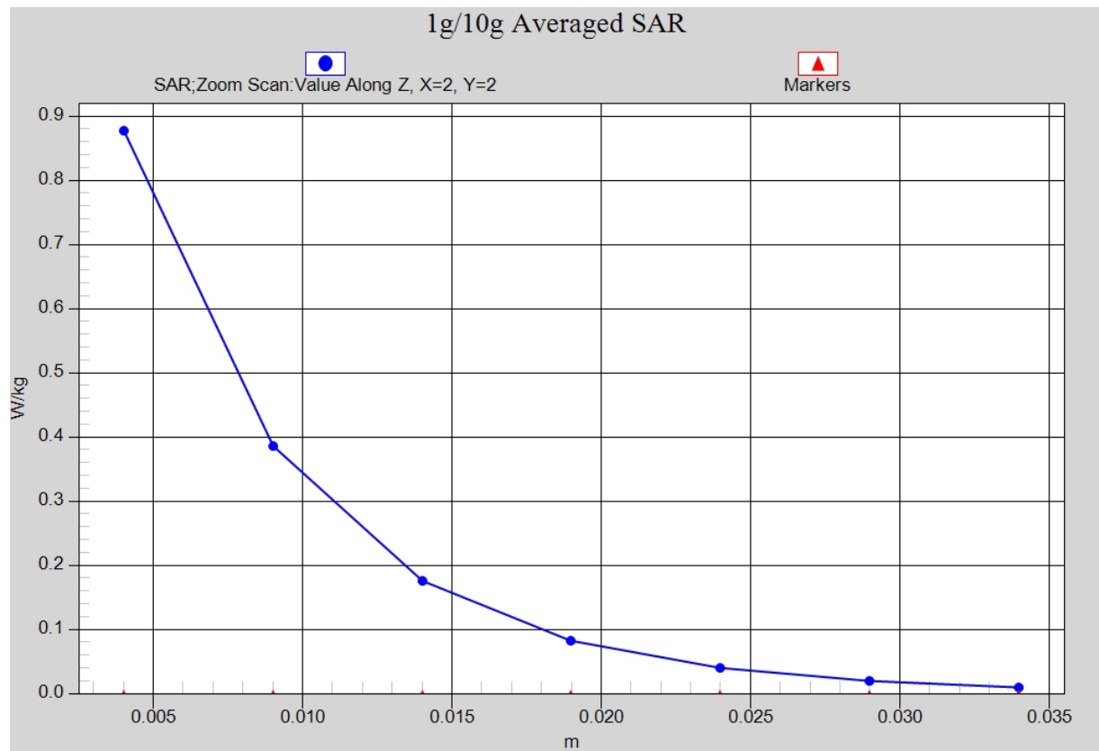
Fig. 15-1 Z-Scan at power reference point (2450 MHz CH1)
