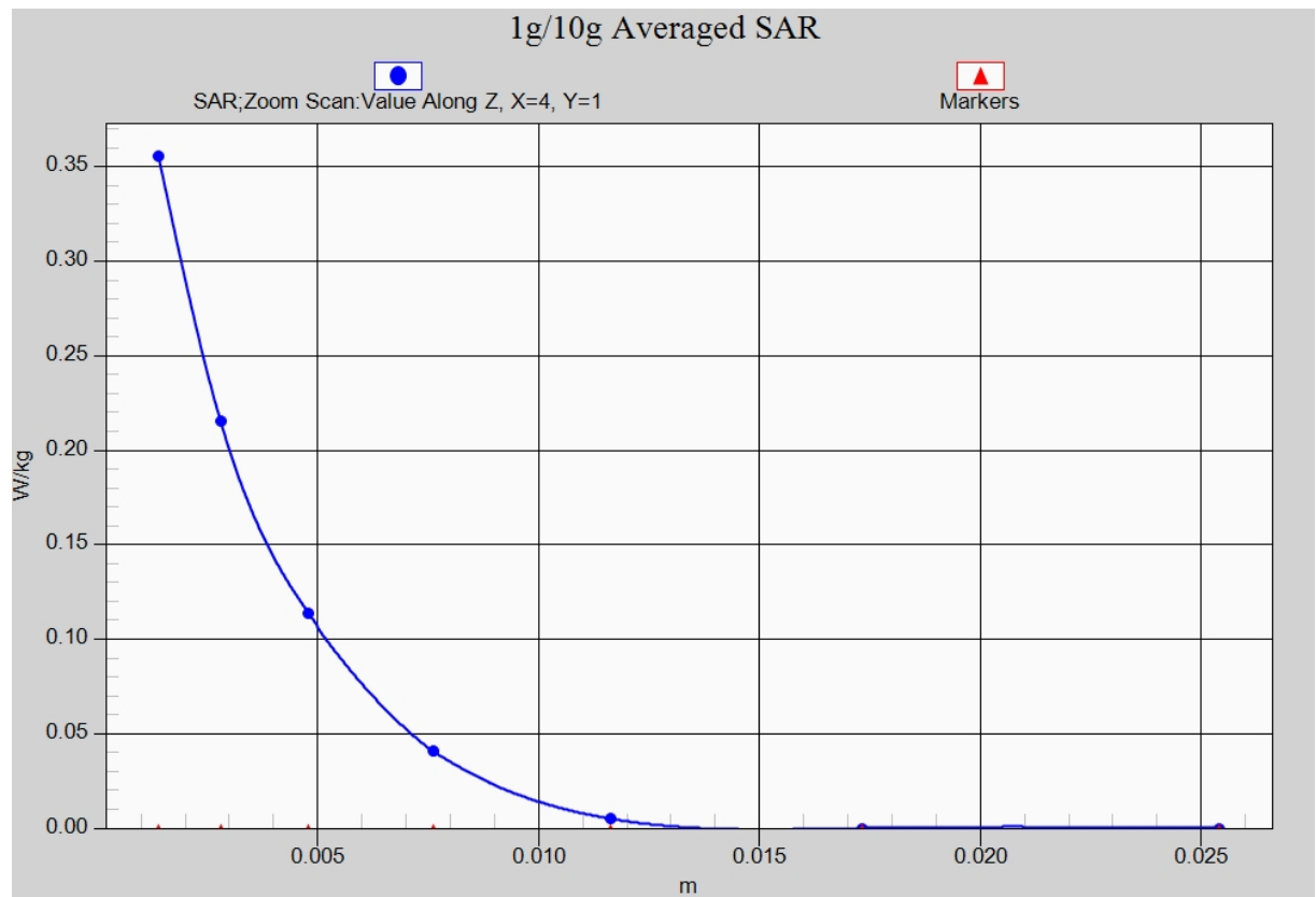
Fig. 18-1 Z-Scan at power reference point (5GHz CH52)
