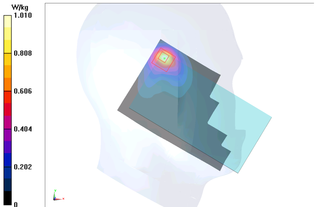
Fig.15 2450 MHz CH1
