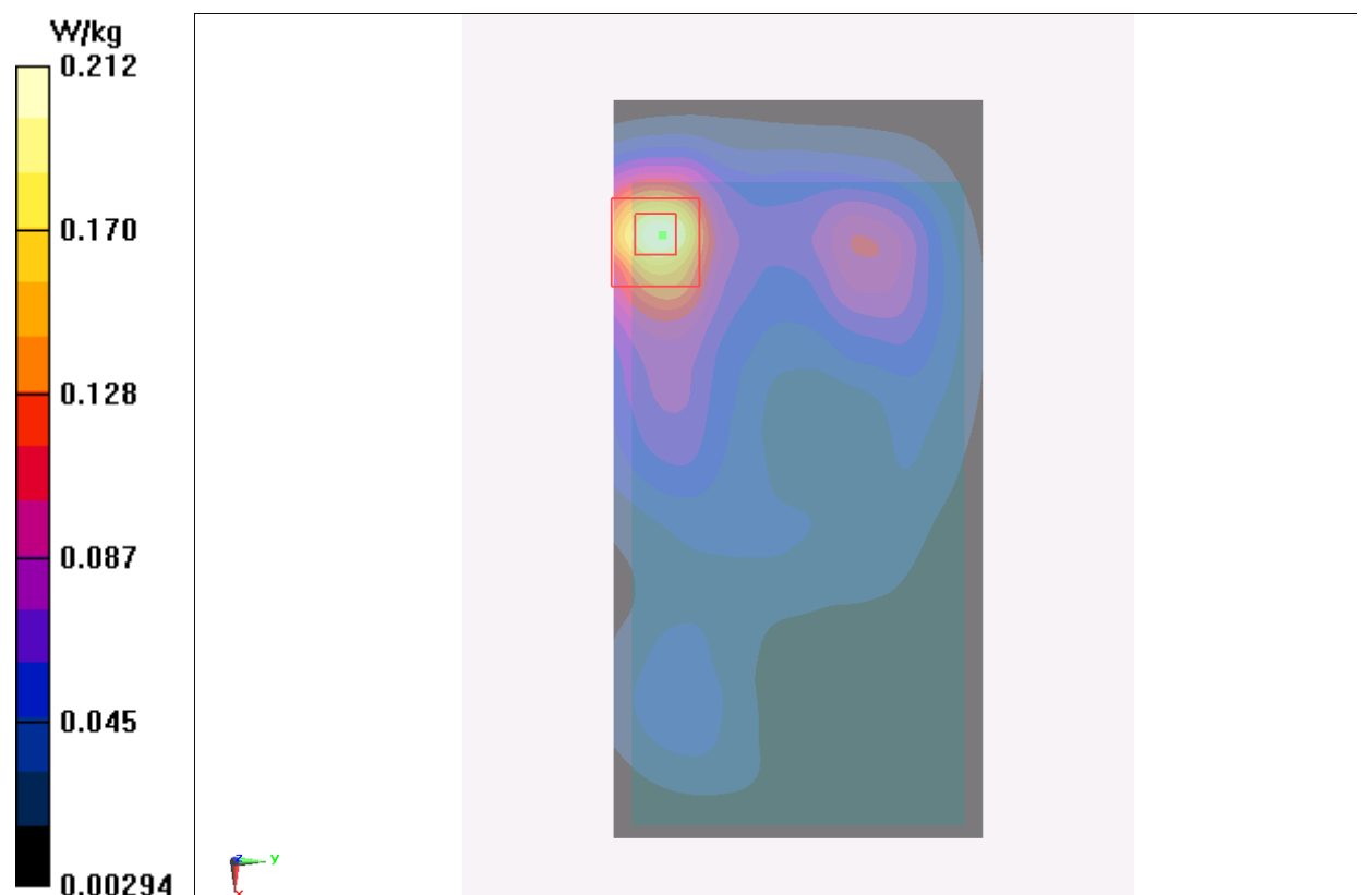
Fig.16 2450 MHz CH1
