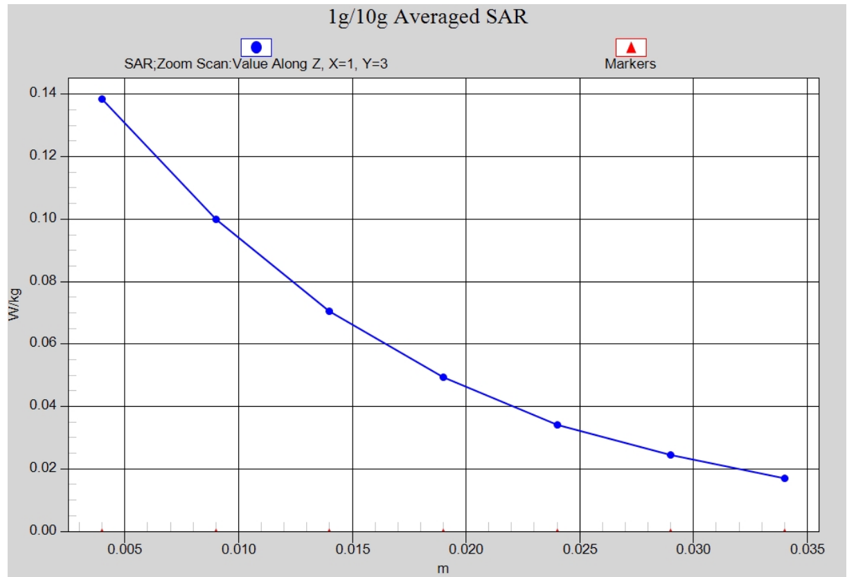
Fig. 9-1 Z-Scan at power reference point (LTE Band2 CH19100)
