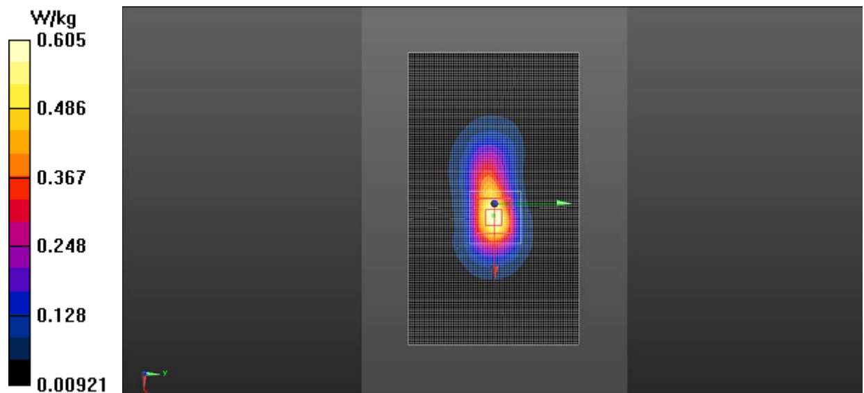
Fig.4 1900 MHz CH810
