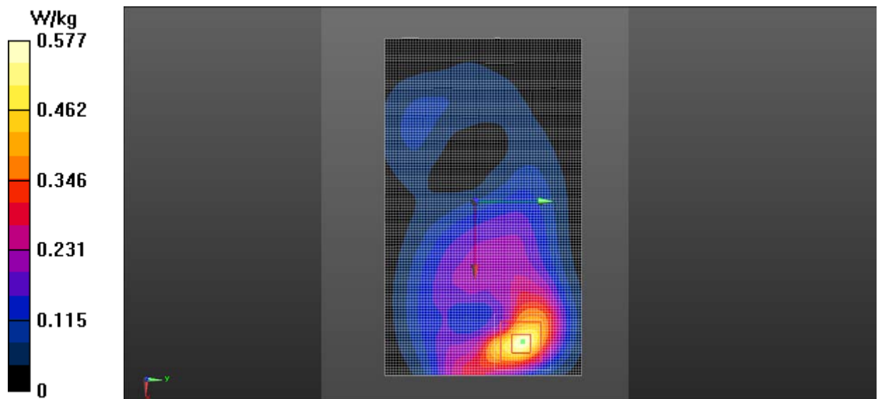
Fig.10 LTE Band2 CH19100
