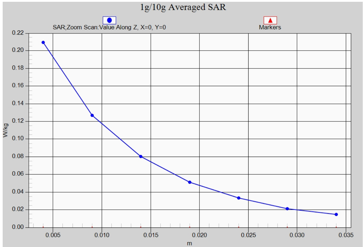
Fig. 12-1 Z-Scan at power reference point (LTE Band4 CH20050)
