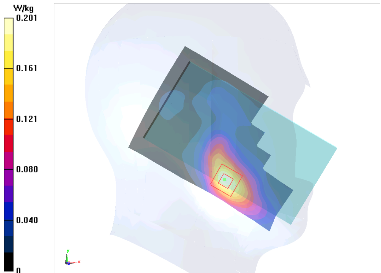
Fig.4 1900 MHz CH810
