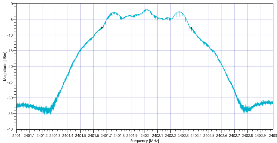
Plot_FCC Part 15.247 Maximum Peak Conducted Output Power DTS ~ BT LE 1 Msps DTS BW_12022021_153721.png
