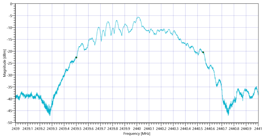
Plot_FCC Part 15.247 Bandwidth 99PCT-20dB ~ BT LE 1 Msps 99PCT_12022021_154443.png
