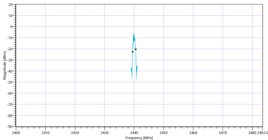
Plot_FCC Part 15.247 Bandwidth 99PCT-20dB ~ BT LE 1 Msps_12022021_154449.png
