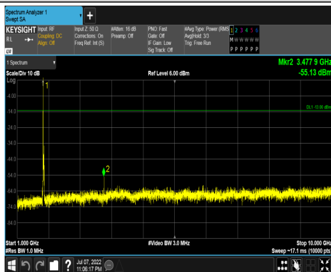
Band66-15MHz-QPSK-132322-1RB#0-Range3:1000~10000MHz
