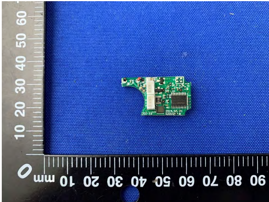
SECONDARY BOARD 11 TOP VIEW
