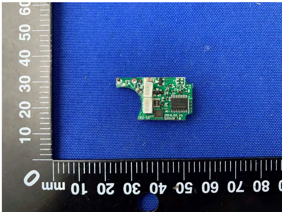
SECONDARY BOARD 10 TOP VIEW
