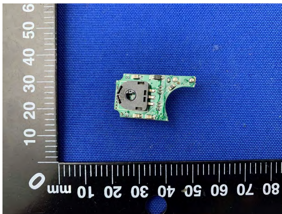
SECONDARY BOARD 16 REAR VIEW
