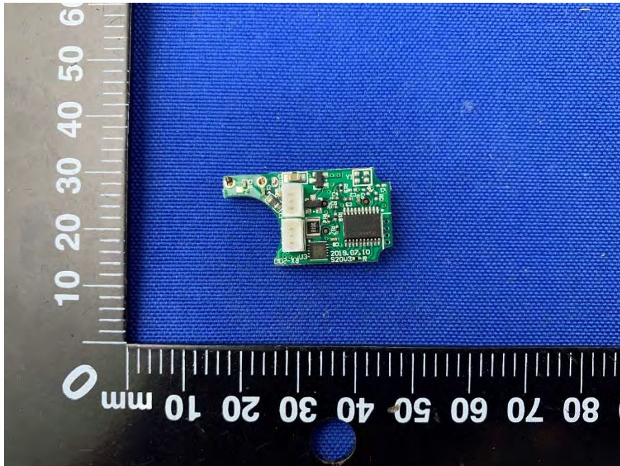
SECONDARY BOARD 15 TOP VIEW
