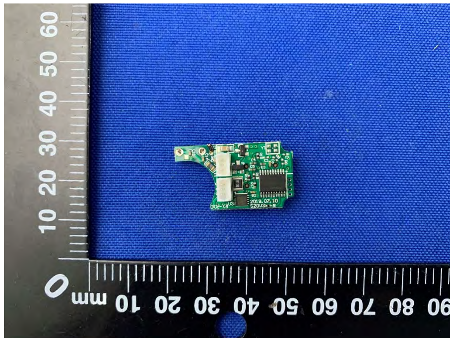
SECONDARY BOARD 17 TOP VIEW
