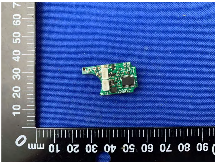
SECONDARY BOARD 14 TOP VIEW
