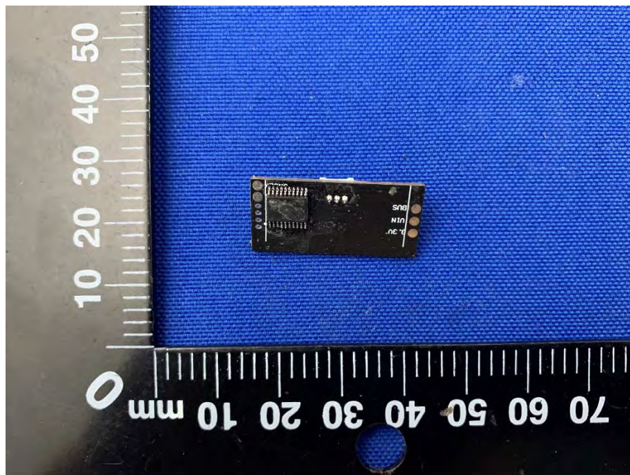
SECONDARY BOARD 18 REAR VIEW
