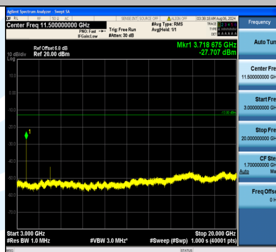
Band2_10MHz_QPSK_18650_1RB#49_3000~20000_3000~20000
