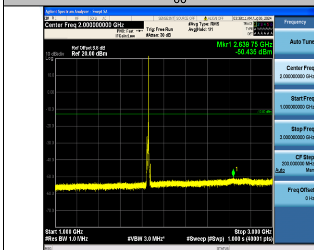
Band2_10MHz_QPSK_18650_1RB#49_1000~3000_1000~3000
