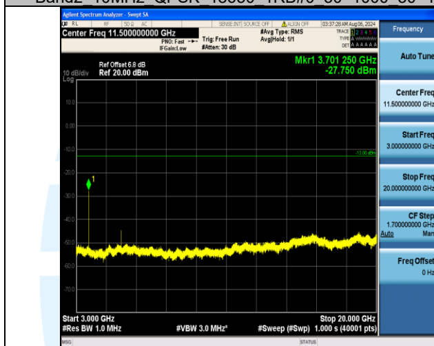
Band2_10MHz_QPSK_18650_1RB#0_3000~20000_3000~20000
