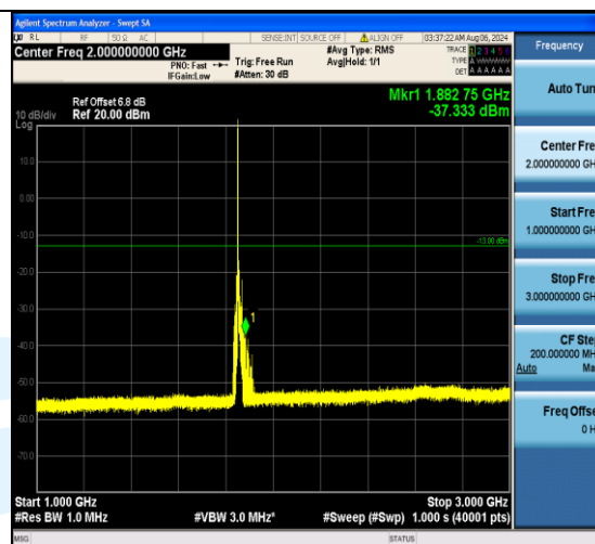
Band2_10MHz_QPSK_18650_1RB#0_1000~3000_1000~3000
