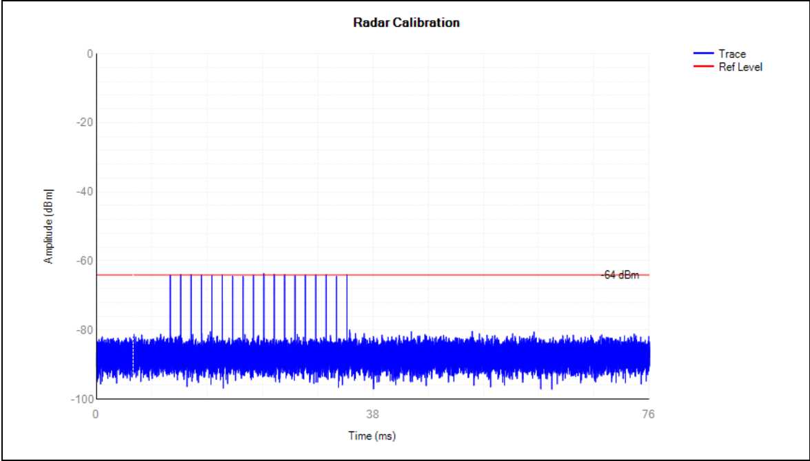
Radar Signal Type 5 ABAB
