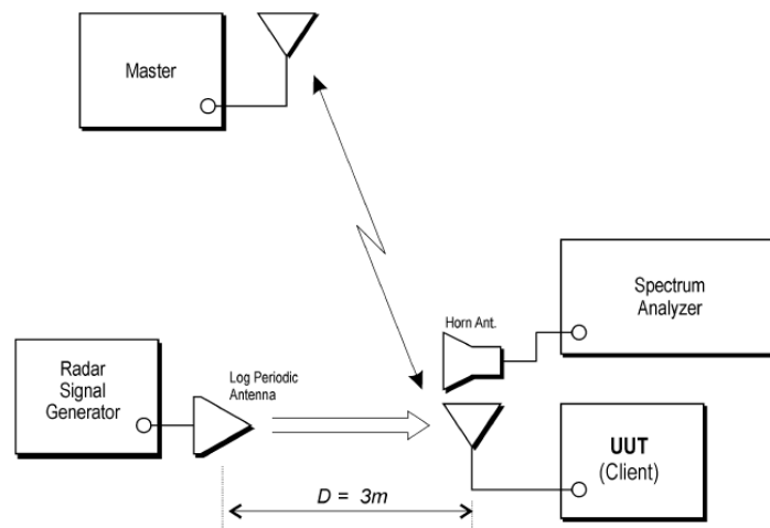
Figure 7: Example Radiated Setup where UUT is a Client and radar Test Waveforms are injected into the Client
