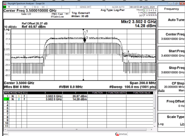
Band77-Part27_100MHz_CP_OFDM_SCS30kHz_256QAM_RB273_0_Chain1_CH633334
