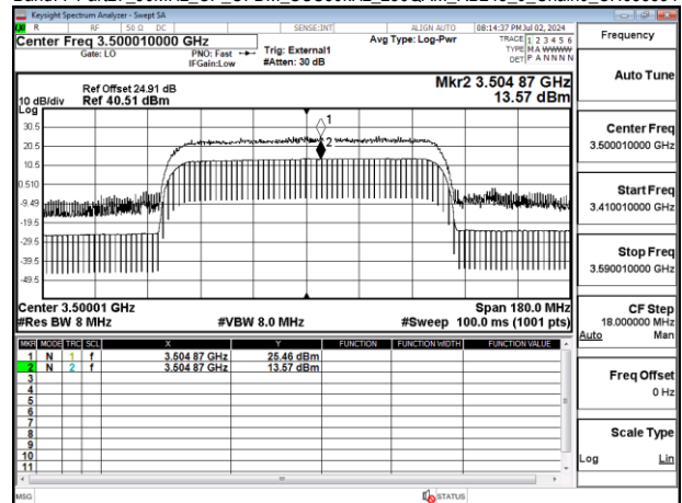
Band77-Part27_90MHz_CP_OFDM_SCS30kHz_256QAM_RB245_0_Chain0_CH633334
