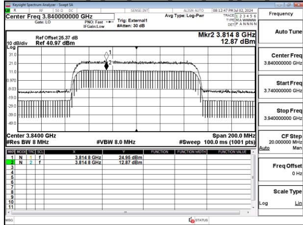
Band77-Part27_100MHz_CP_OFDM_SCS30kHz_256QAM_RB273_0_Chain0_CH662000
