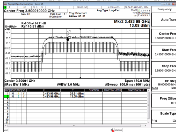
Band77-Part27_90MHz_CP_OFDM_SCS30kHz_256QAM_RB245_0_Chain1_CH633334
