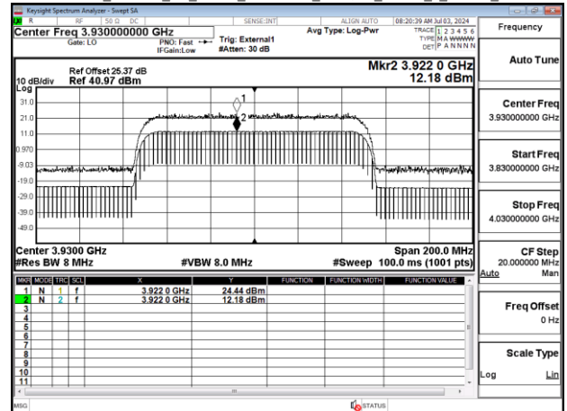
Band77-Part27_100MHz_CP_OFDM_SCS30kHz_256QAM_RB273_0_Chain1_CH662000
