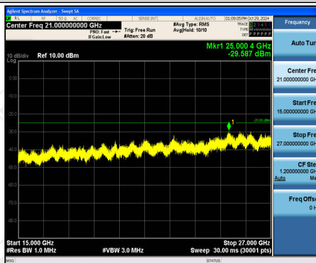
Band7-5MHz-16QAM-20775-1RB#0-Range3:15000~27000MHz
