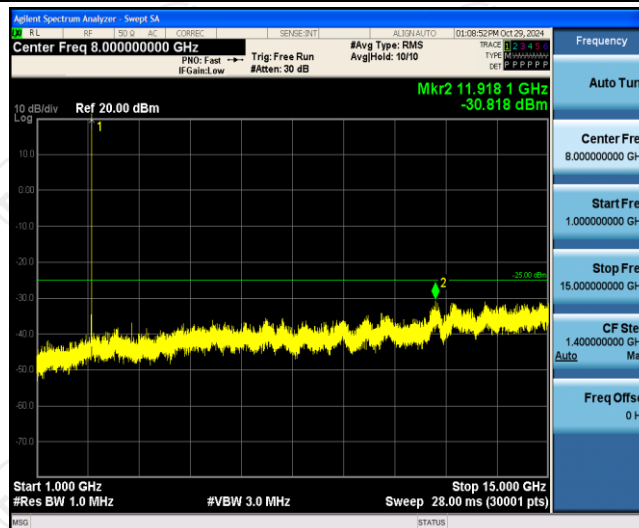
Band7-5MHz-16QAM-20775-1RB#0-Range2:1000~15000MHz
