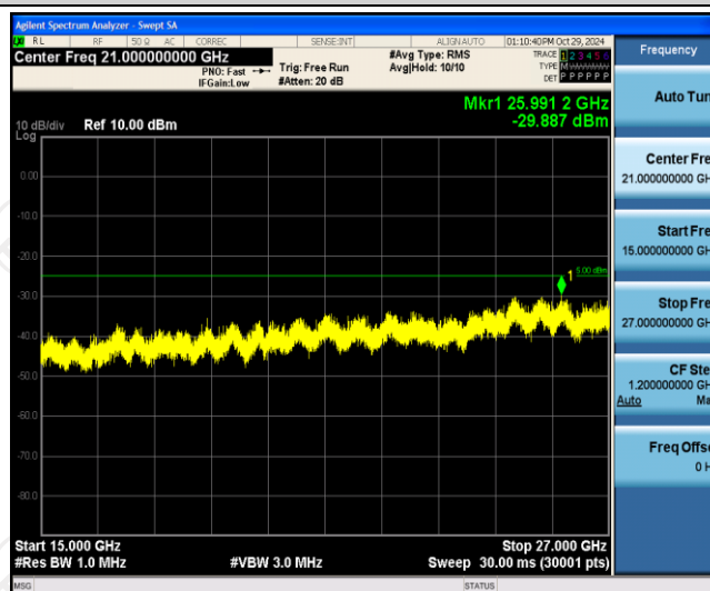
Band7-5MHz-16QAM-21100-1RB#0-Range3:15000~27000MHz
