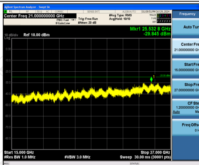
Band7-5MHz-QPSK-21100-1RB#0-Range3:15000~27000MHz
