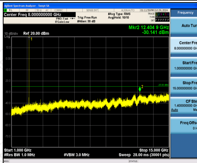
Band7-5MHz-16QAM-21425-1RB#0-Range2:1000~15000MHz
