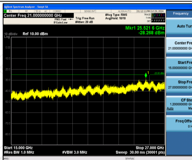
Band7-5MHz-16QAM-21425-1RB#0-Range3:15000~27000MHz
