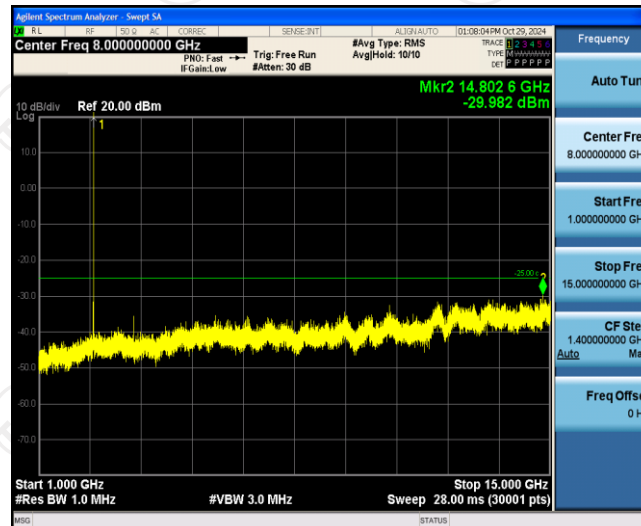
Band7-5MHz-QPSK-20775-1RB#0-Range2:1000~15000MHz
