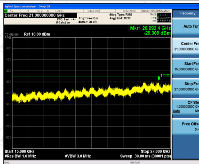
Band7-5MHz-QPSK-20775-1RB#0-Range3:15000~27000MHz
