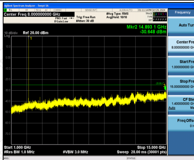
Band7-5MHz-QPSK-21425-1RB#0-Range2:1000~15000MHz
