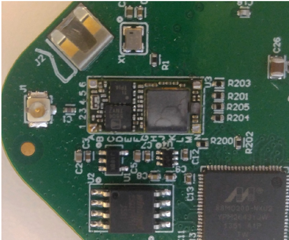
Figure 3. RF Circuit, Shielding removed
