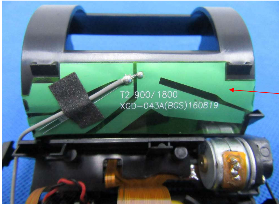
GPRS Antenna
