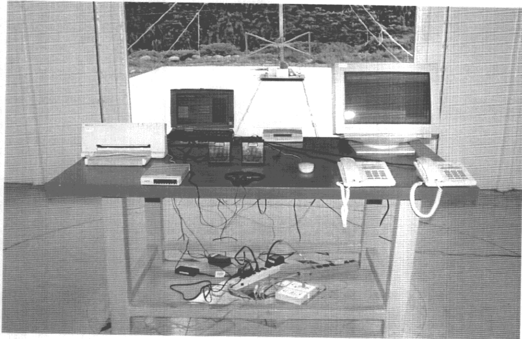
FRONT VIEW OF RADIATED TEST ( Worst Case Test Setup, mode 2)
