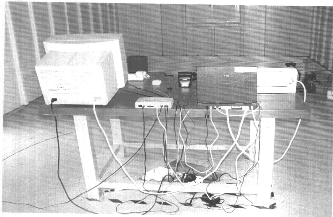
BACK VIEW OF RADIATED TEST ( Worst Case Test Setup, mode 2)
