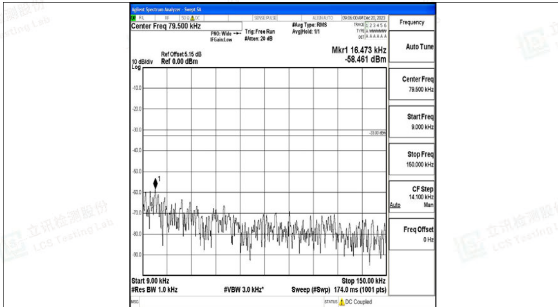
Band26_10MHz_QPSK_26915_1RB#0_0.009~0.15_0.009~0.15
