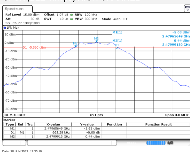
GFSK (BLE 1Mbps) HIGH CHANNEL
