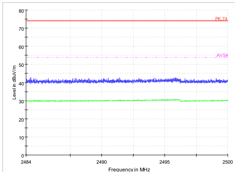
Radiated Emission Band Edge Channel No.:39 Test Mode: GFSK (LE 2Mbps) Polarization: H
