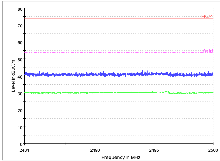
Radiated Emission Band Edge Channel No.:39 Test Mode: GFSK (LE 1Mbps) Polarization: V
