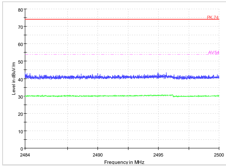
Radiated Emission Band Edge Channel No.:39 Test Mode: GFSK (LE 2Mbps) Polarization: V
