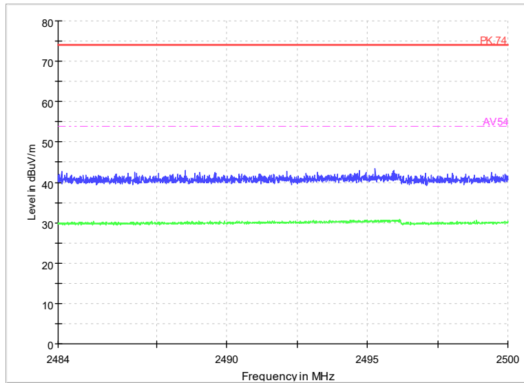
Radiated Emission Band Edge Channel No.:39 Test Mode: GFSK (LE 1Mbps) Polarization: H
