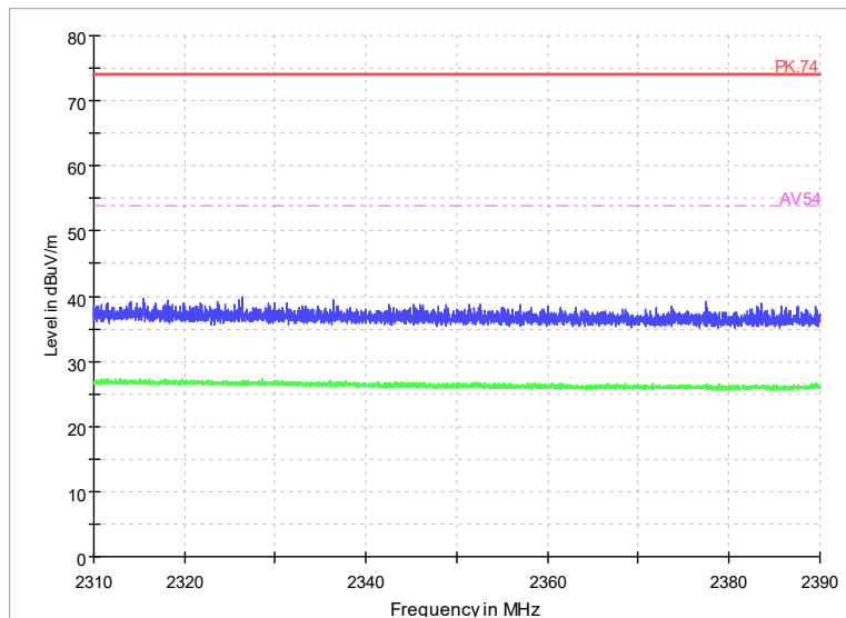
Radiated Emission Band Edge Channel No.:0 Test Mode: GFSK (LE 2Mbps) Polarization: H
