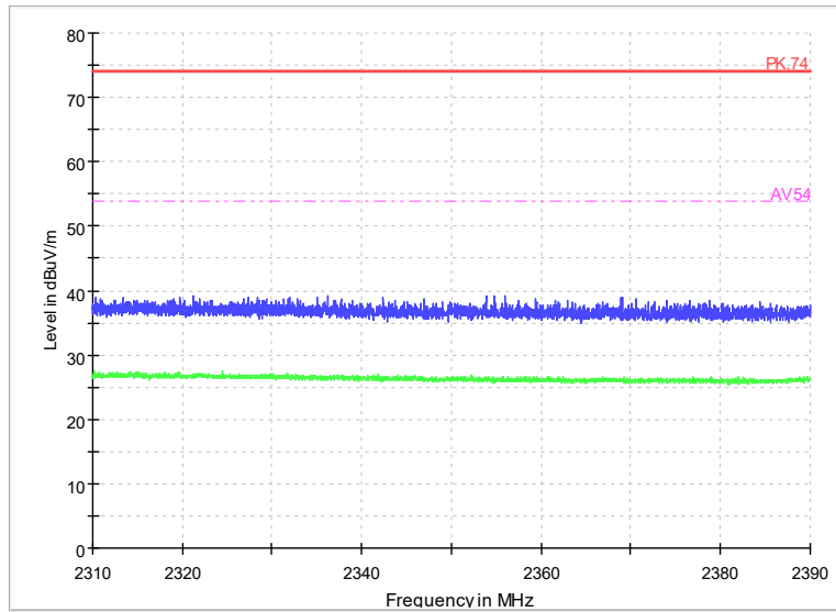
Radiated Emission Band Edge Channel No.:0 Test Mode: GFSK (LE 2Mbps) Polarization: V
