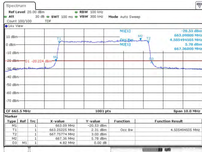
Band71-5MHz-QPSK-133147-25RB#0-4.505
