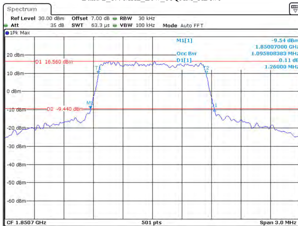
Band 2 1.4 MHz Low 16QAM RB6#0
