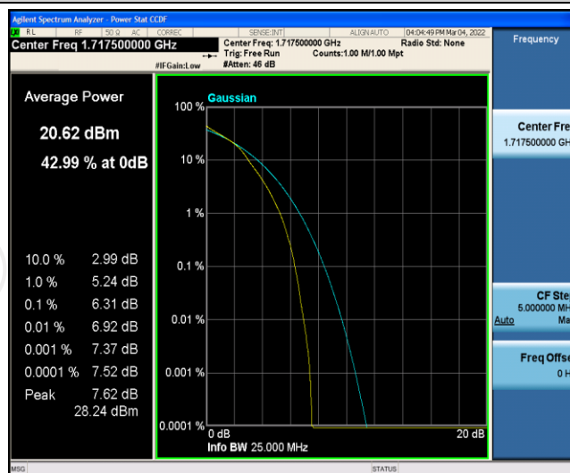
Band66-15MHz-16QAM-132322-1RB#0
