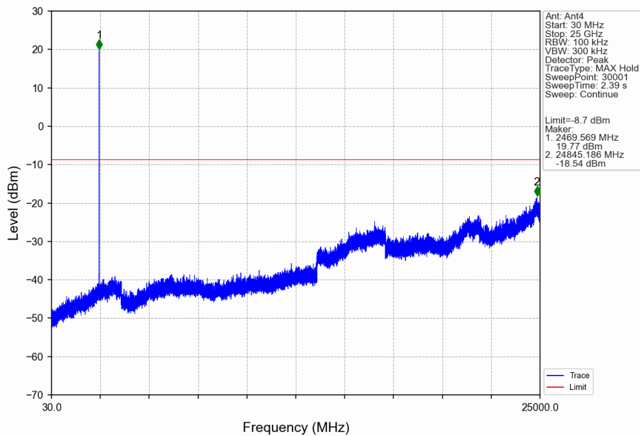
1.4M_HCH_2469.12MHz_Ant4_NTNV
