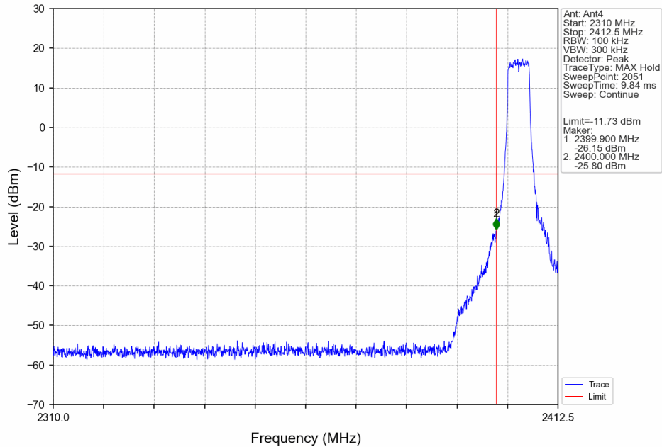
5M_LCH_2404.5MHz_Ant4_NTNV
