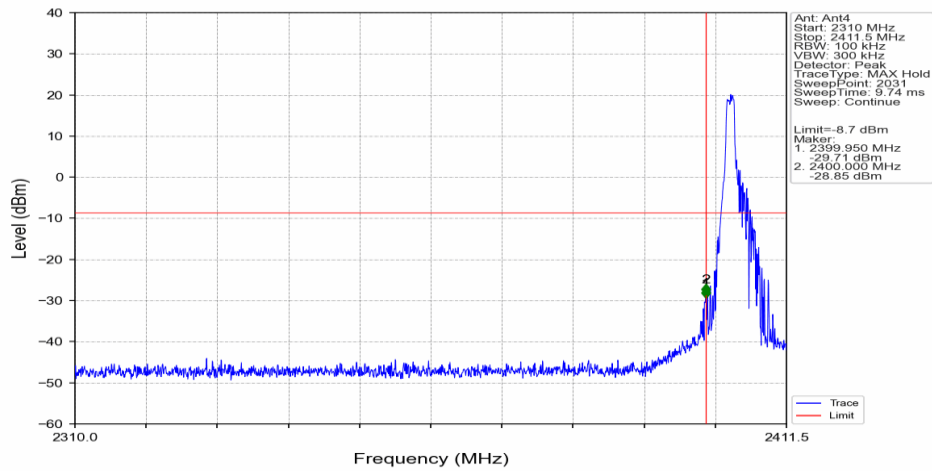
1.4M_LCH_2403.5MHz_Ant4_NTNV
