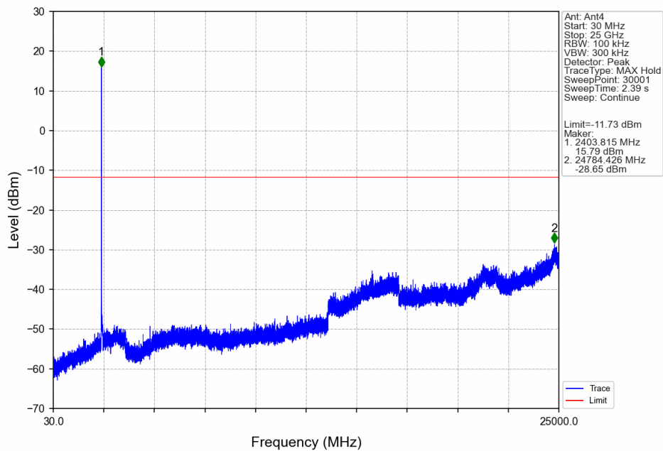
5M_LCH_2404.5MHz_Ant4_NTNV
