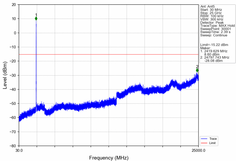
40M_LCH_2422.5MHz_Ant5_NTNV
