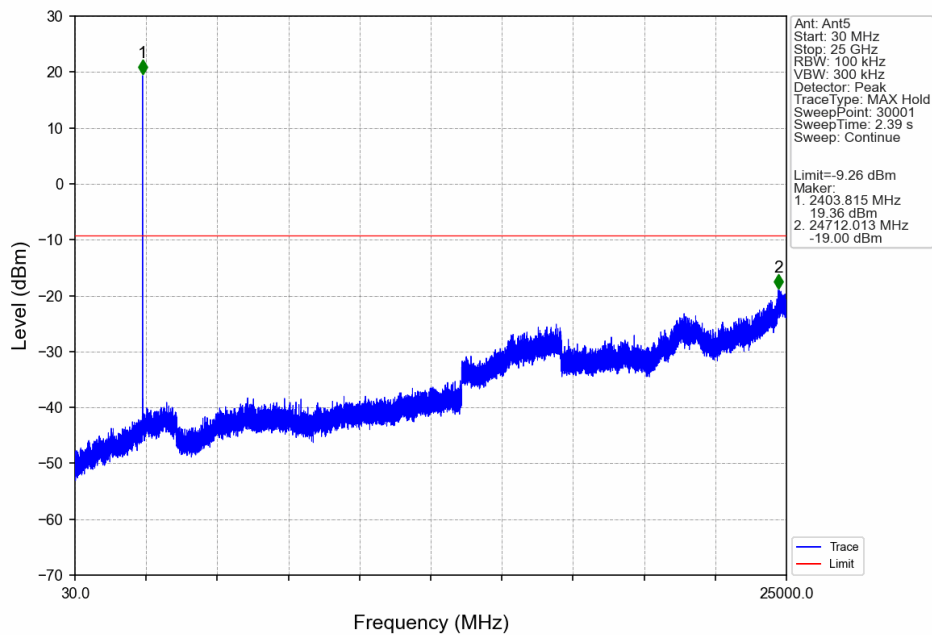
1.4M_LCH_2403.5MHz_Ant5_NTNV
