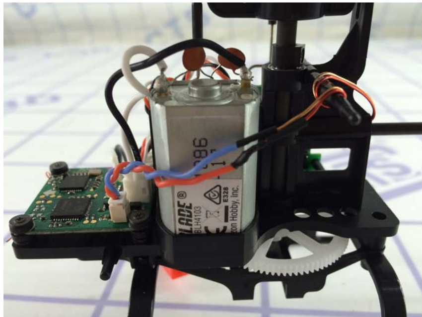
Motor view
