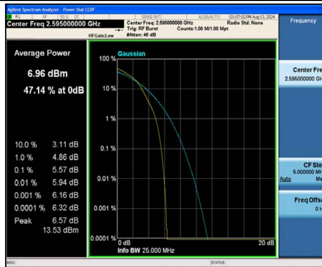
Band38-10MHz-16QAM-38000-27RB#0
