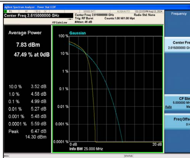
Band38-10MHz-16QAM-38200-27RB#0
