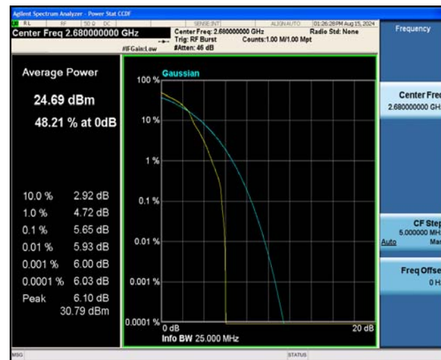
Band41-20MHz-16QAM-41490-27RB#0
