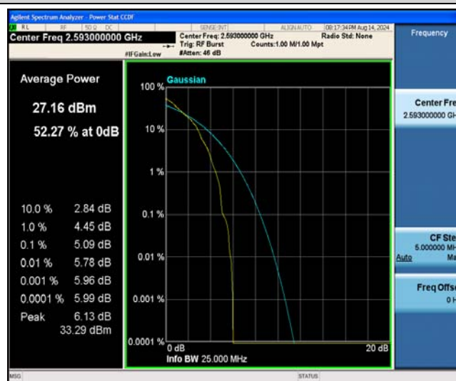
Band41-10MHz-QPSK-40620-50RB#0
