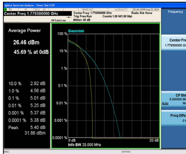
Band66-1.4MHz-16QAM-132665-6RB#0
