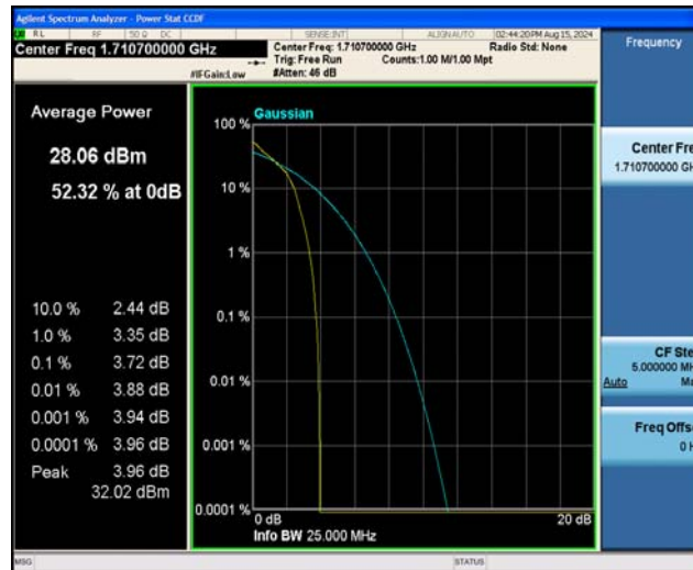
Band66-1.4MHz-QPSK-131979-6RB#0
