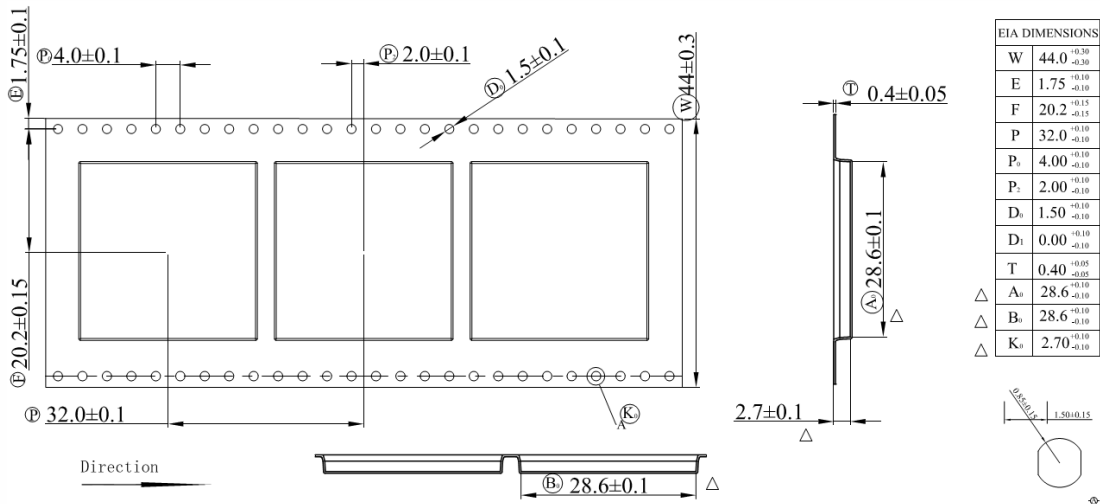
Figure 32: Carrier Tape Detail
