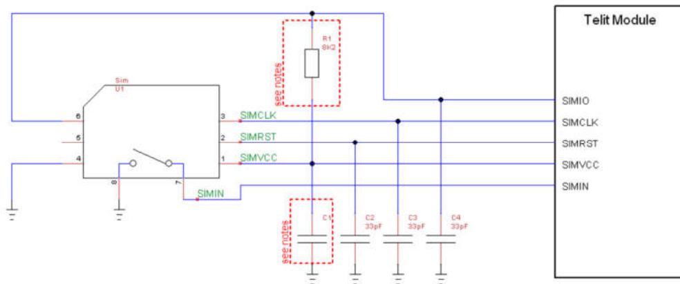
Figure 28: SIM Schematics
