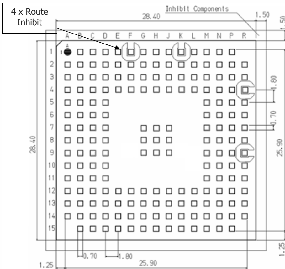
Figure 24: Recommended Footprint - Top View, 181 pads
