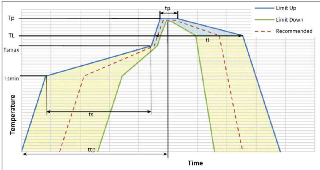
Figure 27: Solder Reflow Profile
