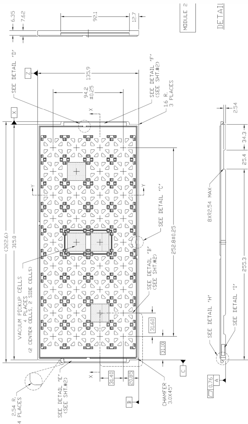
Figure 30: Tray Drawing
