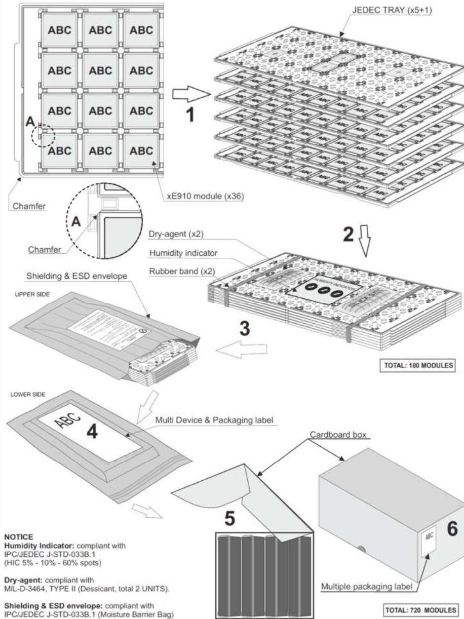
Figure 29: Packing
