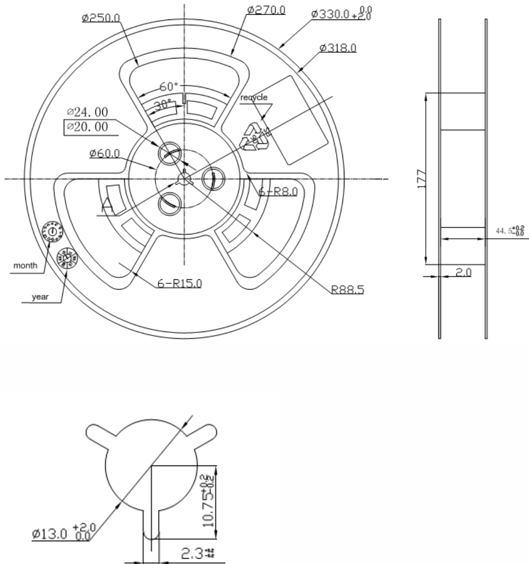
Figure 33: Reel Detail
