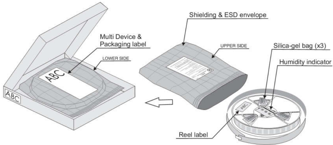
Figure 34: Reel Box Detail
