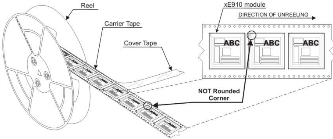
Figure 32: Carrier Tape Detail
