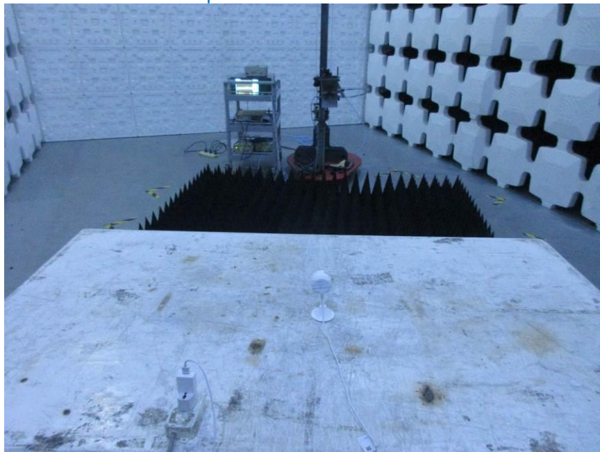
Adaptor 2: TPA-46B050100UU
