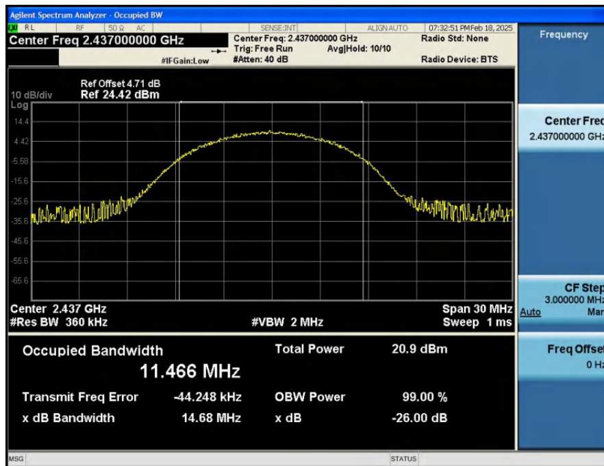
99%_Occupied_Bandwidth_NVNT_ANT1_802_11b_2437
