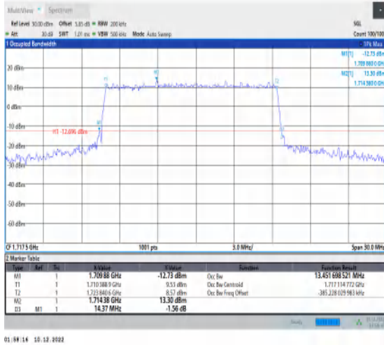
1-N66-15-15-L-3-DFT-16QAM-Outer_Full-75@0-Ant t1-13.452-14.370≤15-PASS
