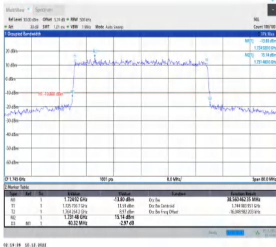
1-N66-15-40-M-1-DFT-QPSK-Outer_Full-216@0-Ant 1-38.56-40.320-≤40-PASS
