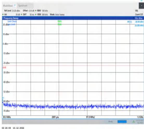
1-N66-15-40-M-1-DFT-PI2BPSK-Inner_1RB_Left-1 @ 1-30-1000-Ant1-33.40--59.94--23-PASS
