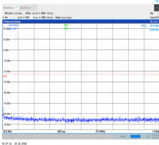
1-N66-15-40-H-1-DFT-PI2BPSK-Inner_1RB_Left-1 @1-30-1000-Ant1-34.85--58.19--23-PASS
