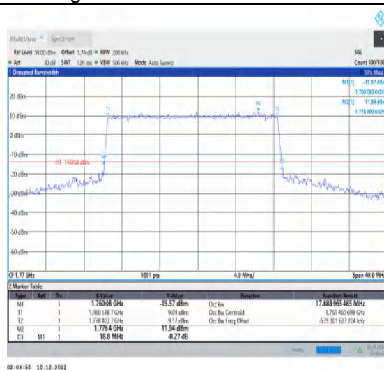
1-N66-15-20-H-3-DFT-16QAM-Outer_Full-100@0-A Ant1-17.884-18.800-≤20-PASS
