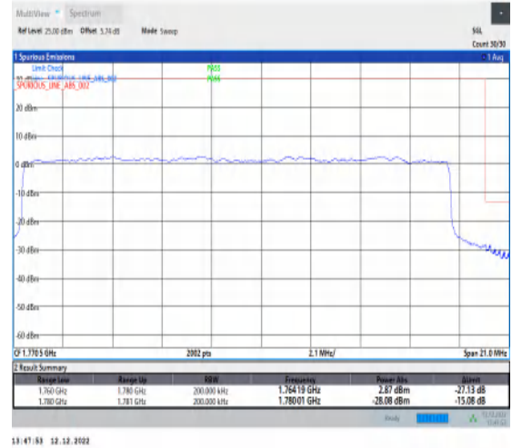
1-N66-15-20-H-3-DFT-PI2BPSK-Outer_Full-100@0-Ant1-1-seegraph-PASS-see graph
