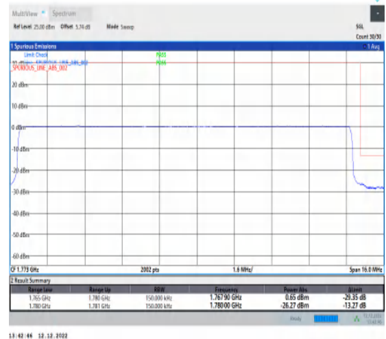
1-N66-15-15-H-6-CP-QPSK-Outer_Full-79@0-Ant1-1-seegraph-PASS-see graph
