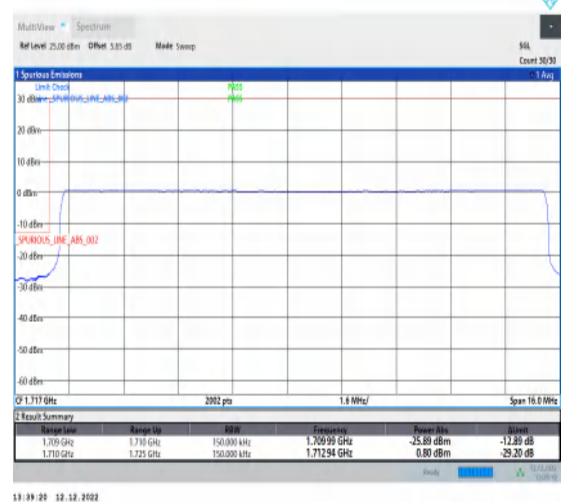
1-N66-15-15-L-6-CP-QPSK-Outer_Full-79@0-Ant1-1-seegraph-PASS-see graph
