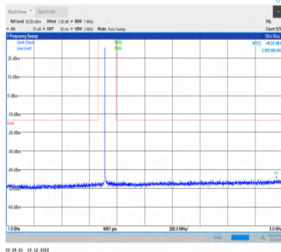
1-N66-15-40-L-1-DFT-PI2BPSK-Inner_1RB_Left-1@ 1-1000-3000-Ant1-2953.00--45.03--13-PASS
