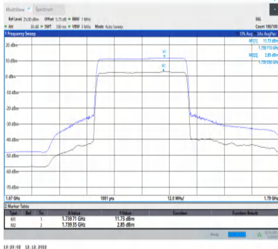
1-N66-15-40-L-1-DFT-256QAM-Outer_Full-216@0-A nt1-8.88-100%-0.00-8.88-PASS-≤13
