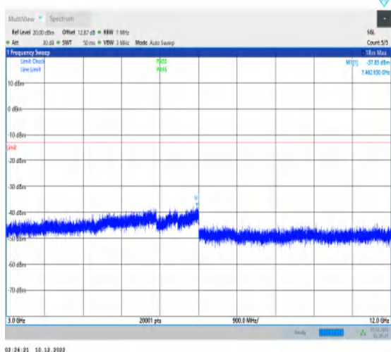
1-N66-15-40-M-1-DFT-PI2BPSK-Inner_1RB_Left-1 @ 1-3000-12000-Ant1-7462.65--37.85--13-PASS
