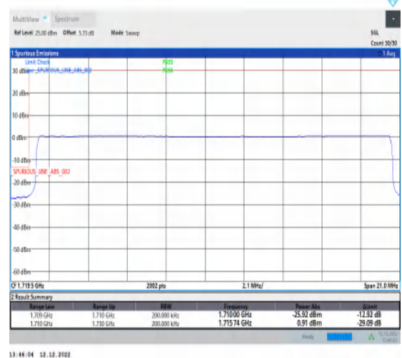
1-N66-15-20-L-6-CP-QPSK-Outer_Full-106@0-Ant1-1-seegraph-PASS-see graph
