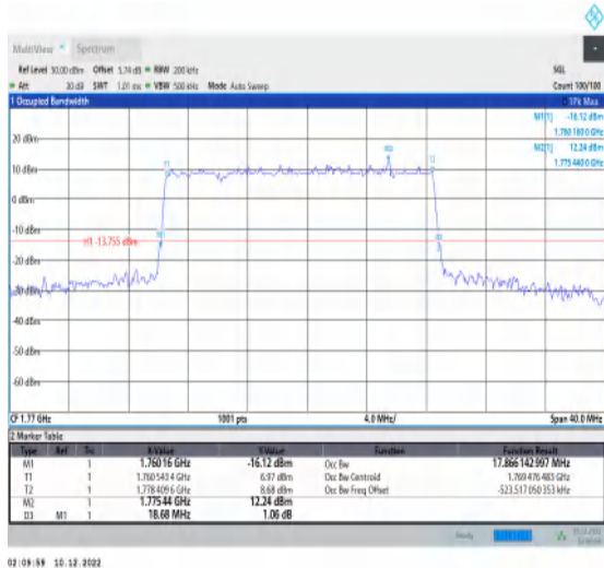
1-N66-15-20-H-4-DFT-64QAM-Outer_Full-100@0-A Ant1-17.866-18.680-≤20-PASS
