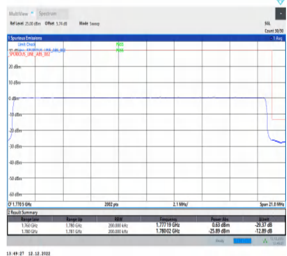
1-N66-15-20-H-6-CP-QPSK-Outer_Full-106@0-Ant1-1-seegraph-PASS-see graph
