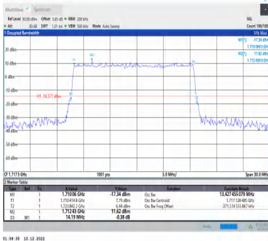
1-N66-15-15-L-5-DFT-256QAM-Outer_Full-75@0-Ant t1-13.427-14.190≤15-PASS
