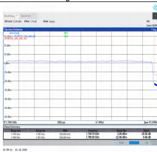
1-N66-15-40-H-3-DFT-PI2BPSK-Outer_Full-216@0-Ant1-1-seegraph-PASS-see graph
