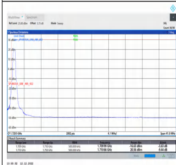
1-N66-15-40-L-4-CP-QPSK-Edge_1RB_Left-1@0-Ant1-1-seegraph-PASS-see graph
