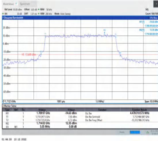
1-N66-15-5-L-1-DFT-QPSK-Outer_Full-25@0-Ant1-4 4.478-5.050-≤5-PASS
