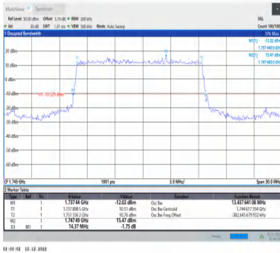
1-N66-15-15-M-2-DFT-PI2BPSK-Outer_Full-75@0-A nt1-13.438-14.370-≤15-PASS
