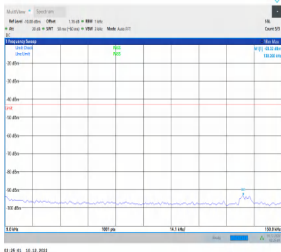
1-N66-15-40-L-1-DFT-PI2BPSK-Inner_1RB_Left-1 @1-0.009-0.15-Ant1-0.13--93.32--43-PASS
