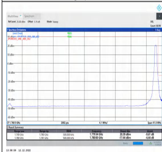
1-N66-15-40-H-5-CP-QPSK-Edge_1RB_Right-1@215-Ant1-1-seegraph-PASS-see graph
