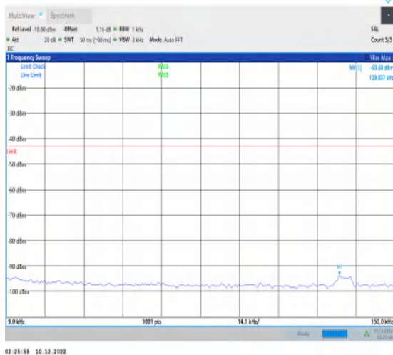
1-N66-15-40-M-1-DFT-PI2BPSK-Inner_1RB_Left-1 @ 1-0.009-0.15-Ant1-0.13--93.68--43-PASS
