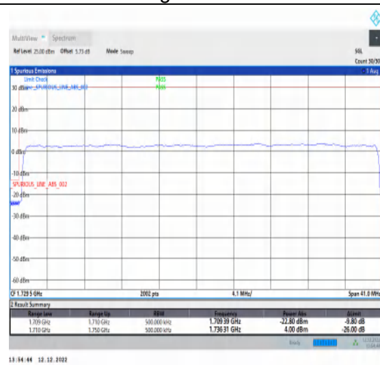
1-N66-15-40-L-3-DFT-PI2BPSK-Outer_Full-216@0-Ant1-1-seegraph-PASS-see graph
