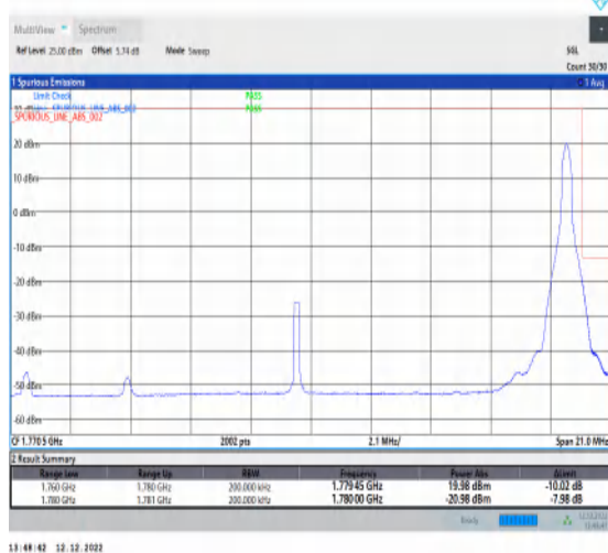
1-N66-15-20-H-5-CP-QPSK-Edge_1RB_Right-1@105-Ant1-1-seegraph-PASS-see graph
