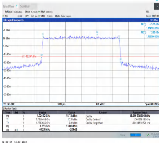
1-N66-15-40-M-3-DFT-16QAM-Outer_Full-216@0-A nt1-38.62-40.240-≤40-PASS
