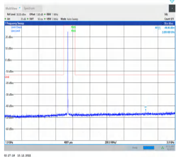
1-N66-15-40-H-1-DFT-PI2BPSK-Inner_1RB_Left-1@ 1-1000-3000-Ant1-2656.00--44.46--13-PASS
