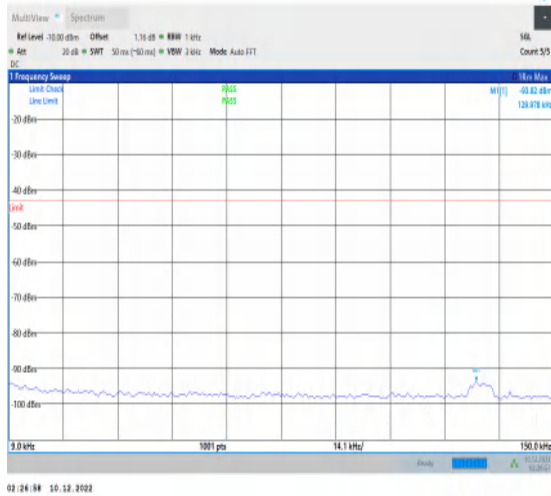
1-N66-15-40-H-1-DFT-PI2BPSK-Inner_1RB_Left-1 @1-0.009-0.15-Ant1-0.13--93.82--43-PASS
