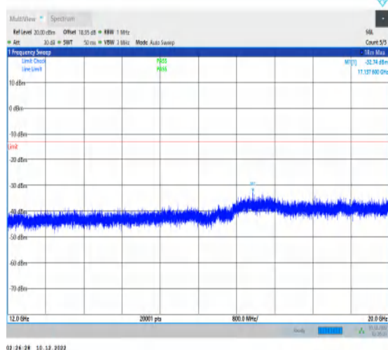
1-N66-15-40-M-1-DFT-PI2BPSK-Inner_1RB_Left-1@ 1-12000-20000-Ant1-17137.60--32.74--13-PASS
