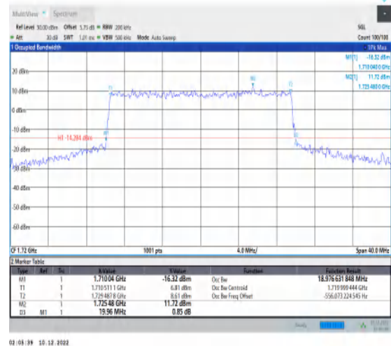
1-N66-15-20-L-7-CP-16QAM-Outer_Full-106@0-Ant 1-18.977-19.960-≤20-PASS
