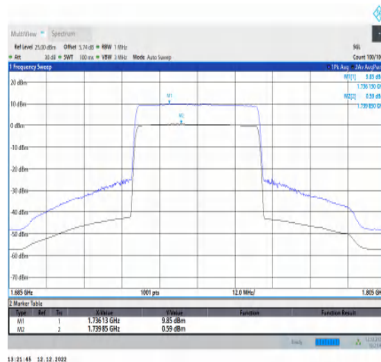
1-N66-15-40-M-2-CP-256QAM-Outer_Full-216@0-A nt1-9.26-100%-0.00-9.26-PASS-≤13
