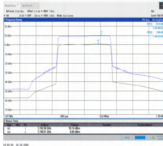
1-N66-15-40-L-2-CP-256QAM-Outer_Full-216@0-A nt1-9.45-100%-0.00-9.45-PASS-≤13
