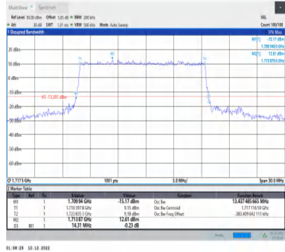
1-N66-15-15-L-4-DFT-64QAM-Outer_Full-75@0-Ant t1-13.437-14.310≤15-PASS
