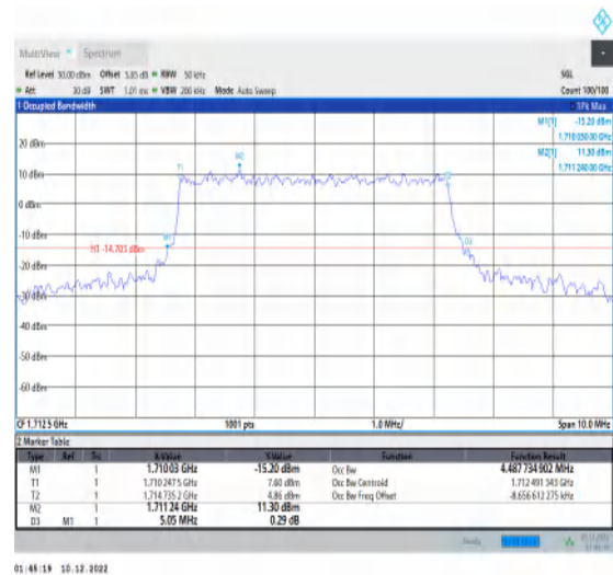
1-N66-15-5-L-4-DFT-64QAM-Outer_Full-25@0-Ant1-4 4.488-5.050-≤5-PASS
