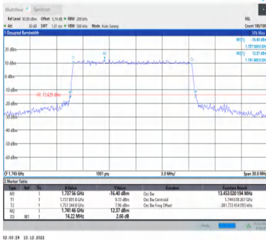
1-N66-15-15-M-4-DFT-64QAM-Outer_Full-75@0-Ant 1-13.453-14.220-≤15-PASS
