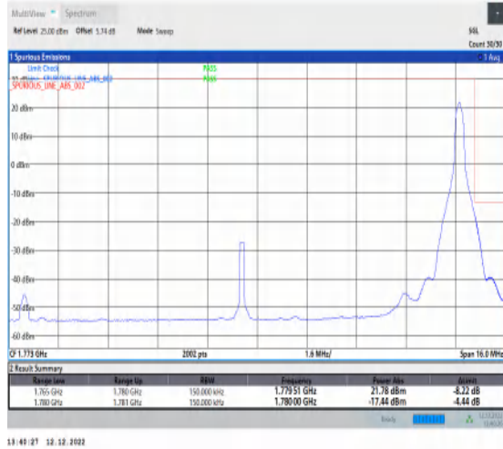
1-N66-15-15-H-2-DFT-PI2BPSK-Edge_1RB_Right-1@78-Ant1-1-seegraph-PASS-see graph
