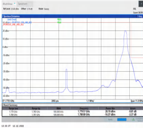
1-N66-15-10-H-2-DFT-PI2BPSK-Edge_1RB_Right-1@51-Ant1-1-seegraph-PASS-see graph
