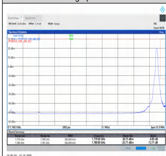
1-N66-15-30-H-5-CP-QPSK-Edge_1RB_Right-1@159-Ant1-1-seegraph-PASS-see graph
