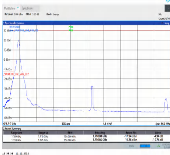
1-N66-15-15-L-4-CP-QPSK-Edge_1RB_Left-1@0-Ant1-1-seegraph-PASS-see graph
