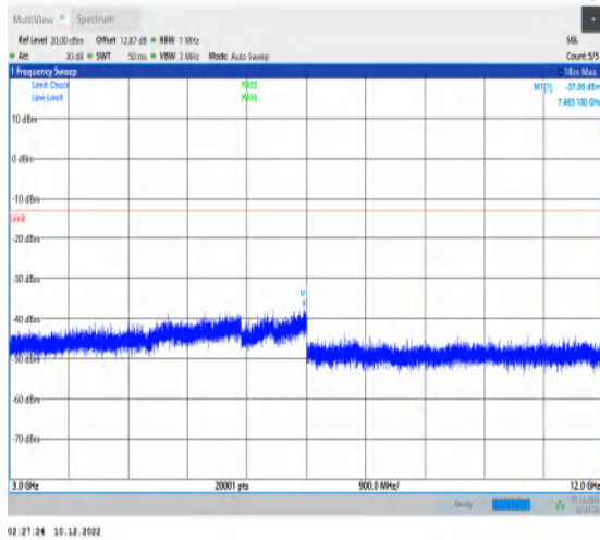
1-N66-15-40-H-1-DFT-PI2BPSK-Inner_1RB_Left-1 @1-3000-12000-Ant1-7463.10--37.00--13-PASS
