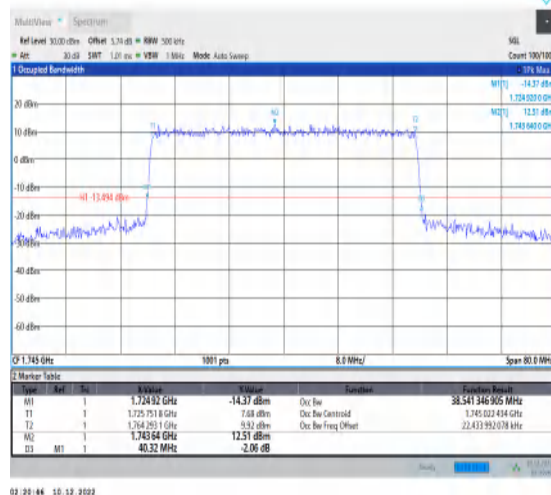
1-N66-15-40-M-4-DFT-64QAM-Outer_Full-216@0-A nt1-38.541-40.320-≤40-PASS
