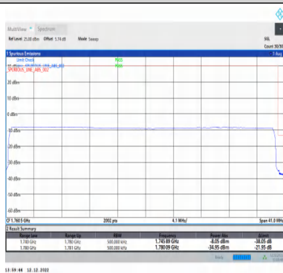
1-N66-15-40-H-6-CP-QPSK-Outer_Full-216@0-Ant1-1-seegraph-PASS-see graph
