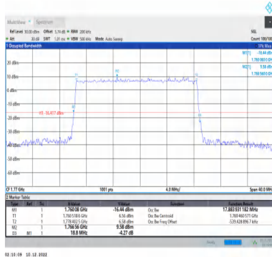
1-N66-15-20-H-5-DFT-256QAM-Outer_Full-100@0-A Ant1-17.884-18.800-≤20-PASS
