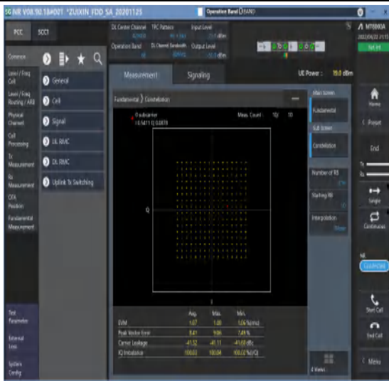
1-N66-PC3-15-40-M-5-DFT-256QAM-Outer_Full-216@0-Ant1-see graph-PASS
