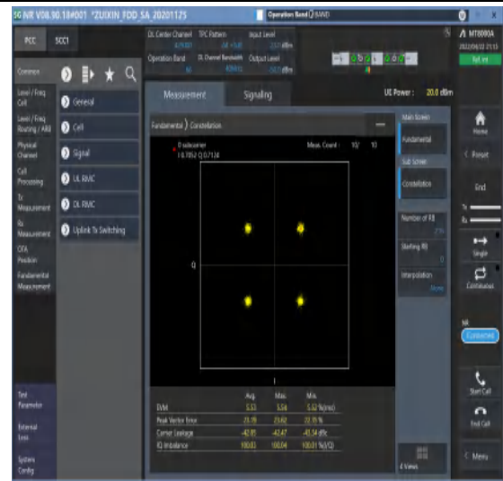
1-N66-PC3-15-40-M-6-CP-QPSK-Outer_Full-216@0-Ant1-see graph-PASS
