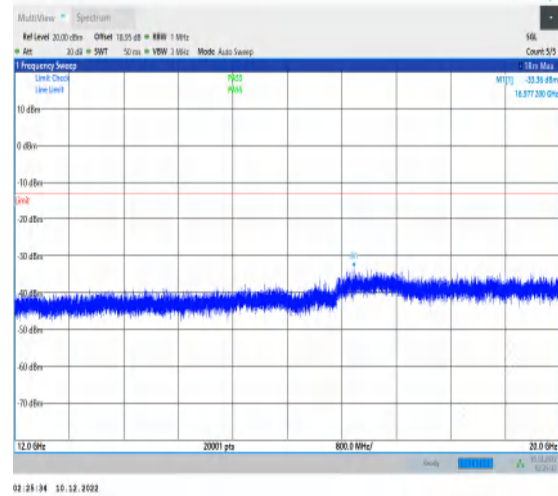
1-N66-15-40-L-1-DFT-PI2BPSK-Inner_1RB_Left-1@ 1-12000-20000-Ant1-16977.20--33.36--13-PASS
