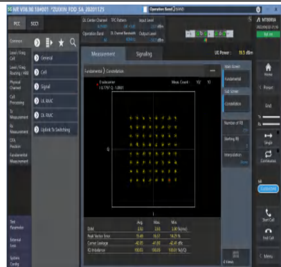
1-N66-PC3-15-40-M-8-CP-64QAM-Outer_Full-216@0-Ant1-see graph-PASS
