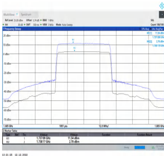
1-N66-15-40-M-1-DFT-256QAM-Outer_Full-216@0-A Ant1-8.84-100%-0.00-8.84-PASS-≤13
