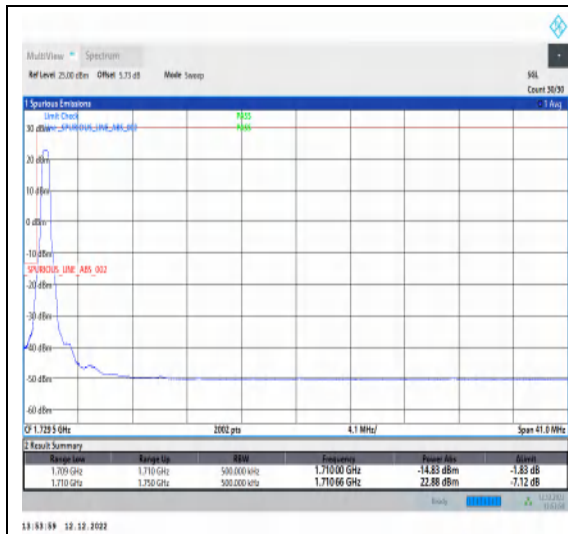
1-N66-15-40-L-1-DFT-PI2BPSK-Edge_1RB_Left-1@0-Ant1-1-seegraph-PASS-see graph
