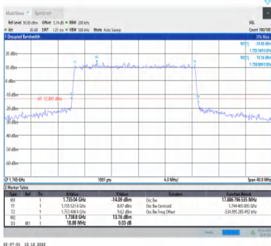
1-N66-15-20-M-1-DFT-QPSK-Outer_Full-100@0-Ant 1-17.887-18.880-≤20-PASS
