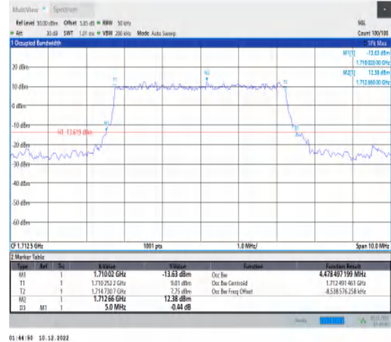
1-N66-15-5-L-2-DFT-PI2BPSK-Outer_Full-25@0-Ant1-4 1-4.478-5.000-≤5-PASS
