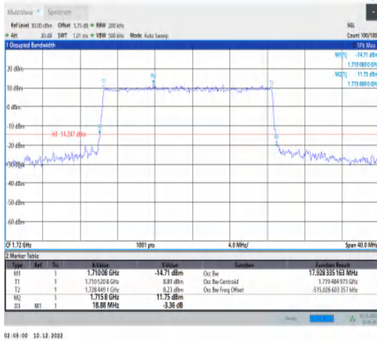
1-N66-15-20-L-4-DFT-64QAM-Outer_Full-100@0-An t1-17.928-18.880-≤20-PASS
