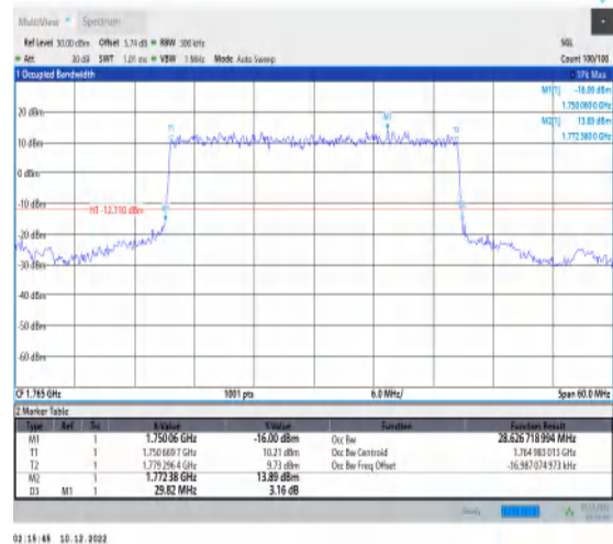
1-N66-15-30-H-2-DFT-PI2BPSK-Outer_Full-160@0-Ant 1-28.627-29.820-≤30-PASS
