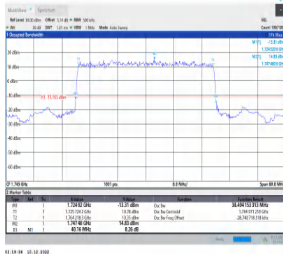
1-N66-15-40-M-2-DFT-PI2BPSK-Outer_Full-216@0-Ant 1-38.494-40.160-≤40-PASS
