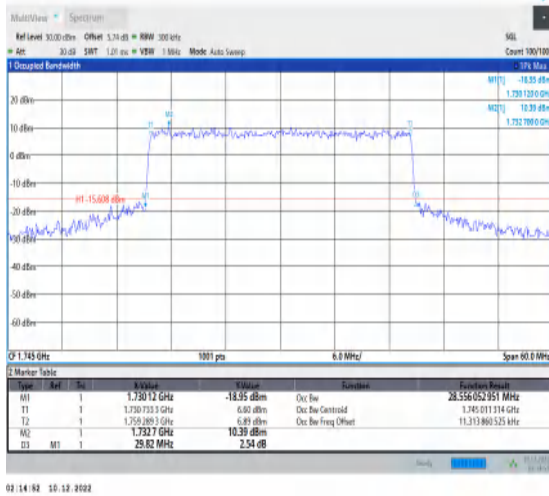
1-N66-15-30-M-8-CP-64QAM-Outer_Full-160@0-Ant 1-28.556-29.820-≤30-PASS
