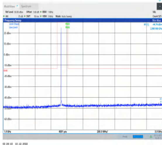
1-N66-15-40-M-1-DFT-PI2BPSK-Inner_1RB_Left-1@ 1-1000-3000-Ant1-2980.00--44.74--13-PASS
