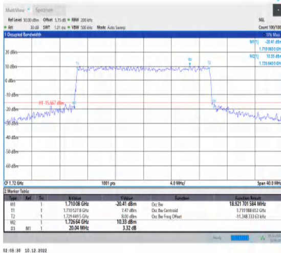
1-N66-15-20-L-6-CP-QPSK-Outer_Full-106@0-Ant1- 18.922-20.040-≤20-PASS
