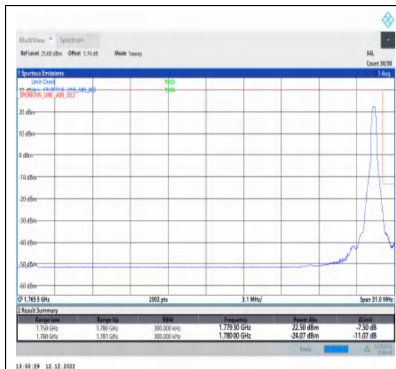
1-N66-15-30-H-2-DFT-PI2BPSK-Edge_1RB_Right-1@159-Ant1-1-seegraph-PASS-see graph
