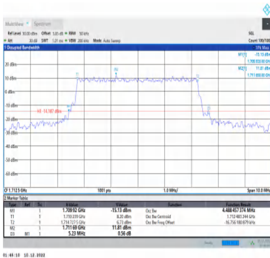
1-N66-15-5-L-3-DFT-16QAM-Outer_Full-25@0-Ant1-4 4.488-5.230-≤5-PASS
