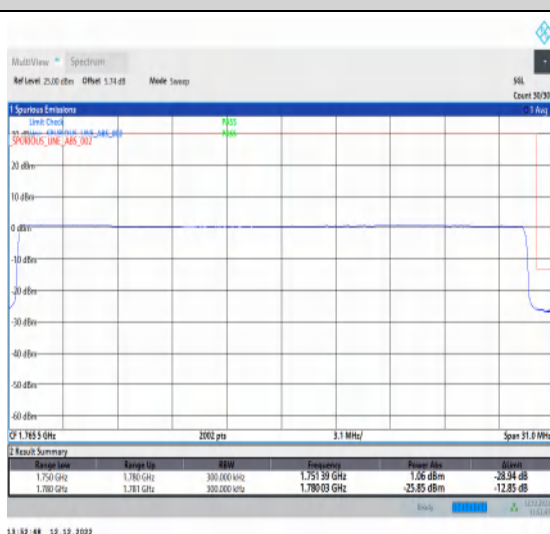
1-N66-15-30-H-6-CP-QPSK-Outer_Full-160@0-Ant1-1-seegraph-PASS-see graph
