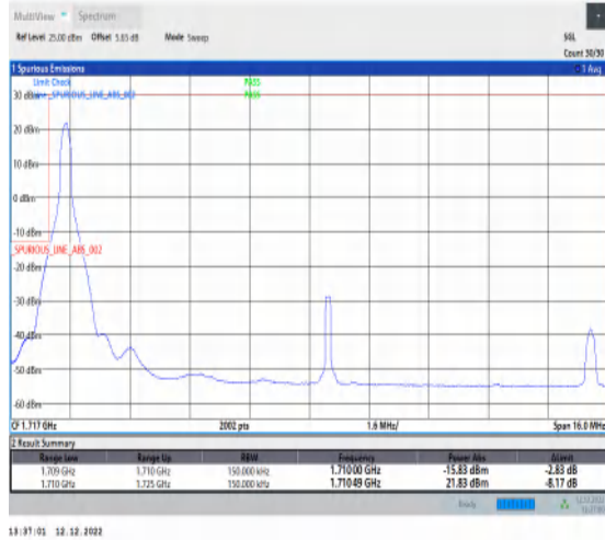
1-N66-15-15-L-1-DFT-PI2BPSK-Edge_1RB_Left-1@0-Ant1-1-seegraph-PASS-see graph
