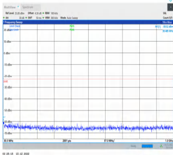
1-N66-15-40-L-1-DFT-PI2BPSK-Inner_1RB_Left-1 @1-30-1000-Ant1-30.49--59.52--23-PASS
