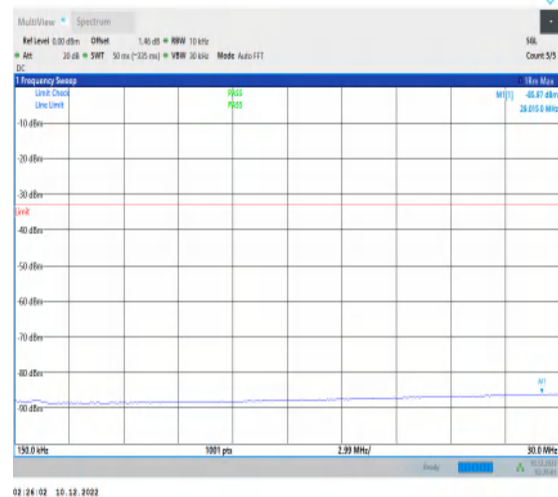
1-N66-15-40-M-1-DFT-PI2BPSK-Inner_1RB_Left-1@ 1-0.15-30-Ant1-29.01--85.97--33-PASS
