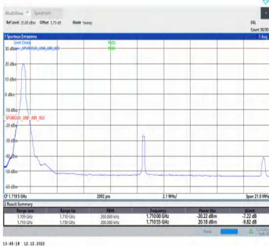
1-N66-15-20-L-4-CP-QPSK-Edge_1RB_Left-1@0-Ant1-1-seegraph-PASS-see graph
