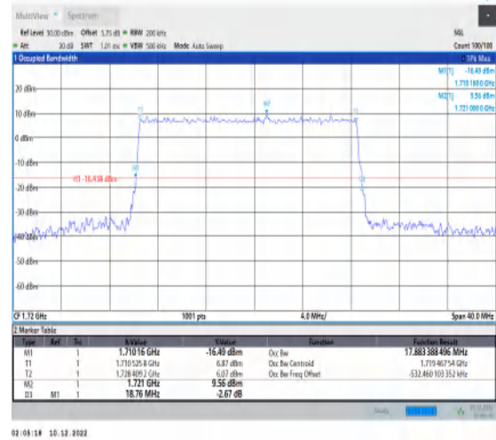
1-N66-15-20-L-5-DFT-256QAM-Outer_Full-100@0-A nt1-17.883-18.760-≤20-PASS
