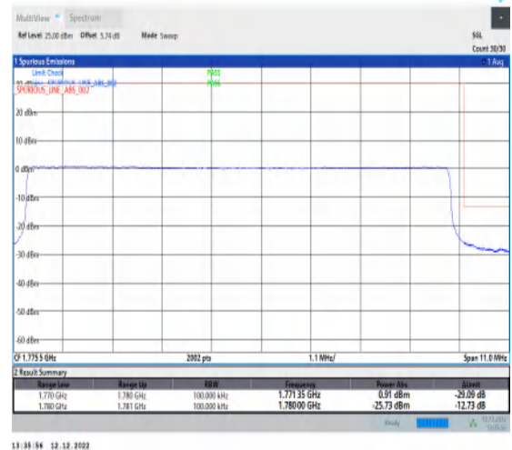
1-N66-15-10-H-6-CP-QPSK-Outer_Full-52@0-Ant1-1-seegraph-PASS-see graph
