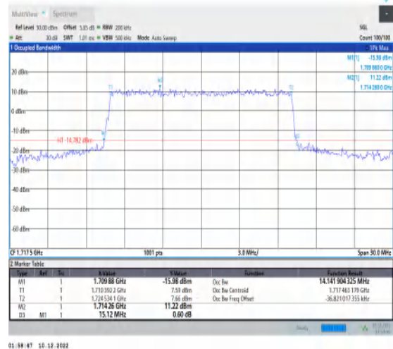
1-N66-15-15-L-6-CP-QPSK-Outer_Full-79@0-Ant1-1 t1-14.142-15.120≤15-PASS
