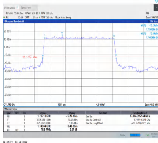
1-N66-15-20-M-2-DFT-PI2BPSK-Outer_Full-100@0-Ant 1-17.866-18.800-≤20-PASS
