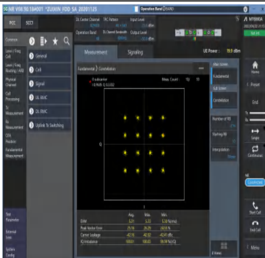
1-N66-PC3-15-40-M-7-CP-16QAM-Outer_Full-216@0-Ant1-see graph-PASS
