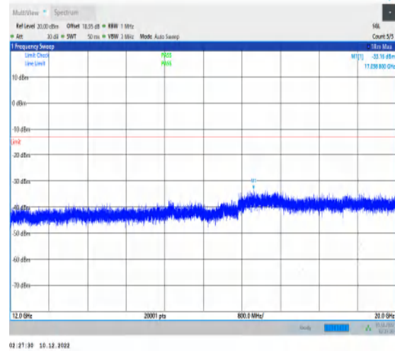
1-N66-15-40-H-1-DFT-PI2BPSK-Inner_1RB_Left-1@ 1-12000-20000-Ant1-17038.80--33.16--13-PASS
