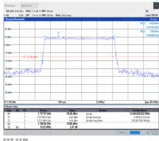
1-N66-15-15-M-5-DFT-256QAM-Outer_Full-75@0-A nt1-13.455-14.250-≤15-PASS
