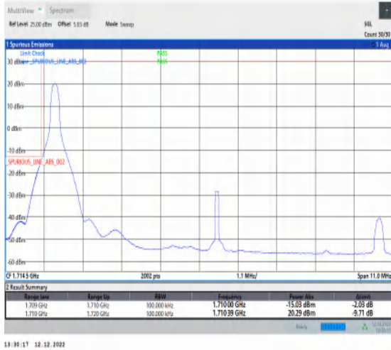
1-N66-15-10-L-1-DFT-PI2BPSK-Edge_1RB_Left-1@0-Ant1-1-seegraph-PASS-see graph
