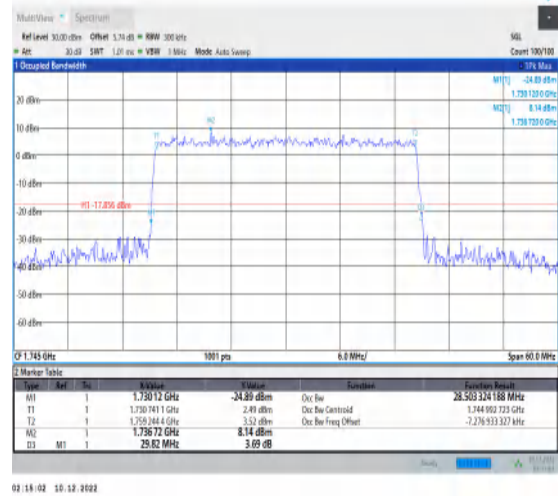
1-N66-15-30-M-9-CP-256QAM-Outer_Full-160@0-A nt1-28.503-29.820-≤30-PASS
