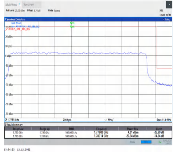
1-N66-15-10-H-3-DFT-PI2BPSK-Outer_Full-50@0-Ant1-1-seegraph-PASS-see graph
