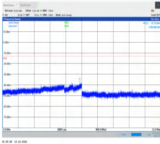
1-N66-15-40-L-1-DFT-PI2BPSK-Inner_1RB_Left-1 @ 1-3000-12000-Ant1-7392.00--37.73--13-PASS
