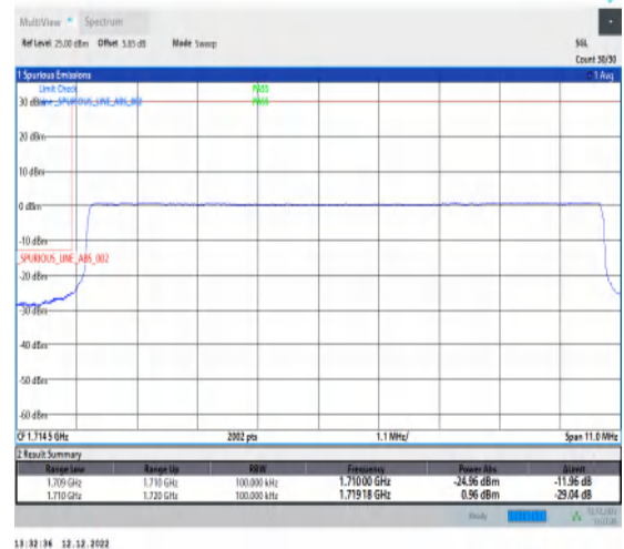
1-N66-15-10-L-6-CP-QPSK-Outer_Full-52@0-Ant1-1-seegraph-PASS-see graph
