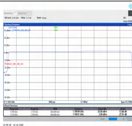
1-N66-15-40-L-6-CP-QPSK-Outer_Full-216@0-Ant1-1-seegraph-PASS-see graph
