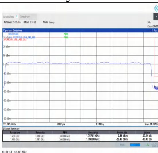
1-N66-15-30-H-3-DFT-PI2BPSK-Outer_Full-160@0-Ant1-1-seegraph-PASS-see graph
