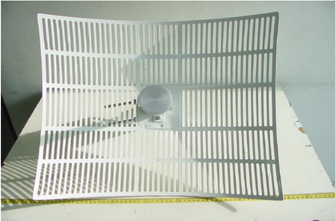
Front View of Antenna 1
