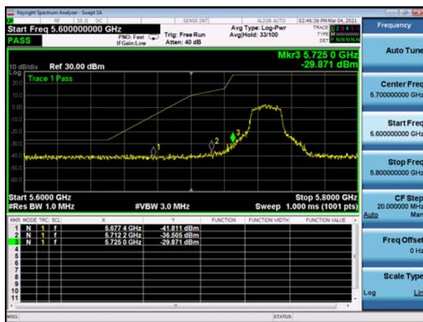
U-NII-3 ,Plot 1,Band Edge-802.11a(20M Hz),5745MHz
