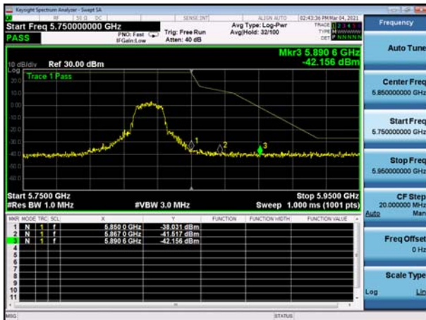
U-NII-3 ,Plot 1,Band Edge-802.11a(20 Hz),5825MHz
