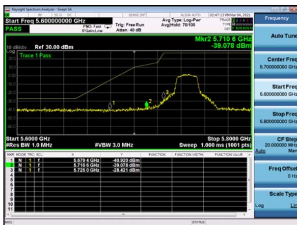
U-NII-3 ,Plot 1,Band Edge-802.11n(20M Hz),5745MHz
