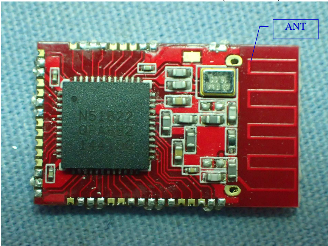
Figure 7 Internal View (BLE Module, Front View)
