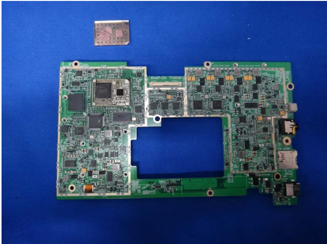
(38) EUT Photo
