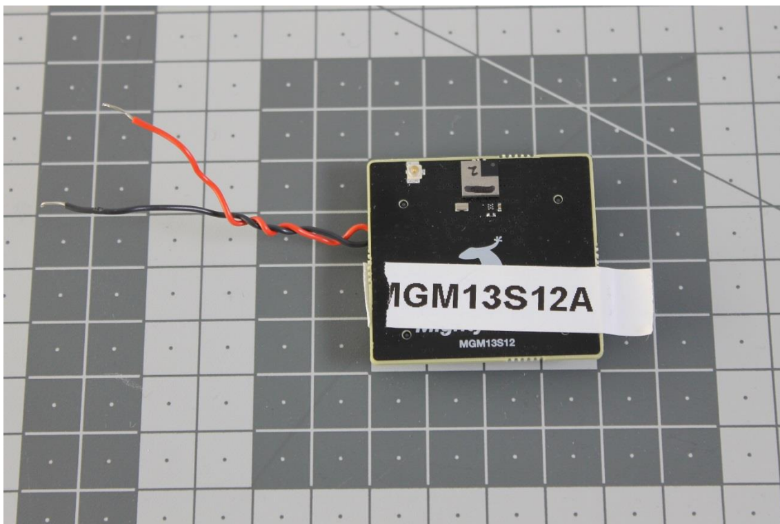
Photograph 4. EUT 2, MGM13S12E
