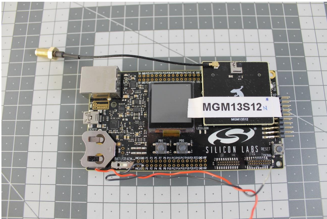
Photograph 1. EUT 1 MGM13S12N
