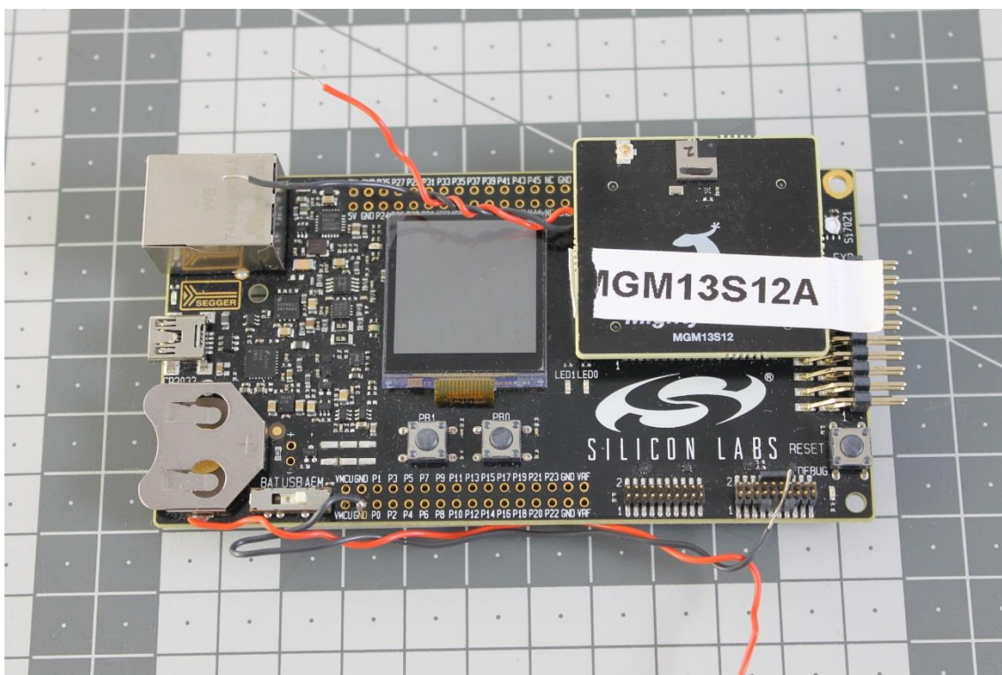
Photograph 3. EUT 2, MGM13S12A
