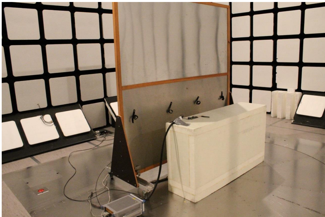
Photograph 10. Conducted Emissions
