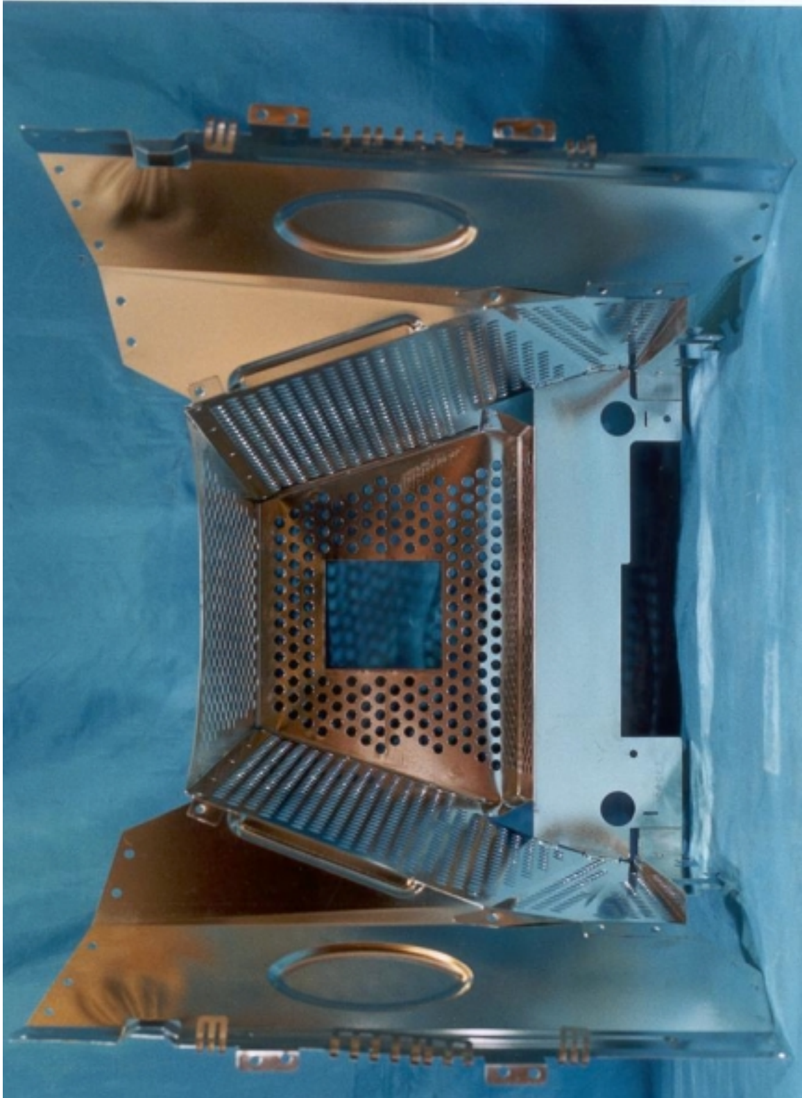
Metal Cover
