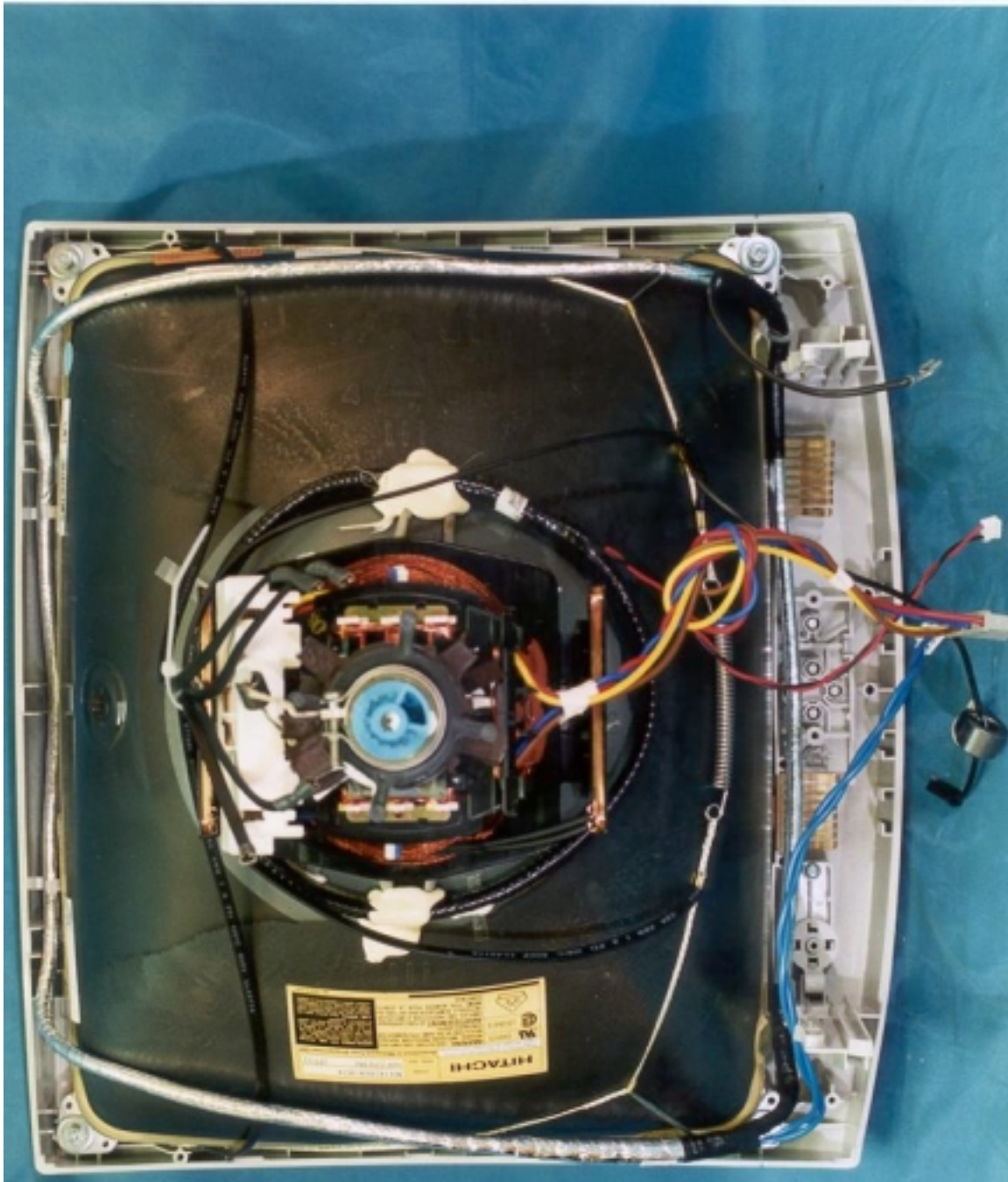
CRT Assembly
