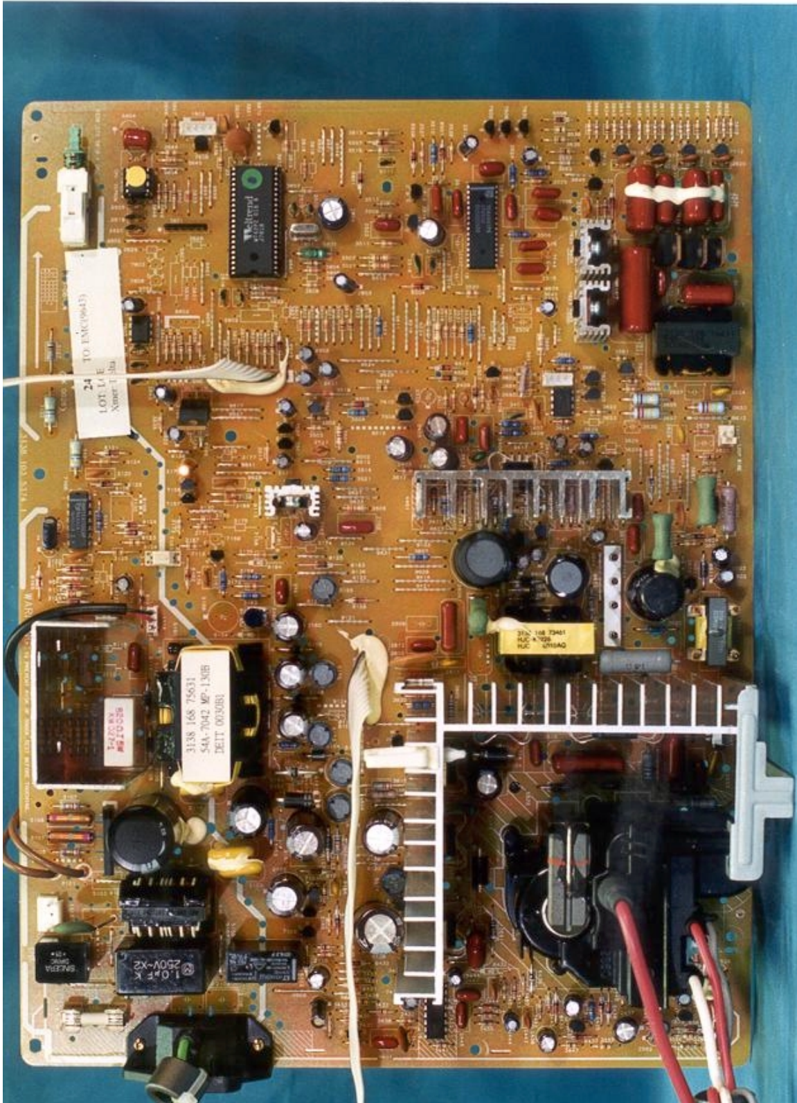
PCB Layout
