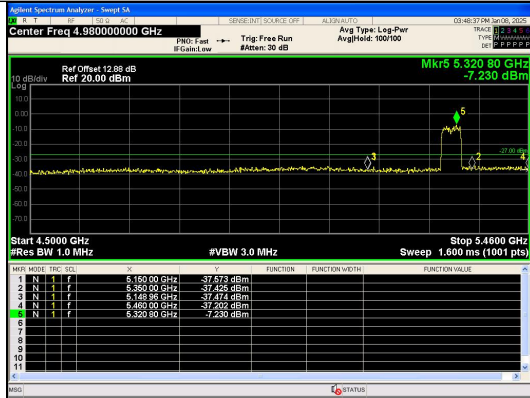
Out Of Band Emission IEEE 802.11n_Channel 62_40MHz_Antenna 0
