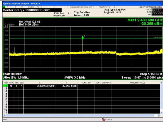
Spurious Emission:30.0~5150 MHz IEEE 802.11n_Channel 54_40MHz_Antenna 0
