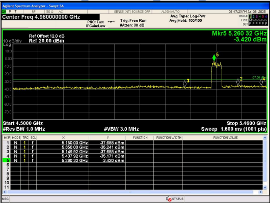
Out Of Band Emission IEEE 802.11n_Channel 54_40MHz_Antenna 0
