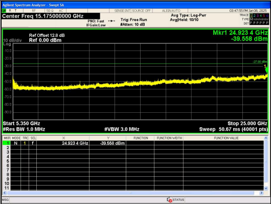
Spurious Emission:5350~25000.0 MHz IEEE 802.11n_Channel 54_40MHz_Antenna 0
