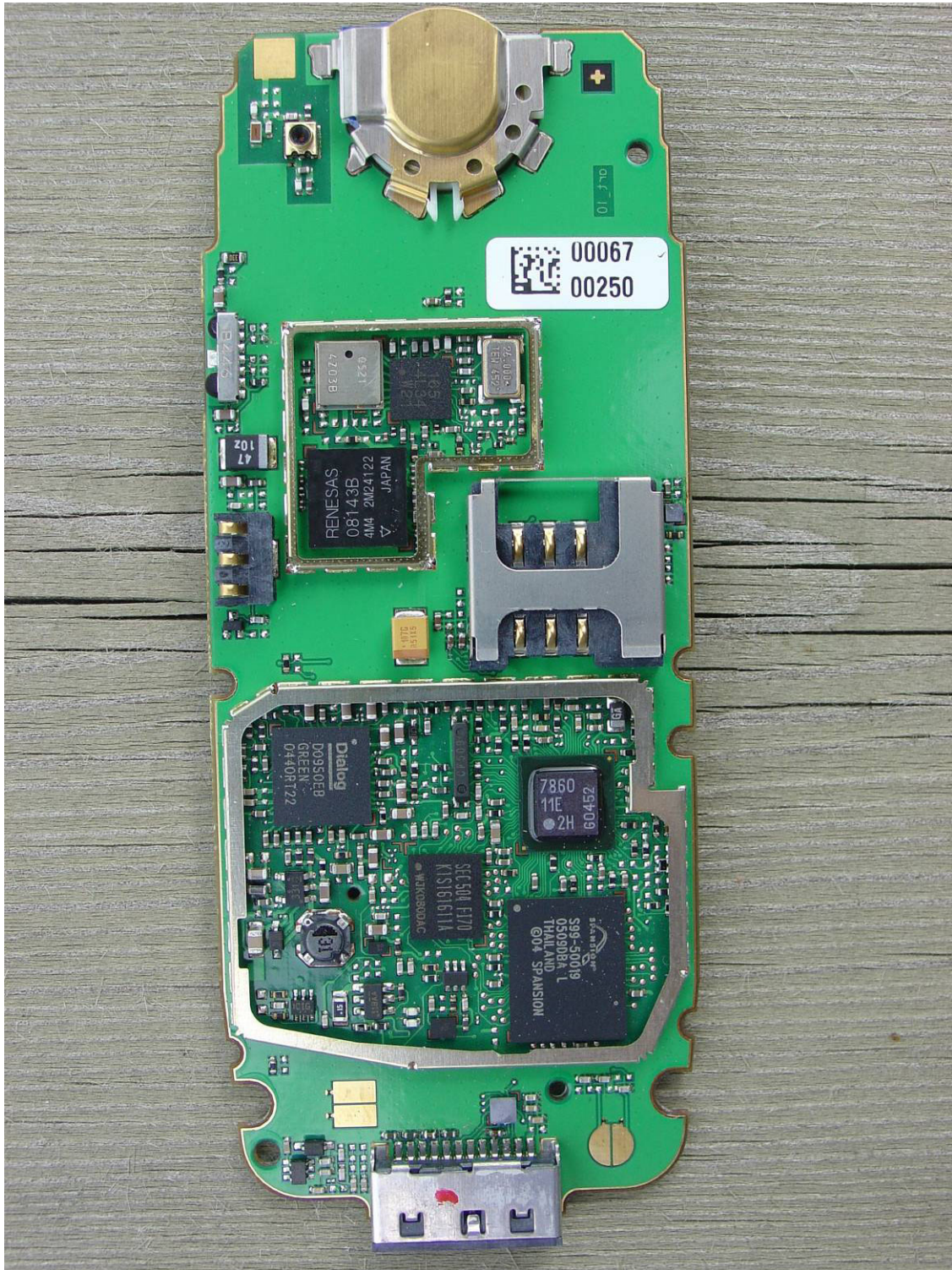
AX75 Back view shields removed
