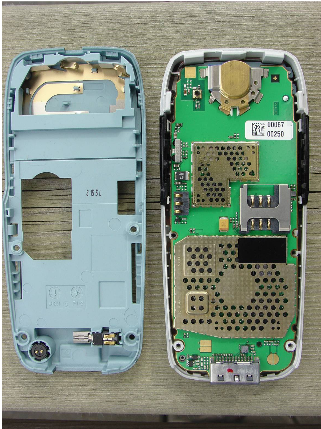
AX75 Disassembly Step 1
