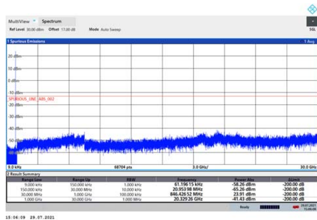
LTE-M Band 5 3MHz CH-High 9kHz~30GHz
