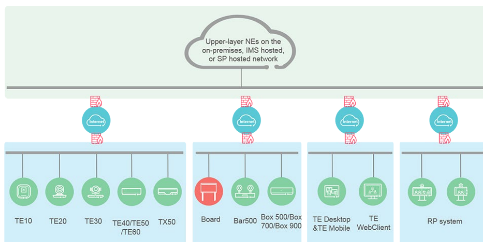
Figure 3-1 Networking scheme
