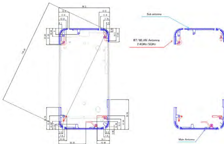
Fig.16 Antenna position of EUT
