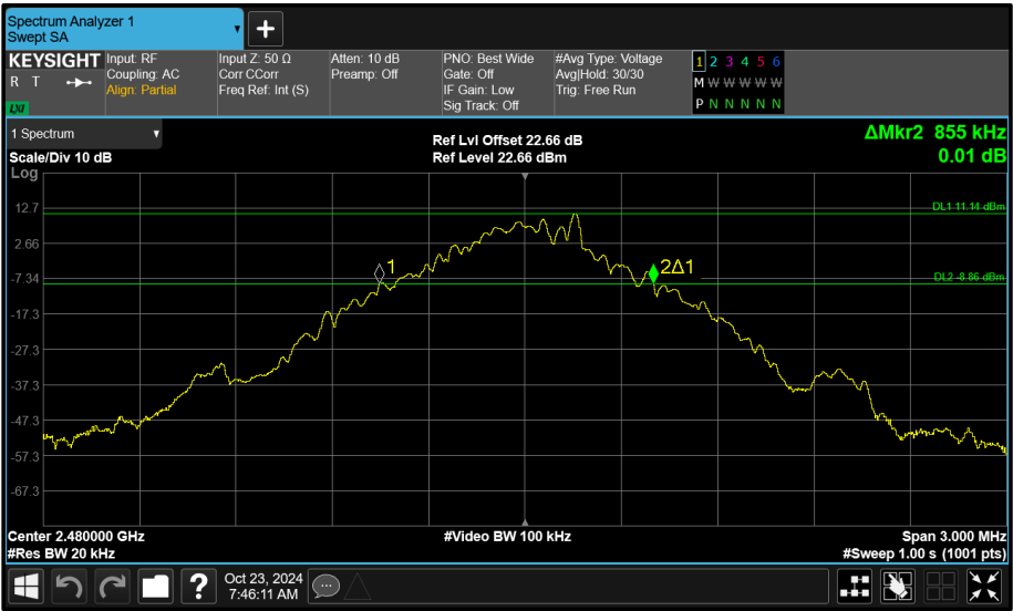
Figure 78 - Core 1 (B) 2480 MHz (CH78) 20 dB Bandwidth
