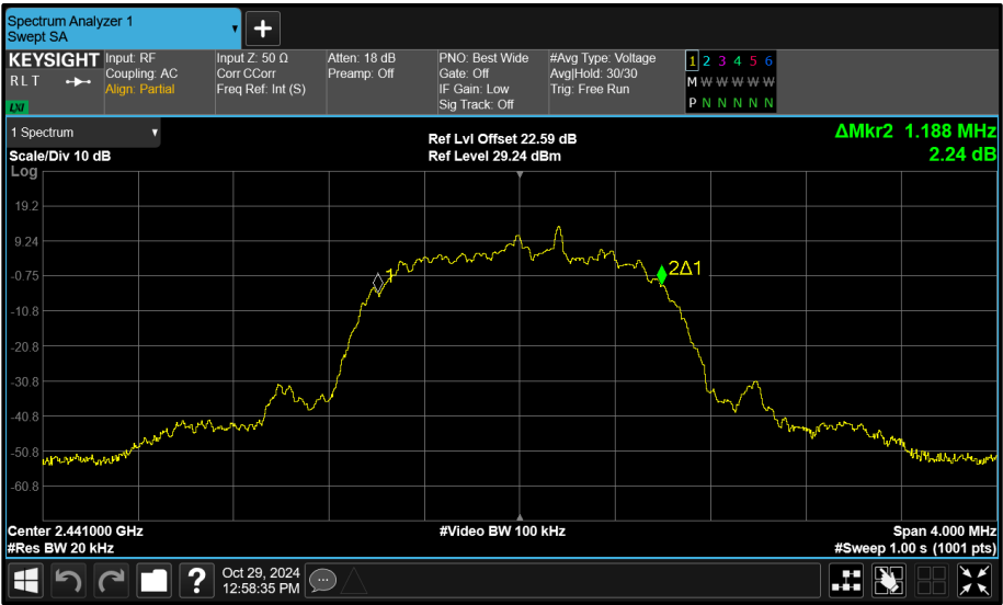
Figure 122 - Core 1 (B) 2441 MHz (CH39) 99% Bandwidth
