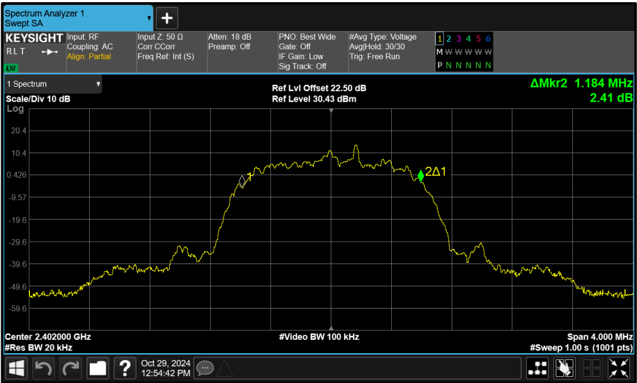
Figure 121 - Core 1 (B) 2402 MHz (CH0) 99% Bandwidth
