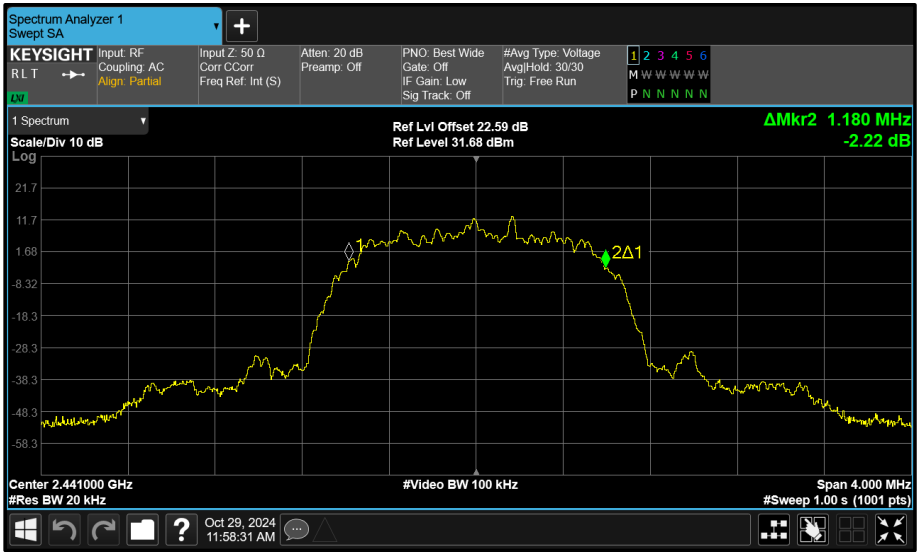
Figure 116 - Core 1 (B) 2441 MHz (CH39) 99% Bandwidth
