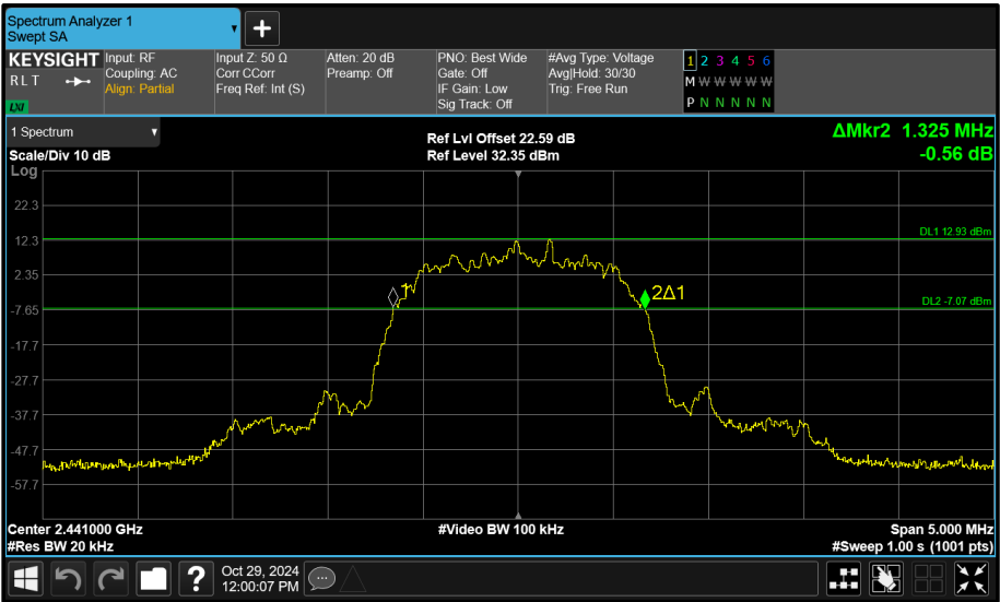
Figure 113 - Core 1 (B) 2441 MHz (CH39) 20 dB Bandwidth
