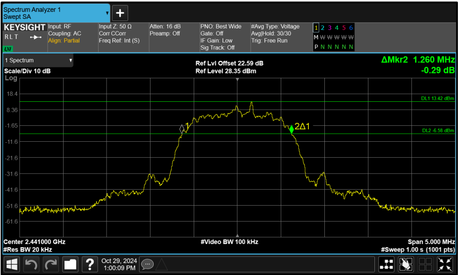
Figure 119 - Core 1 (B) 2441 MHz (CH39) 20 dB Bandwidth
