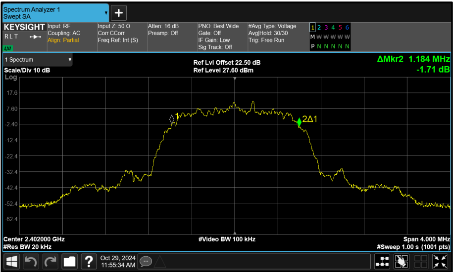
Figure 115 - Core 1 (B) 2402 MHz (CH0) 99% Bandwidth
