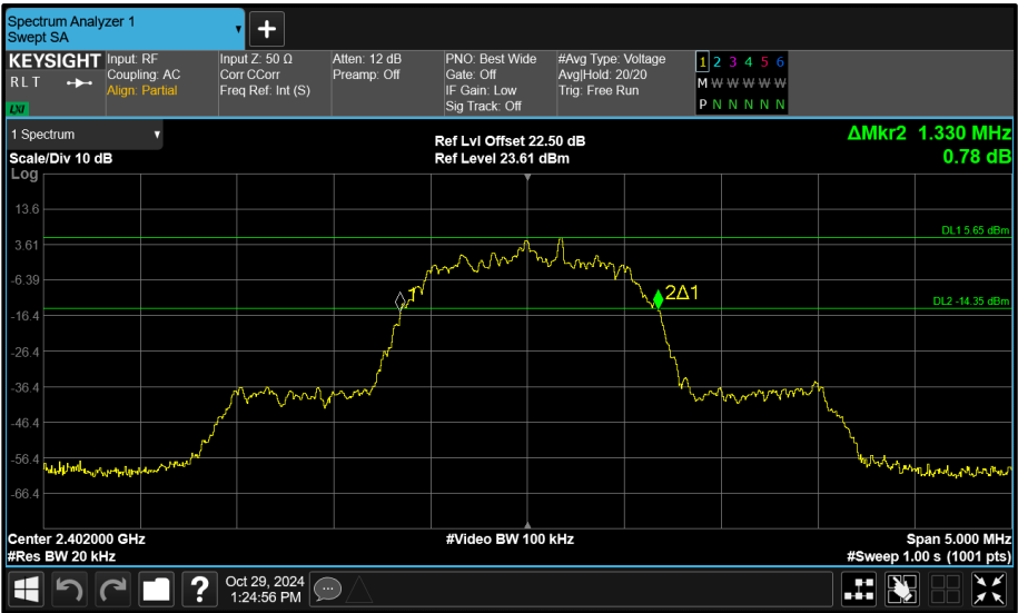
Figure 137 - Core 1 (B) 2402 MHz (CH0) 20 dB Bandwidth
