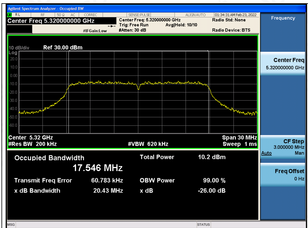
Test_Graph_802.11ac20_ANT2_5320_MCS9_OBW
