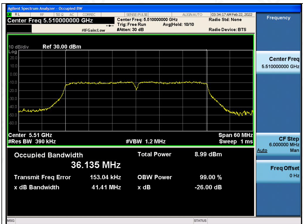
Test_Graph_802.11ac40_ANT1_5510_MCS9_OBW
