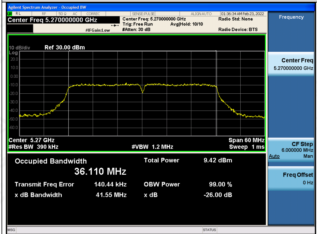
Test_Graph_802.11ac40_ANT2_5270_MCS9_OBW
