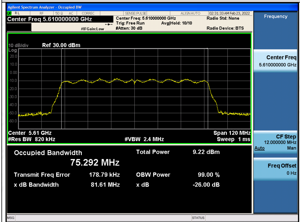
Test_Graph_802.11ac80_ANT2_5610_MCS9_OBW
