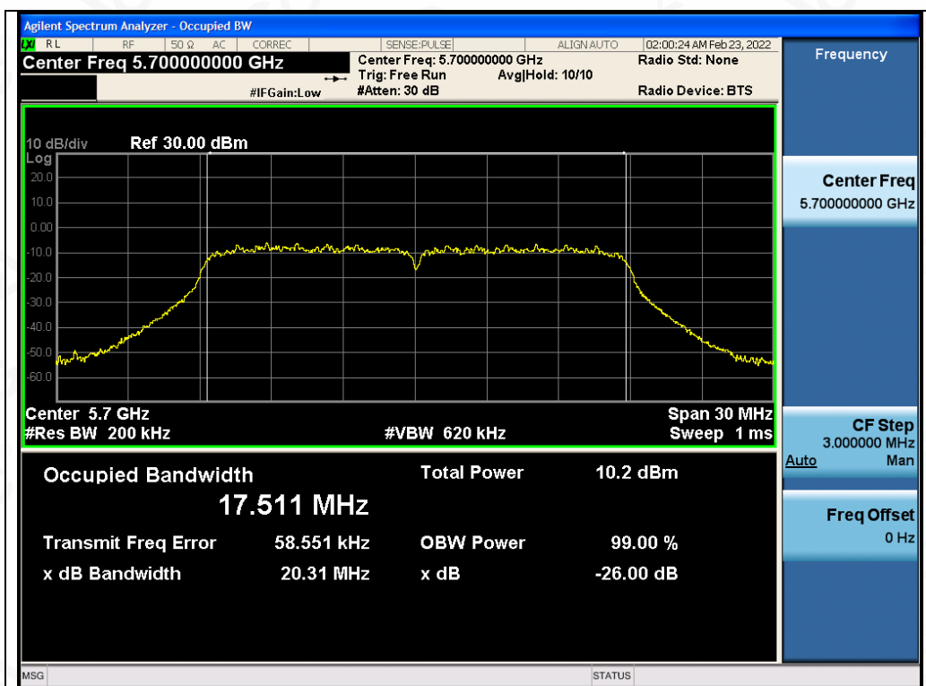
Test_Graph_802.11n20_ANT2_5700_MCS0_OBW
