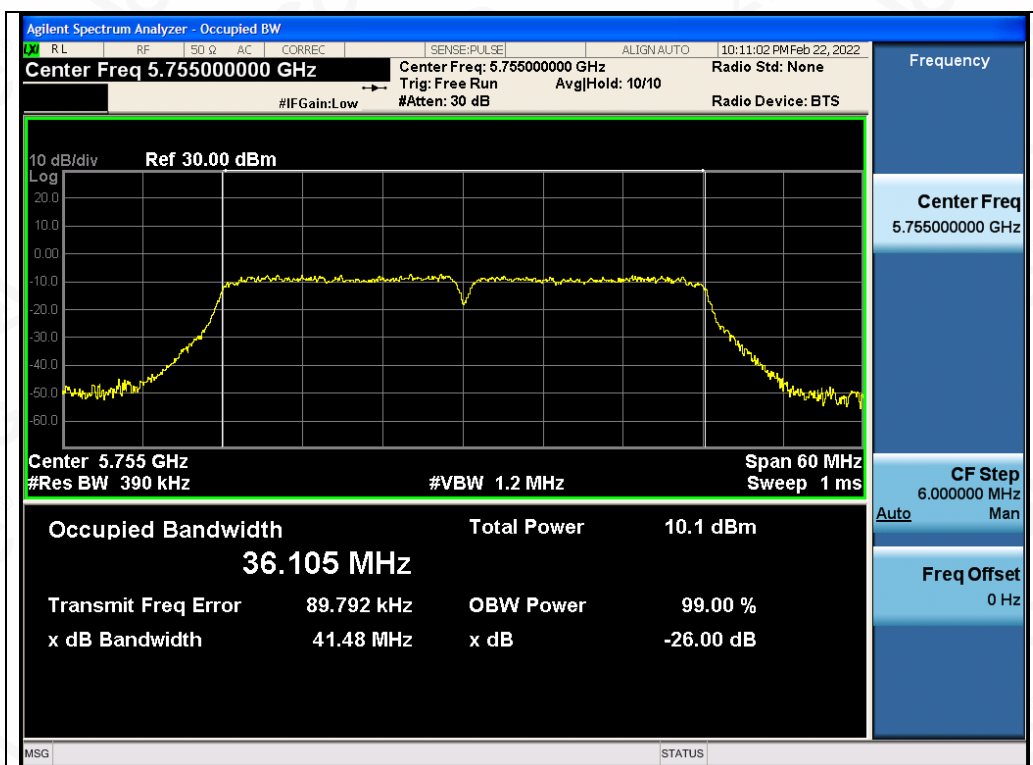
Test_Graph_802.11n40_ANT2_5755_MCS0_OBW
