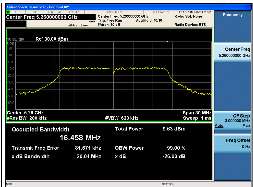
Test_Graph_802.11a_ANT2_5260_6Mbps_OBW
