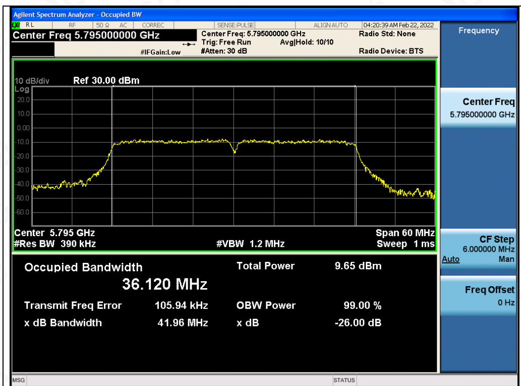
Test_Graph_802.11ac40_ANT1_5795_MCS9_OBW
