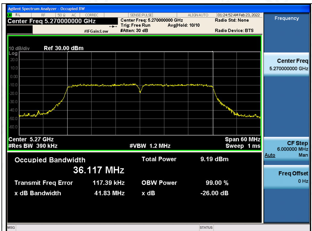
Test_Graph_802.11n40_ANT2_5270_MCS0_OBW
