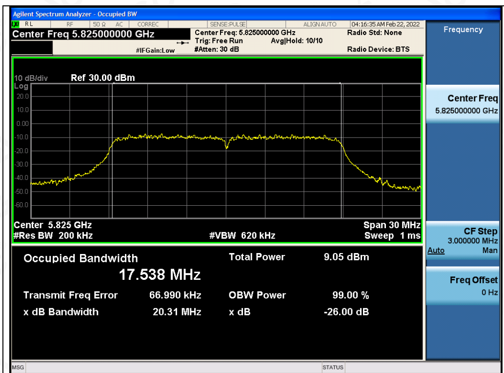
Test_Graph_802.11ac20_ANT1_5825_MCS9_OBW
