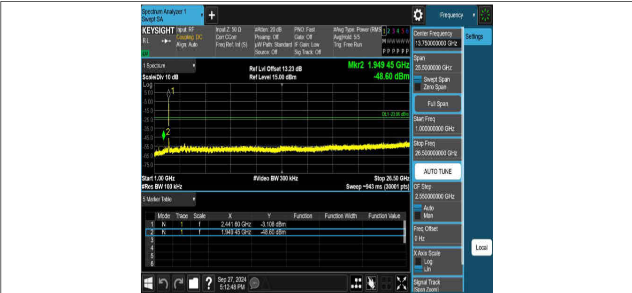
11AX40SISO_Ant1_2452_0~Reference
