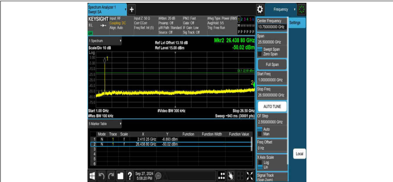
11AX40SISO_Ant1_2437_0~Reference
