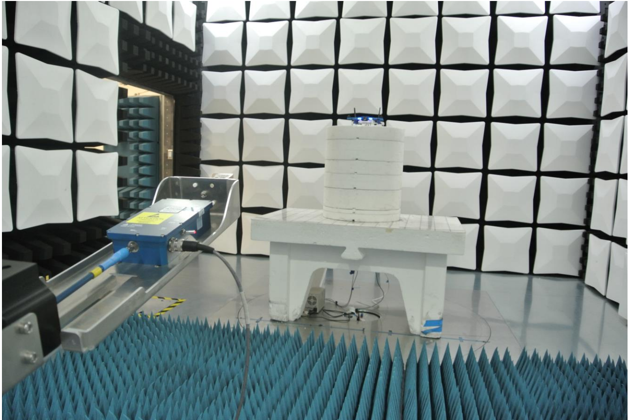
Figure 5: Test Setup for Radiated Emissions 18GHz to 40 GHz
