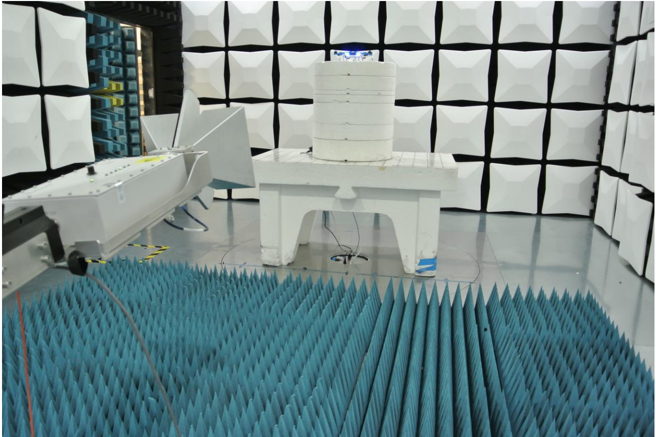
Figure 4: Test Setup for Radiated Emissions 1GHz to 18GHz
